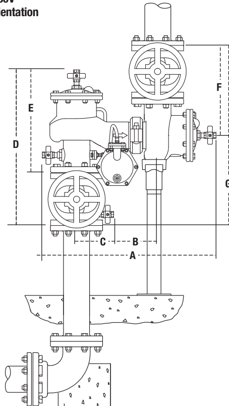
Relief Valve Detail Relief shipped on right side (shown) field reversible to left side.
