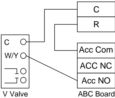
Figure 7b: Open Loop Solenoid Valve Connection Option Typical slow operating external 24V water solenoid valve (type V100FPT) wiring.
