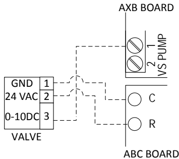
Figure 7c: Modulating Water Valve Connection Option Typical 0-10VDC modulating water valve.
