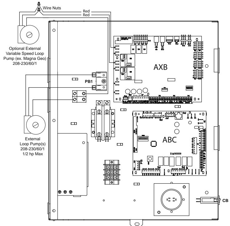
Figure 11: Pump Wiring 208-230/60/1
