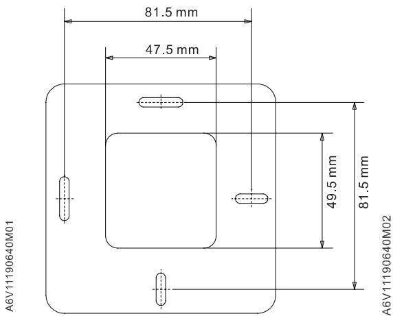
Metallic mounting plate
