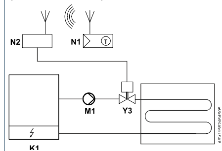
Floor heating with pump (with RCR114.1)
