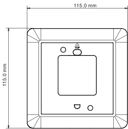
White decorative frame
