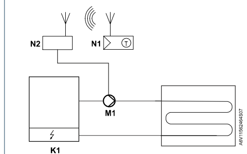
Electric floor heating (with RCR114.1)
