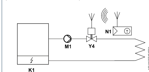
Radiator with valve (with SSA911.01.TH)
