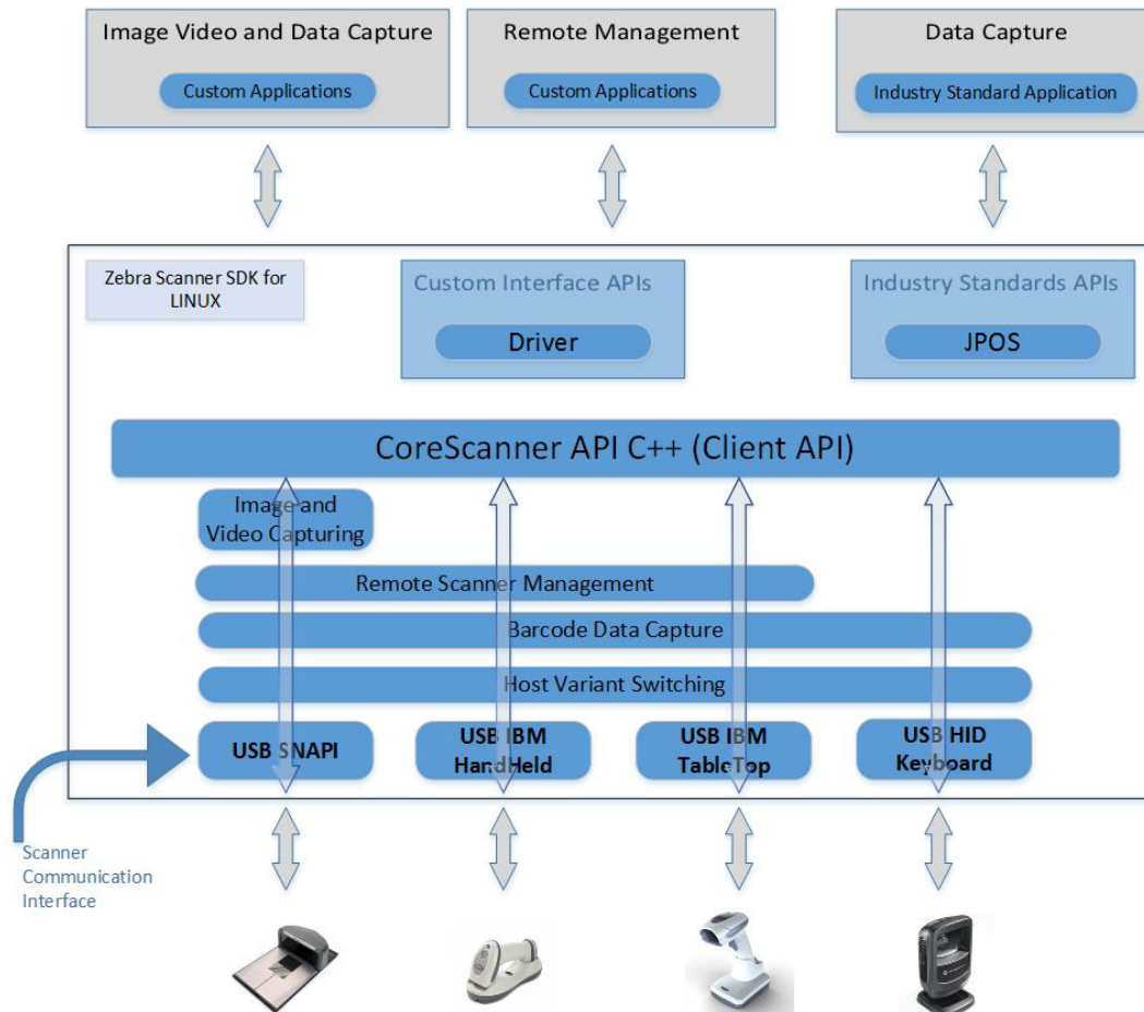
Figure 1-2 SDK Architecture
