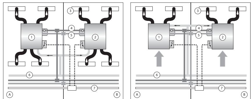
Figure 1 - Typical installations
