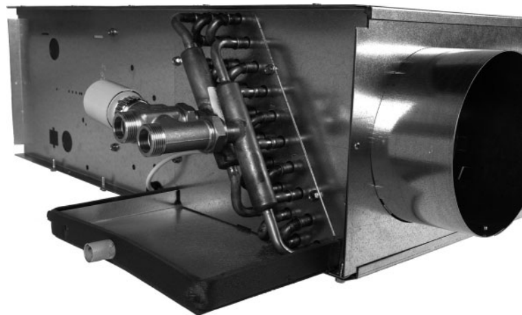
Figure 12 - Valve package
