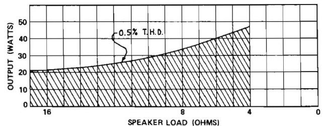
The impedance of all loudspeakers varies with frequency. The SA 30 - 30 has extra reserve power for any load with lowest distortion.
