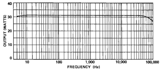
Frequency Response (32 watts @ 8 Ω)
