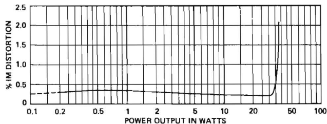
Intermodulation Distortion (1 chan, 8 Ω) 60 Hz and 7000 Hz (mixed 4:1) Low intermodulation distortion at all power output levels below clipping ensures complete tonal clarity, and separation of complex sounds.
