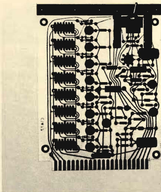
Integrated circuit logic module.
