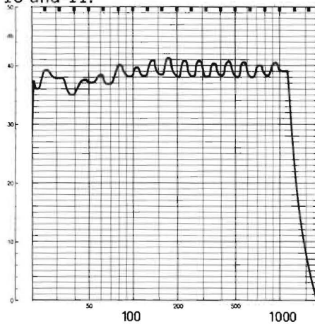
Figure 10. Pass band obtained when all attenuators above 1 kHz are set to maximum attenuation.
