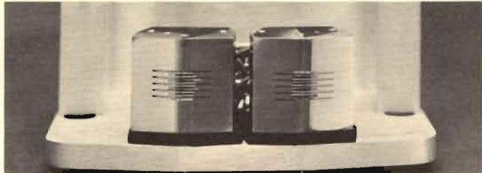
Model 1220 Focused Gap record head assembly, 8-T, ¼ in.
