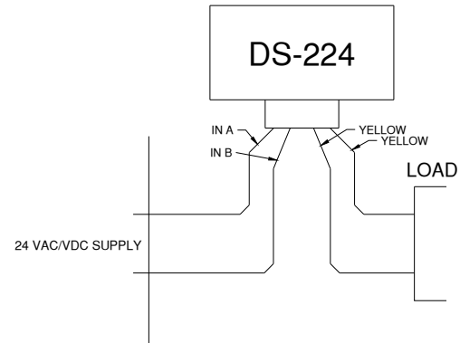
24VAC/VDC Sensor Supply, Dry Contact Thermostat-Style Control
