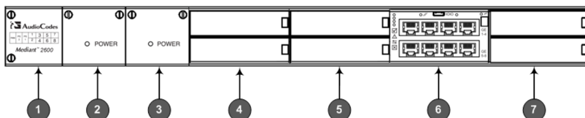
Figure 3-1: Front Panel
