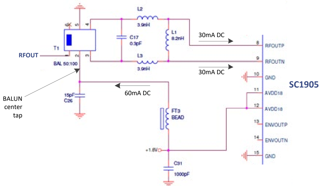
Figure 8. RFOUT BALUN, matching network and decoupling.
