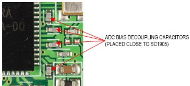
Figure 11. ADC decoupling capacitors.
