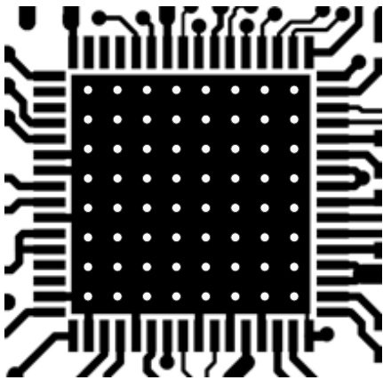
Figure 14. Via array under SC1905 ground paddle.
