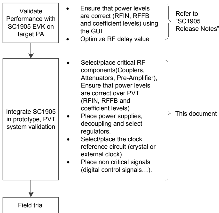
Figure 1. SC1905 integration flow.
