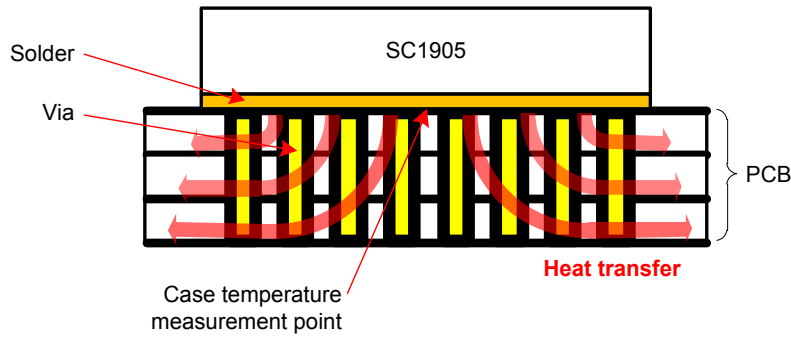
Figure 17. PCB fabrication layer stack.
