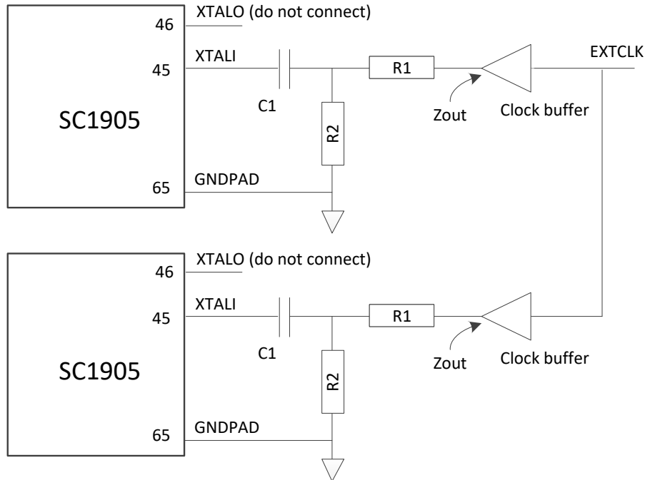
Figure 25. External clock diagram for multiple SC1905 applications.
