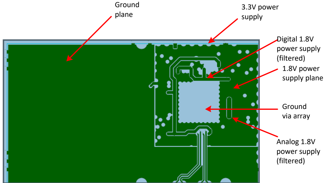
Figure 16. Layer 3, power supply distribution.
