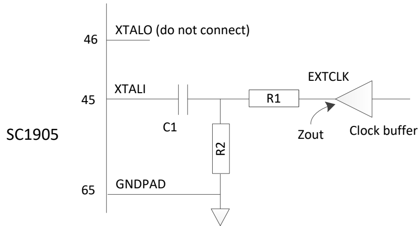
Figure 21. External clock diagram.
