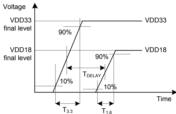
Figure 18. VDD18 and VDD33 power-on timing sequence.
