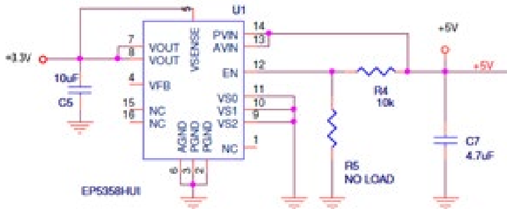
Figure 19. 5V to 3.3V switching regulator.
