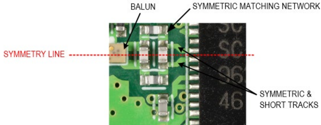
Figure 6. Balun + differential matching network.
