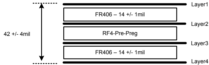
Figure 13. PCB fabrication layer stack.
