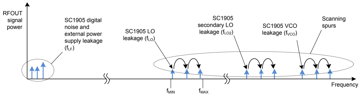
Figure 10. SC1905 spurious content (CAL mode).
