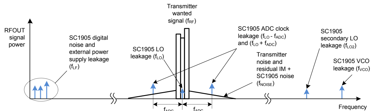
Figure 9. SC1905 spurious content (TRACK/FSA mode).
