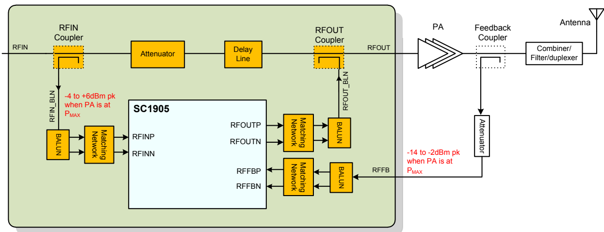
Figure 5. System block diagram.
