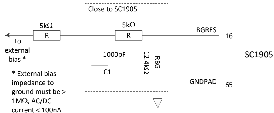
Figure 22. External bias circuit using the SC1905 bandgap voltage.
