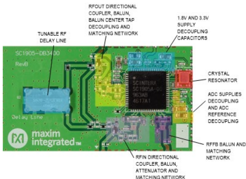
Figure 12. SC1905 reference board floor plan.
