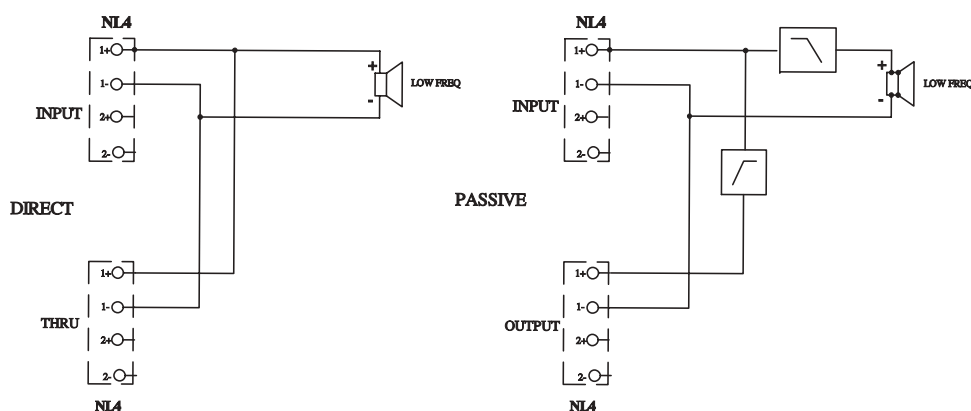
REV01 SUB 118P BLOCK DIAGRAM
