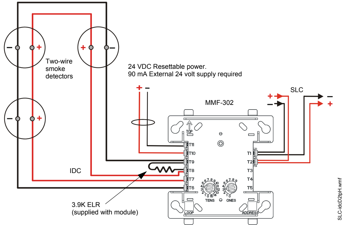
Figure 5.16 Typical Style D IDC Wiring with an MMF-302
