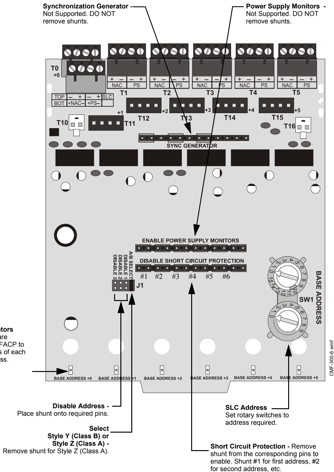
Figure 6.4 CMF-300-6 Control Module Settings
