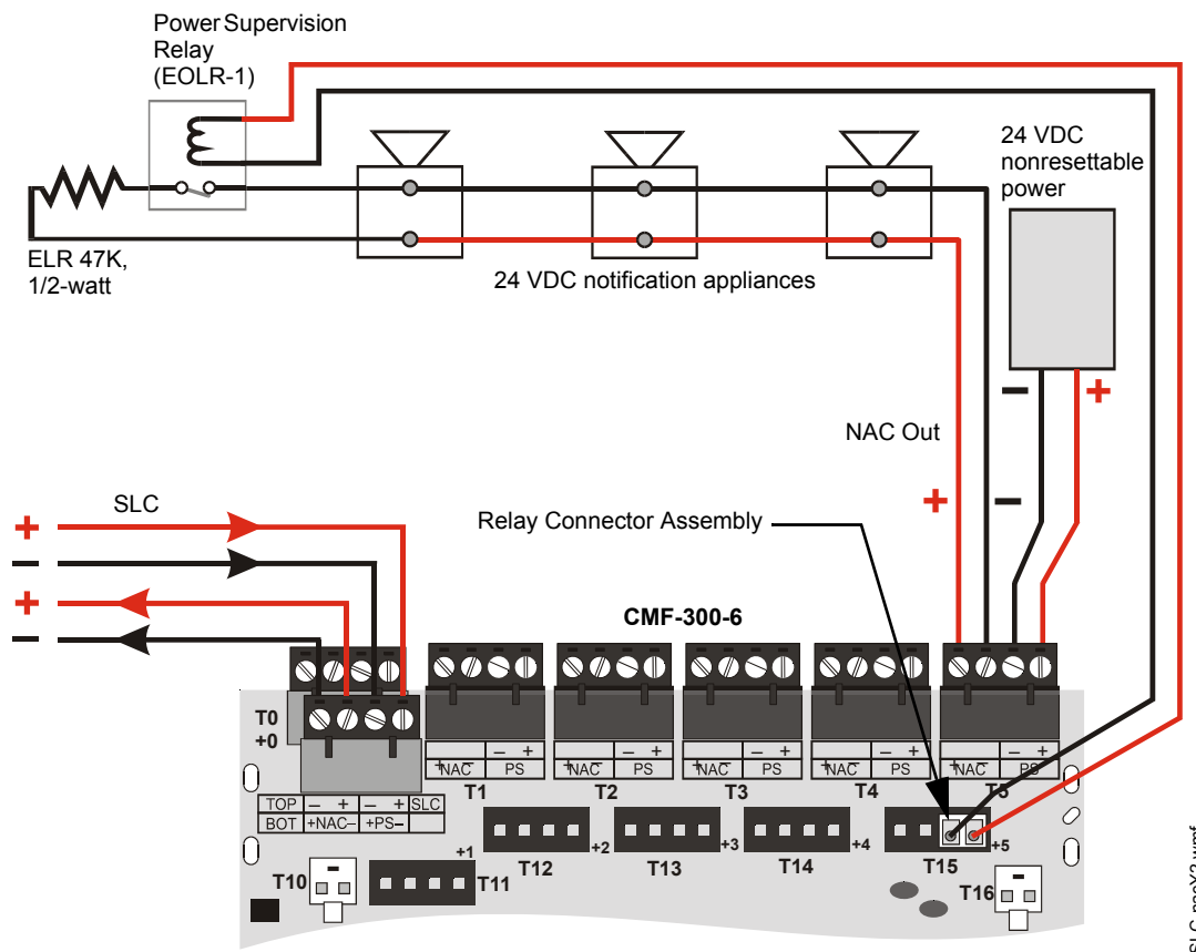
Figure 6.5 NFA Style Y Notification Appliance Circuit
