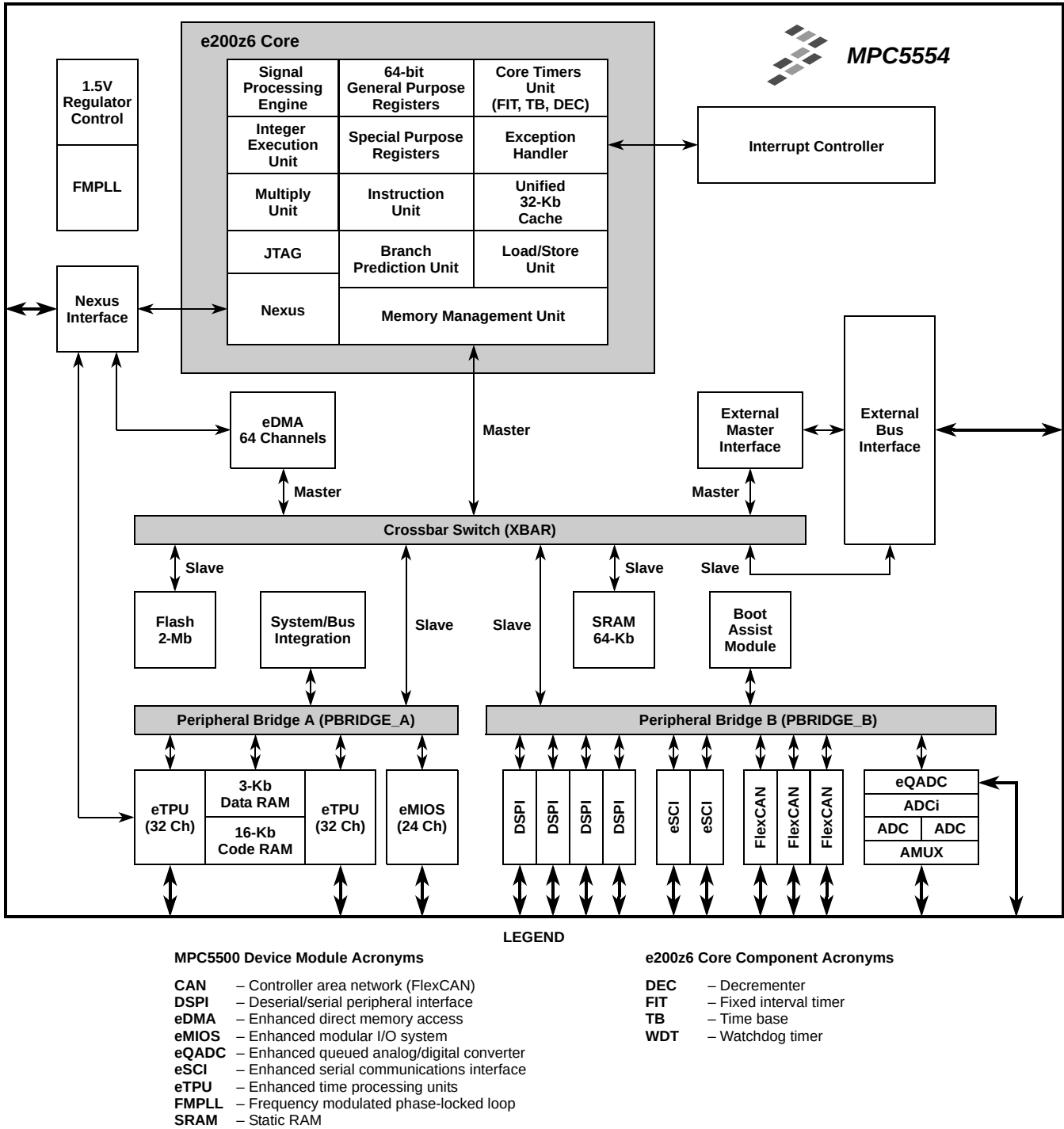
Figure 5. MPC5554 Block Diagram
