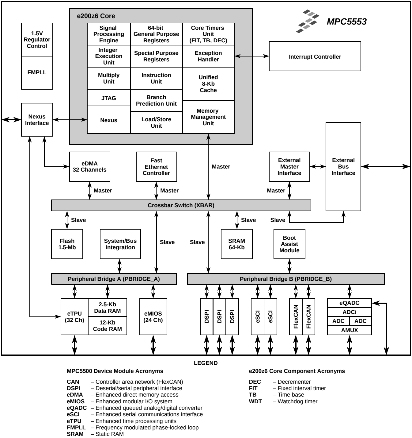
Figure 4. MPC5553 Block Diagram
