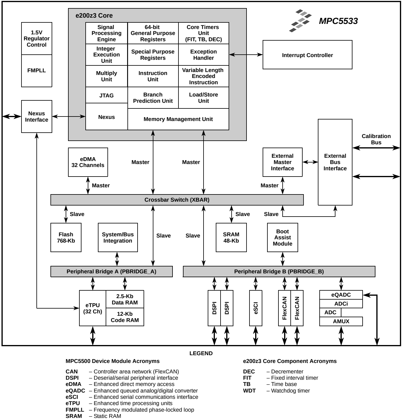
Figure 2. MPC5533 Block Diagram
