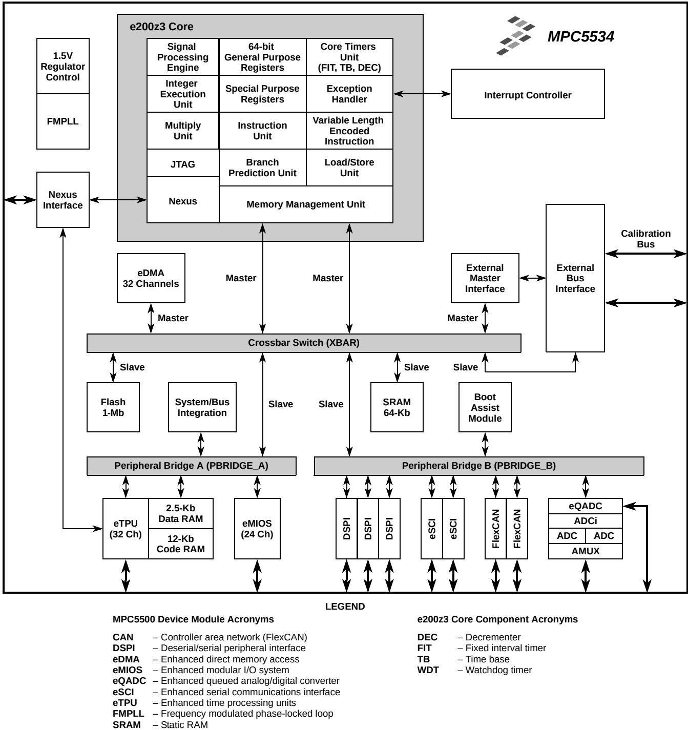
Figure 3. MPC5534 Block Diagram
