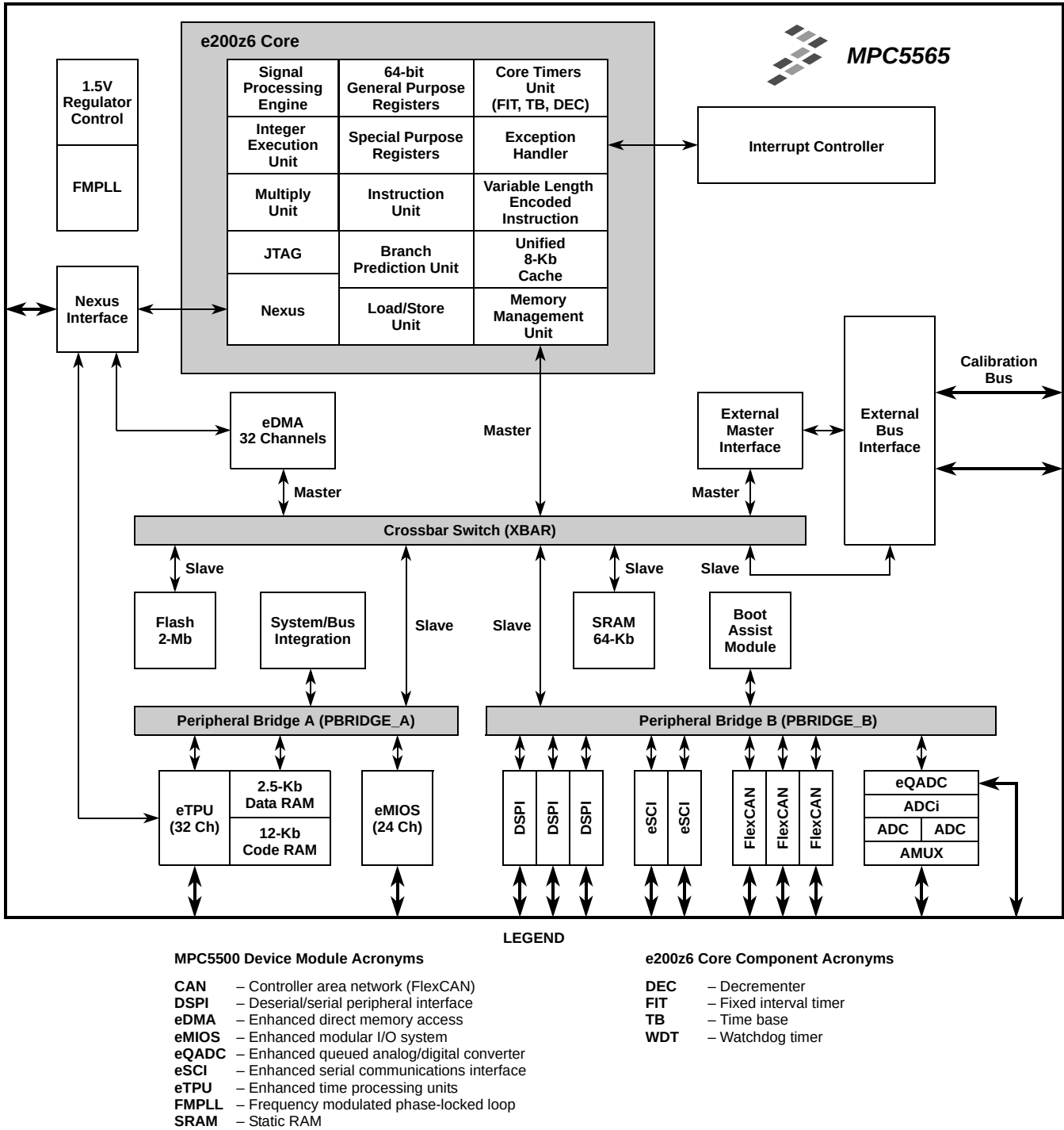
Figure 7. MPC5565 Block Diagram
