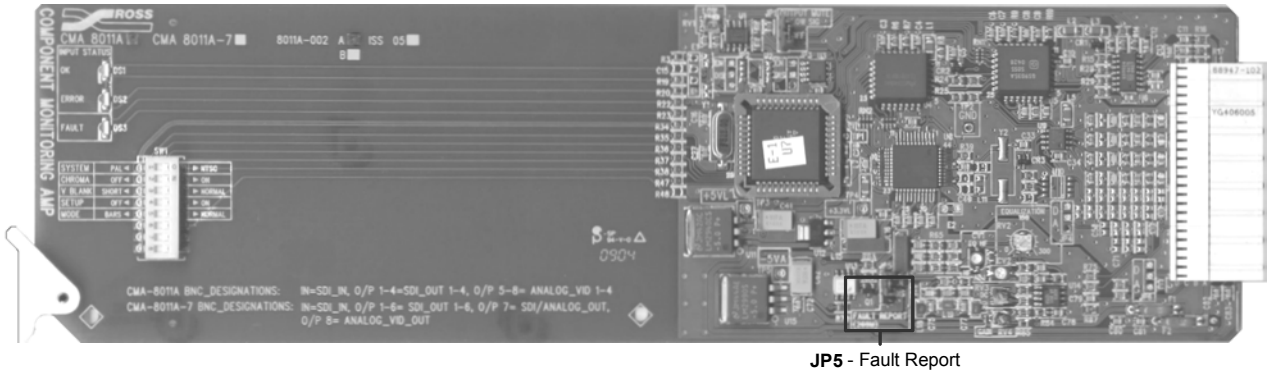
Figure 6. SMPTE 269M Alarm Reporting Jumper Location
