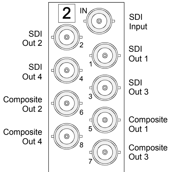
Figure 3. Cabling Designations for RossGear 8000 Series Frames
