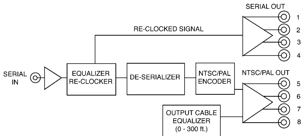
Figure 1. Simplified Block Diagram of CMA-8011A Functions
