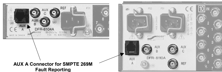
Figure 7. SMPTE 269M Alarm Reporting Frame Connections
