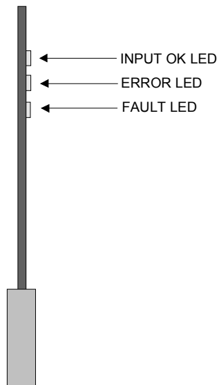
Figure 4. LEDs
