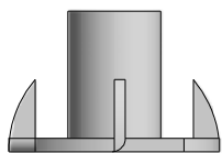
(9) - T-NUT 3/8 - H100073
