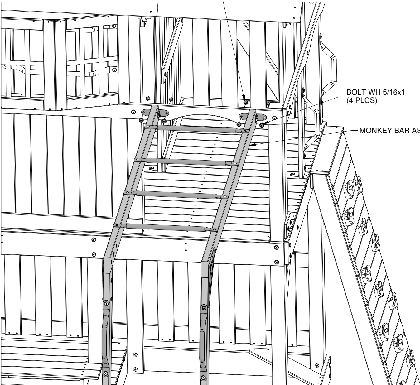
T-NUT 5/16 (4 PLCS)
