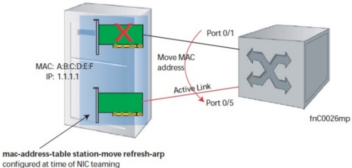
Figure 18. MAC Address Station Move
