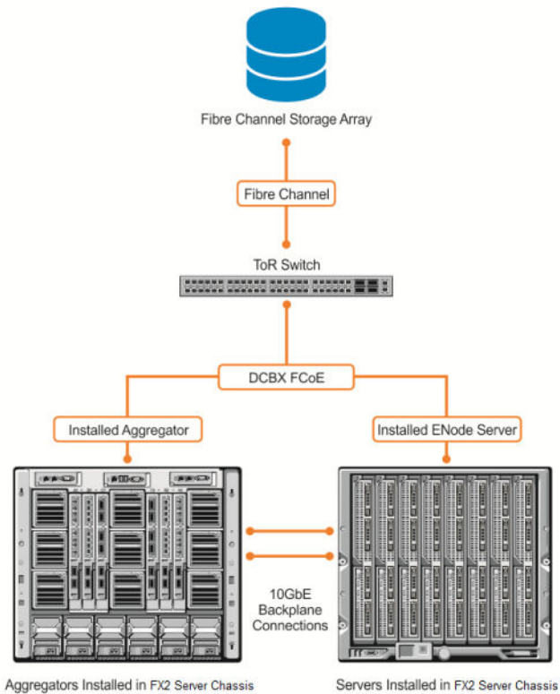
Figure 9. FIP Snooping on an Aggregator
