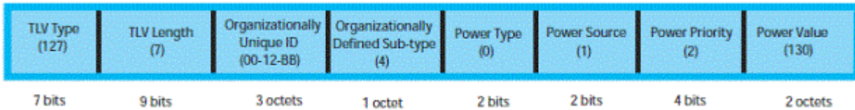
Figure 25. Extended Power via MDI TLV
