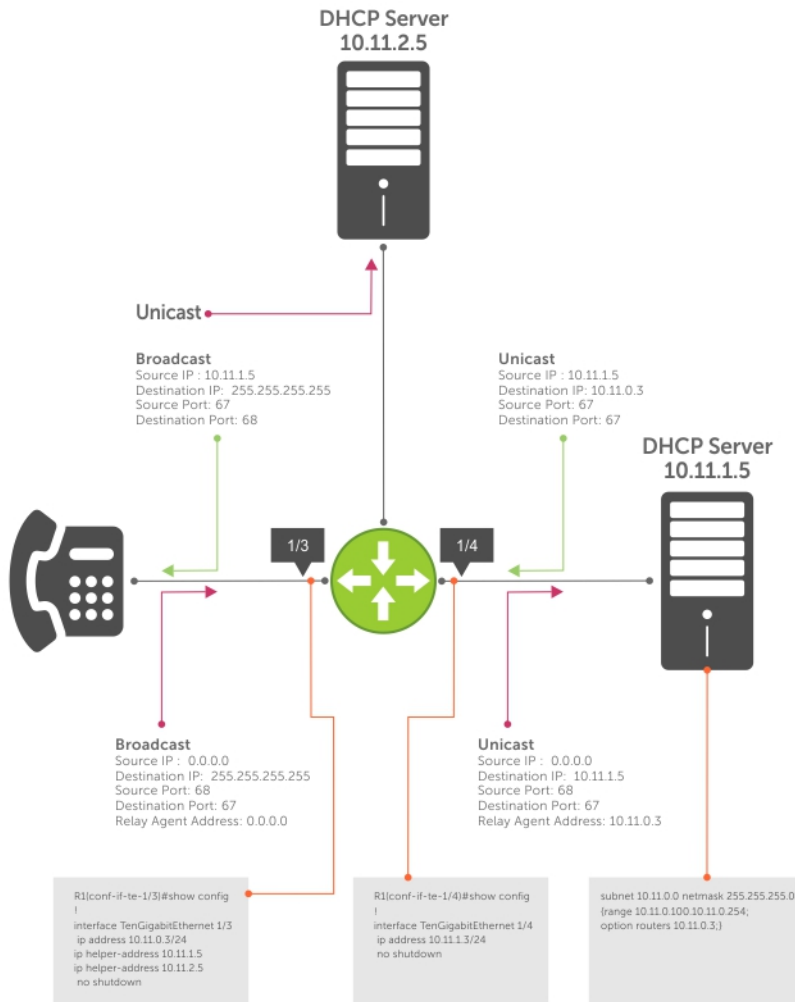
Figure 5. Assigning Network Parameters using DHCP
