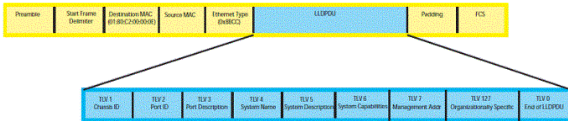
Figure 20. LLDPDU Frame
