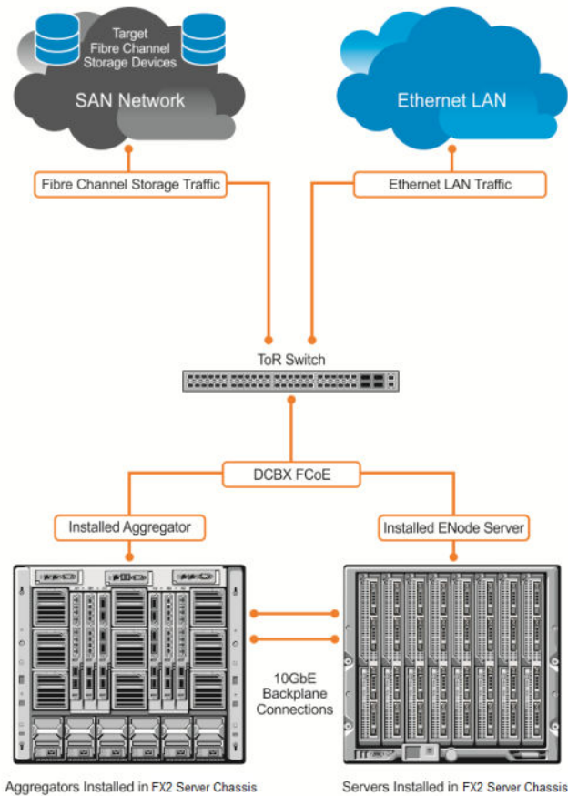
Figure 8. FIP Snooping on an Aggregator
