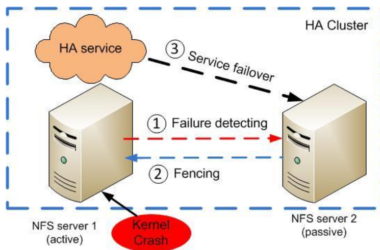
Figure 2. A failure scenario in NSS-HA
