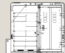
Style-C Roll-up, Right Hand Swing
