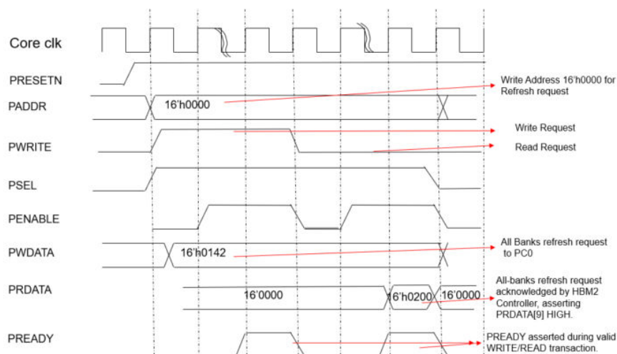
Figure 30. Timing of APB Refresh Request to All Banks
