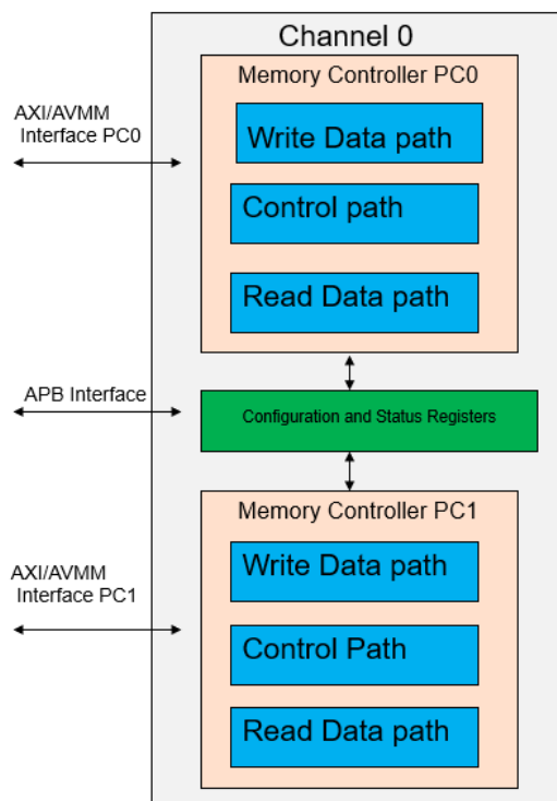
Figure 5. Intel Stratix 10 HBM2 Controller Block Diagram
