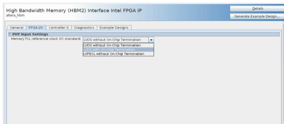
Figure 8. FPGA I/O Tab
