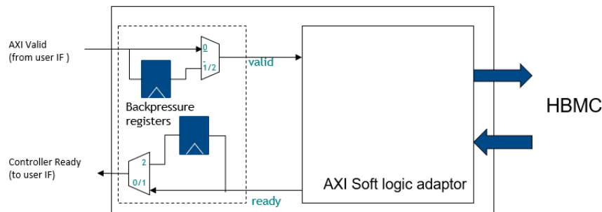
Figure 26. Non-zero Latency Backpressure Implementation
