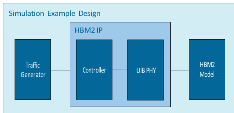
Figure 12. High Bandwidth Memory (HBM2) Interface Intel FPGA IP Generated for Simulation
