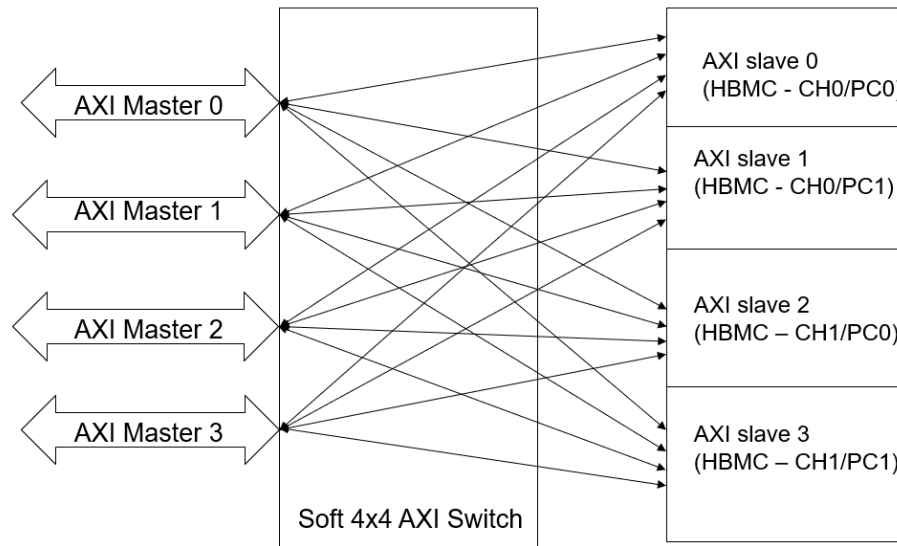
Figure 31. 4x4 HBM2 AXI Switch
