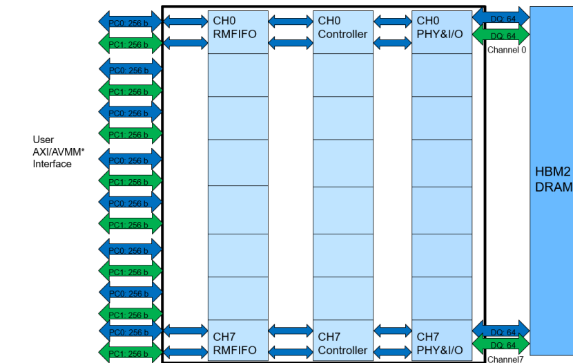
Figure 4. Intel Stratix 10 HBM2 Interface Using HBM2 Channels 0 and 7 through the UIBSS
