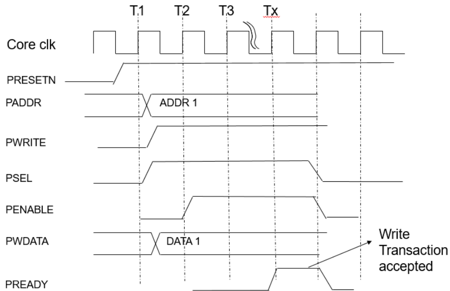
Figure 27. APB Write Transaction
