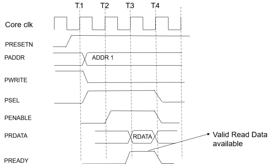
Figure 28. APB Read Transaction
