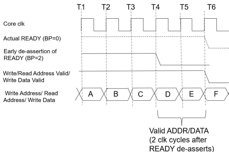
Figure 25. Early Controller READY Deassertion Using Backpressure Latency
