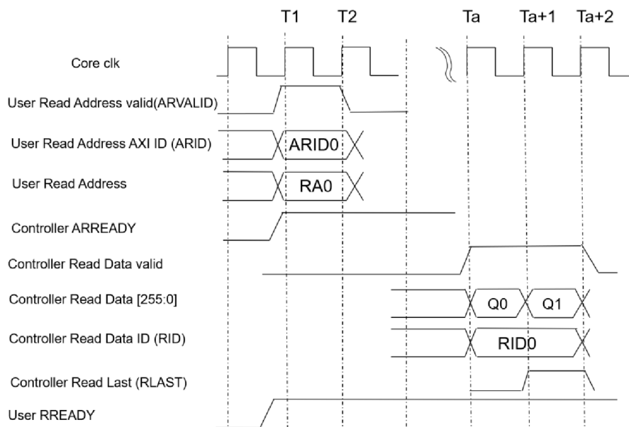
Figure 23. AXI Read Transaction – Using Pseudo-BL8 Memory Read Transaction
