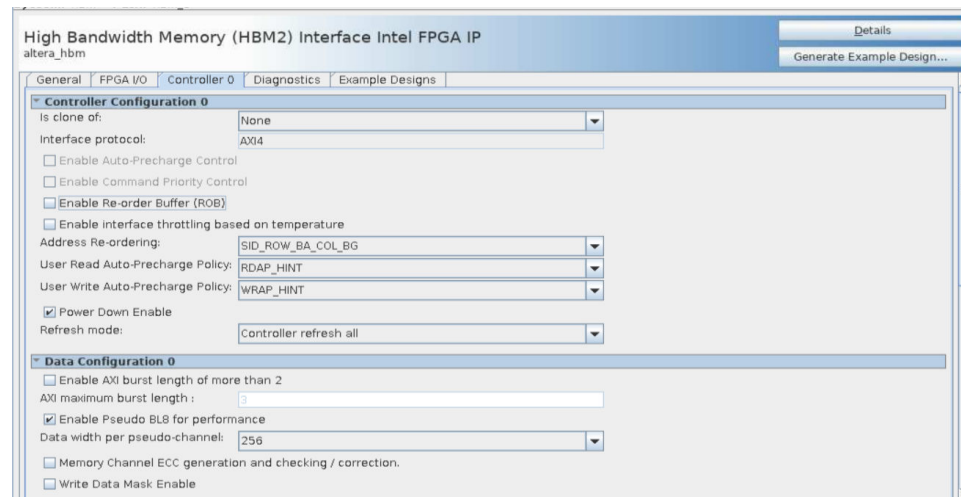
Figure 13. Controller Tab Settings for High Efficiency Simulation
