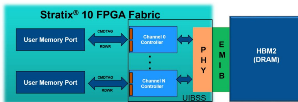
Figure 1. Intel Stratix 10 Device with UIB, EMIB, and HBM2 DRAM
