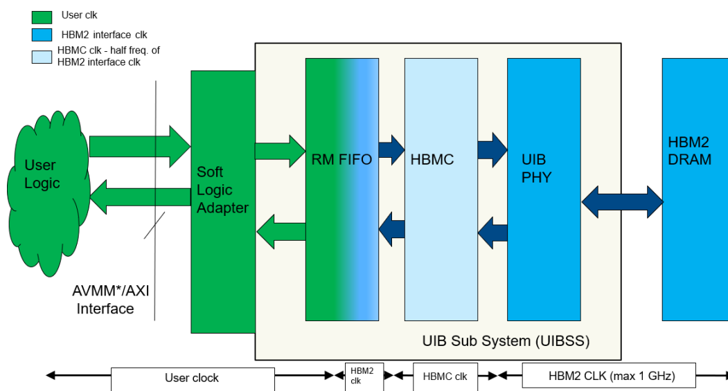
Figure 3. Block Diagram of Intel Stratix 10 HBM2 Implementation
