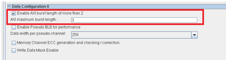
Figure 20. Parameters to Enable BL>2 and Set Maximum Burst Length
