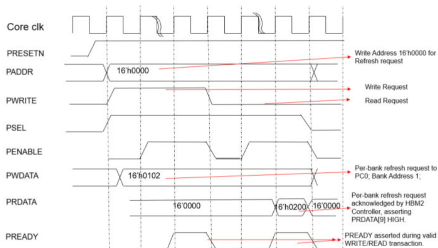
Figure 29. Timing of APB Refresh Request Per Bank
