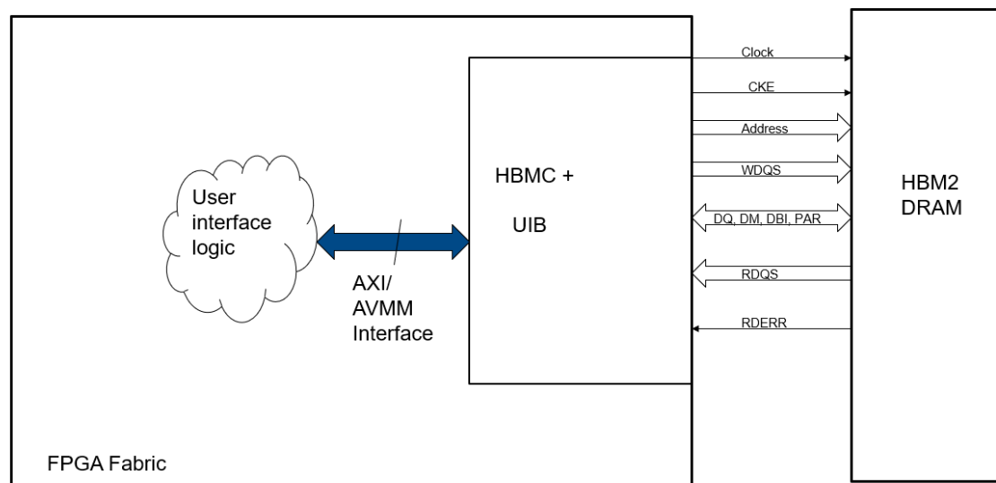
Figure 15. High Level Block Diagram of HBM2 Implementation
