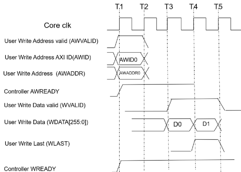
Figure 22. AXI Write Transaction – Using Pseudo-BL8 Memory Write Transaction
