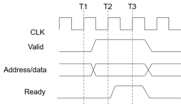
Figure 21. AXI Protocol Handshake Process
