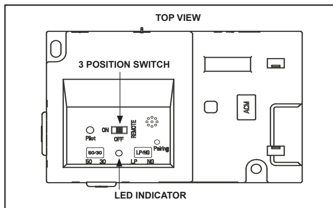
Figure 3.6. IFT-ECM
