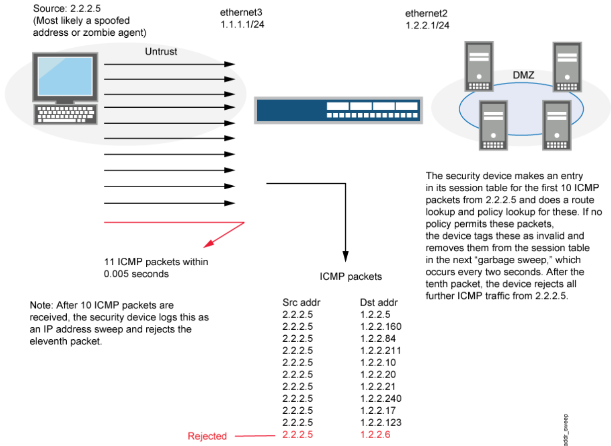
Figure 23: Address Sweep
