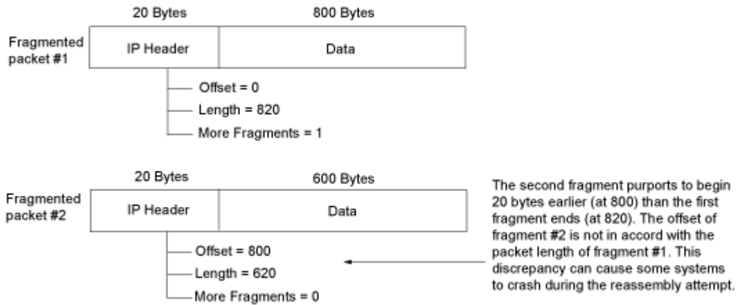
Figure 12: Fragment Discrepancy
