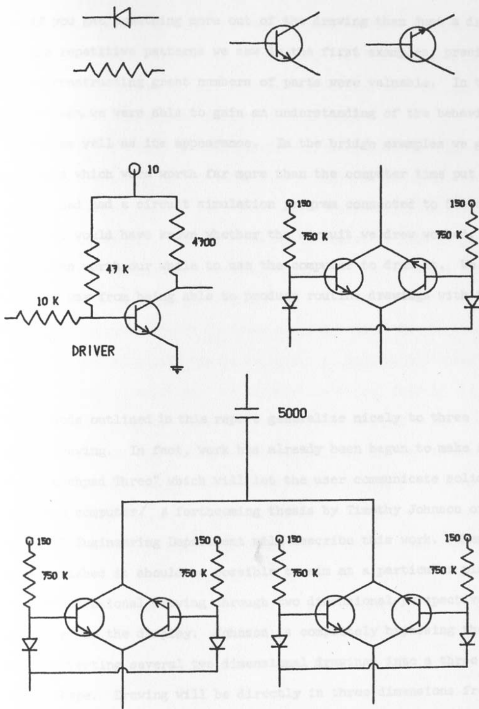
FIGURE 9.11. CIRCUIT DIAGRAMS
