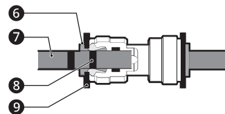
⑥ Collet ⑦ Tube ⑧ Insert line ⑨ Clip
