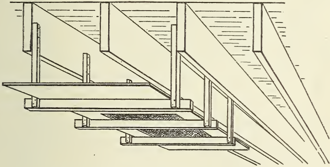
FIGURE 10.—A convenient screen storage rack
