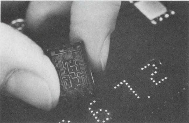
LED numerics in a 4 × 7 dot matrix from HP have an on-board decoder/driver with memory.
