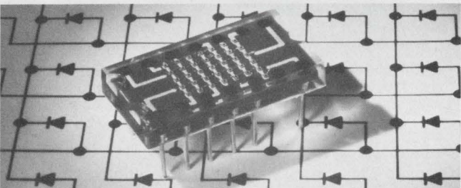
A 5 × 7 LED matrix from TI provides full-alphanumeric capability with 300-mil characters.
