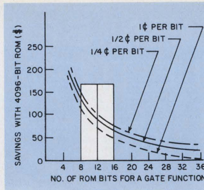
4. The savings incurred by substituting bits of 4096-bit ROM for gate functions can reach 80%.
