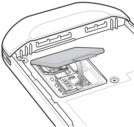
Figure 21 Replace Access Door
