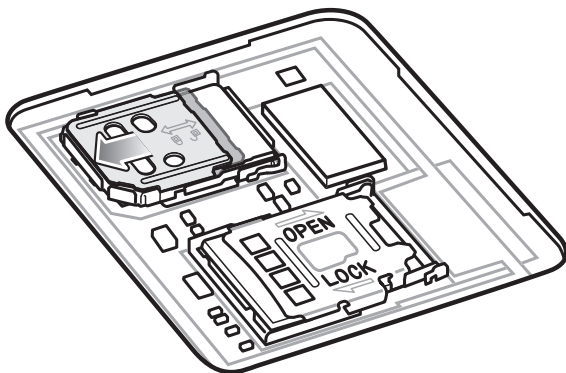
Figure 14 Lock SIM Card Holder Door
