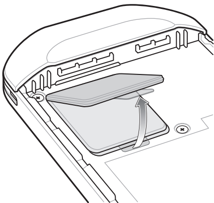
Figure 22 Remove Access Door
