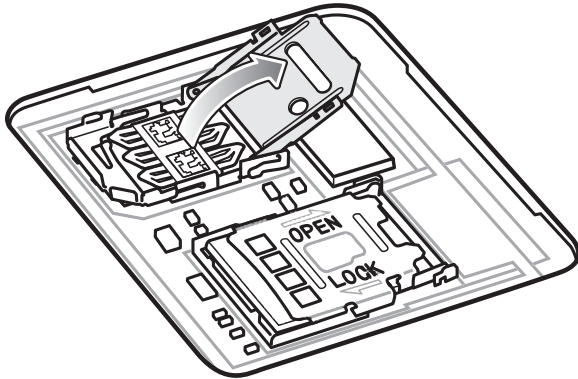
Figure 24 Lift the SIM Card Door
