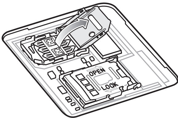
Figure 11 Lift the SIM Card Holder
