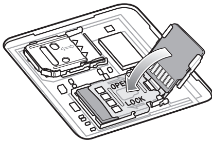
Figure 7 Re-install Access Door
