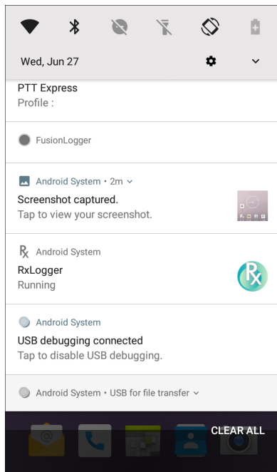
Figure 37 Notification Panel
