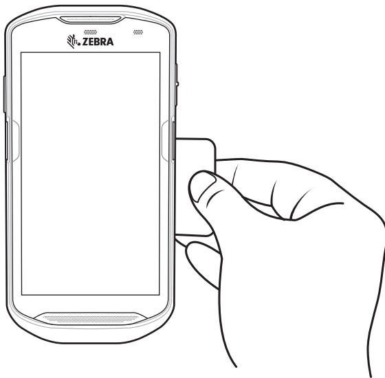
Figure 134 Reading Cards
