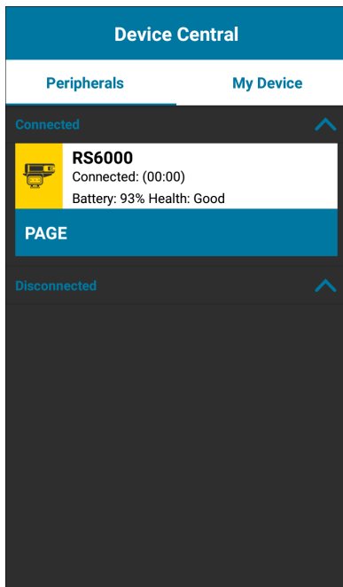
Figure 72 Peripherals Tab
