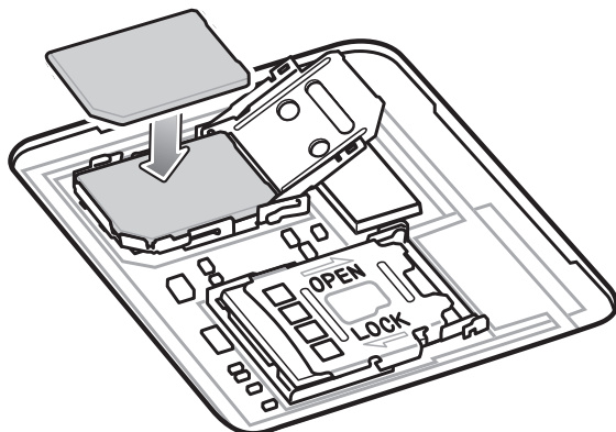
Figure 12 Place SIM Card in Holder
