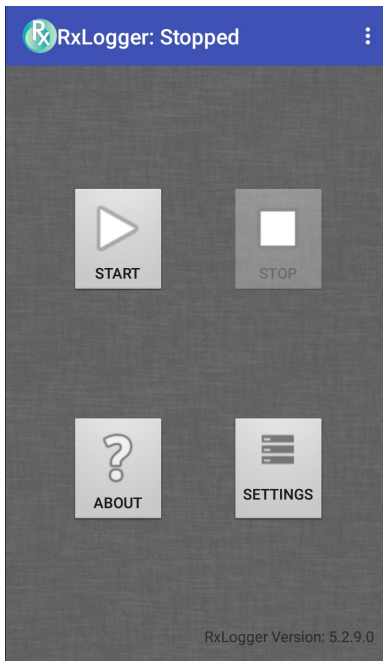
Figure 92 RxLogger
