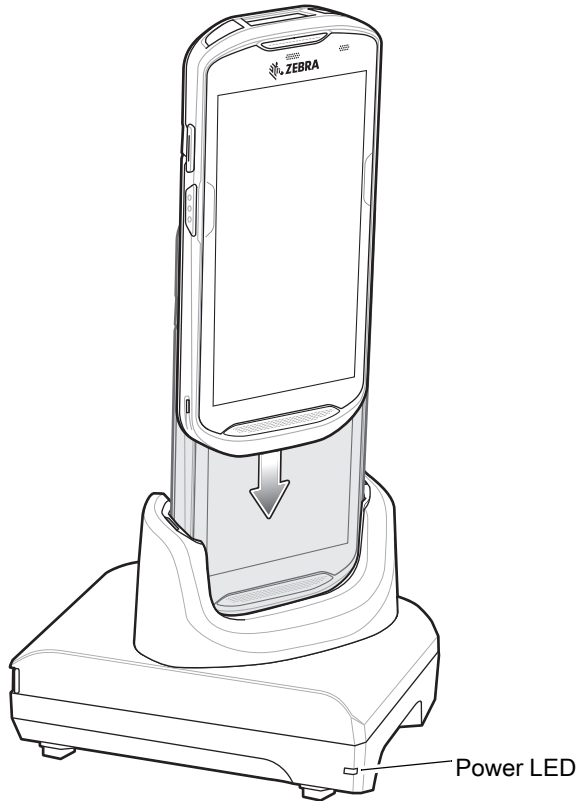
Figure 137 Battery Charging
