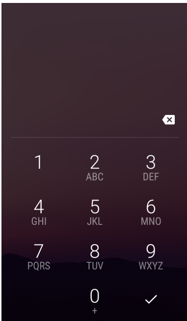
Figure 43 PIN Screen
