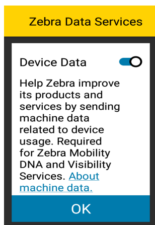
Figure 17 Zebra Services
