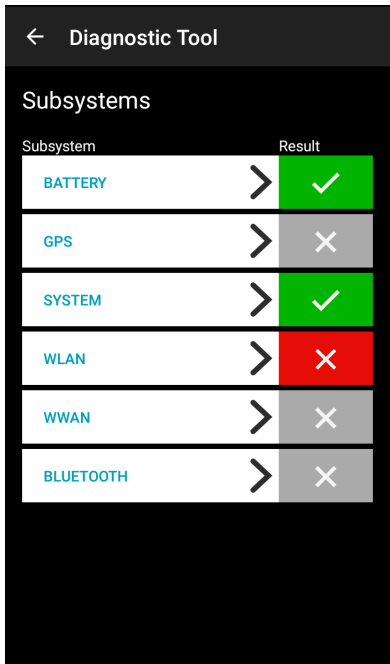
Figure 78 Subsystem Screen
