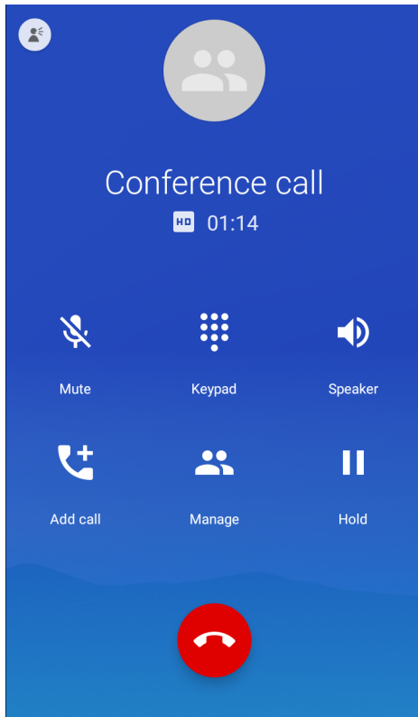
Figure 55 Merged Calls
