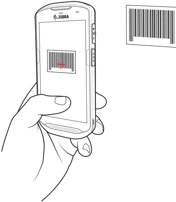
Figure 111 Camera Scanning
