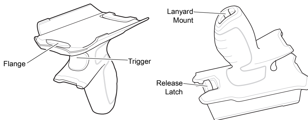
Figure 163 Trigger Handle
