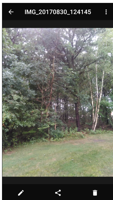
Figure 84 Photo Example
