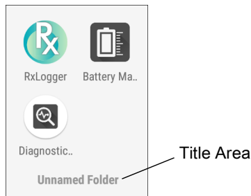
Figure 40 Open Folder
