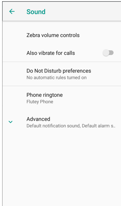
Figure 33 Sound Screen
