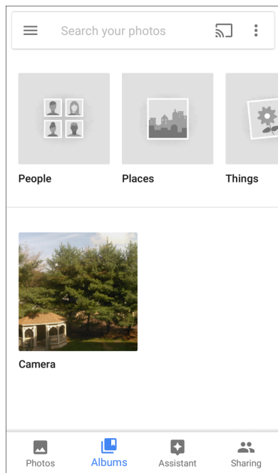
Figure 87 Albums View
