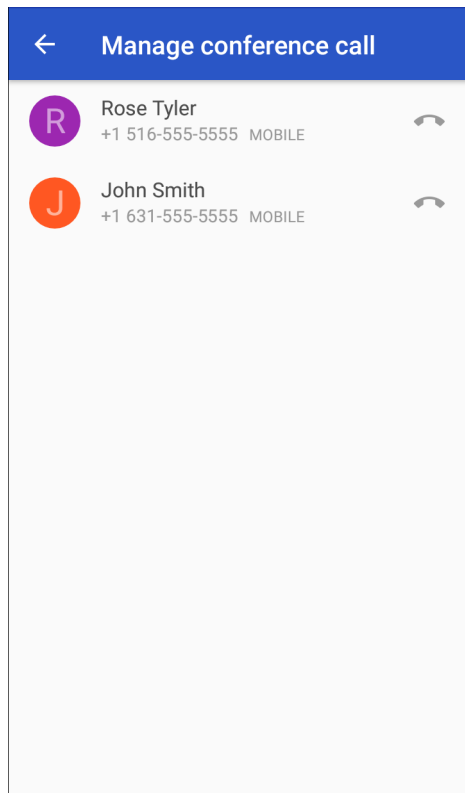
Figure 56 Un-merge Calls
