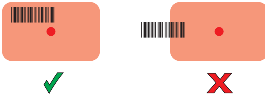
Figure 109 Aiming Pattern
