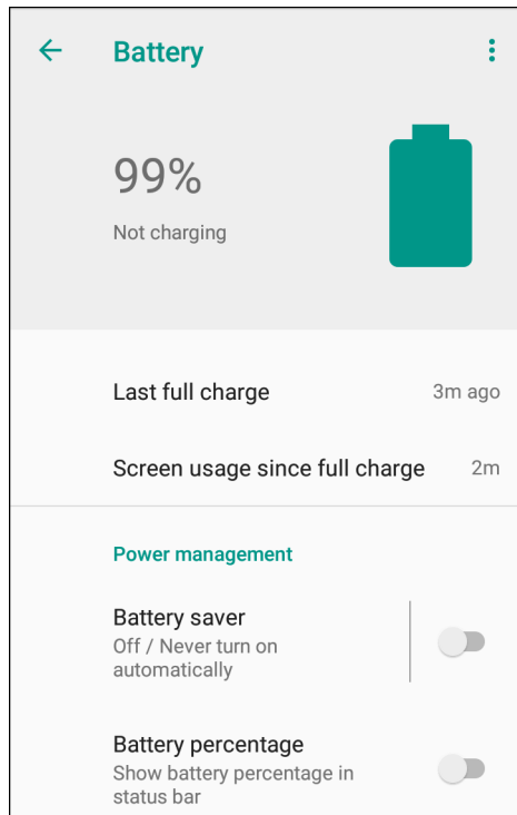
Figure 27 Battery Screen
