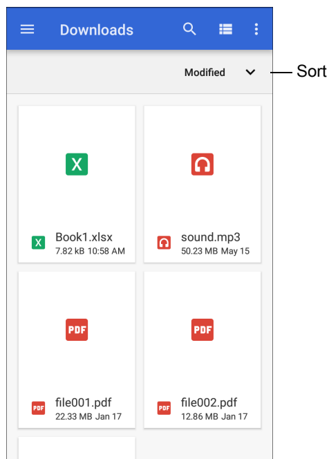
Figure 80 Files Screen
