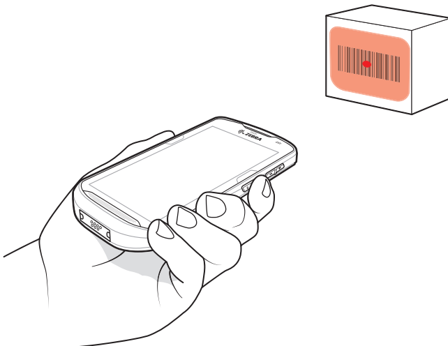
Figure 108 Imager Scanning
