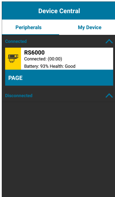
Figure 73 Page RS6000
