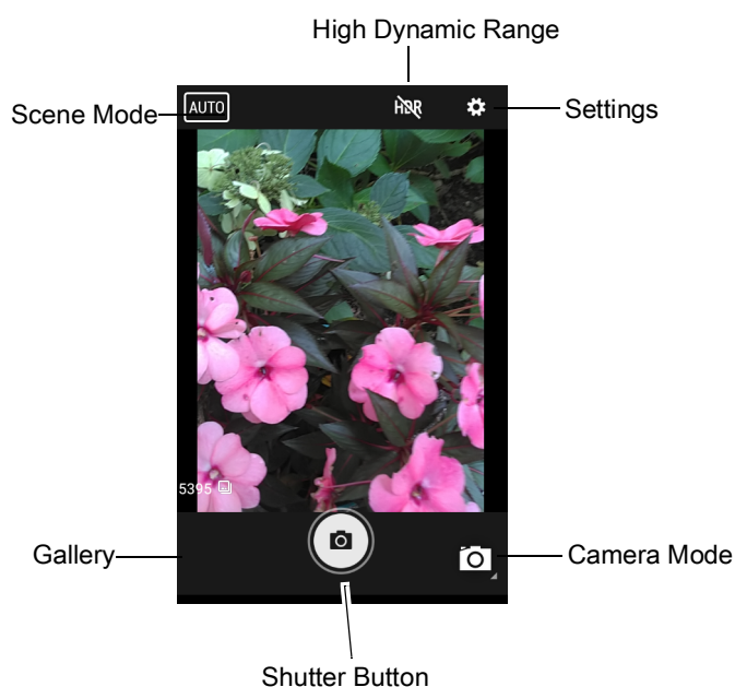
Figure 68 Camera Mode
