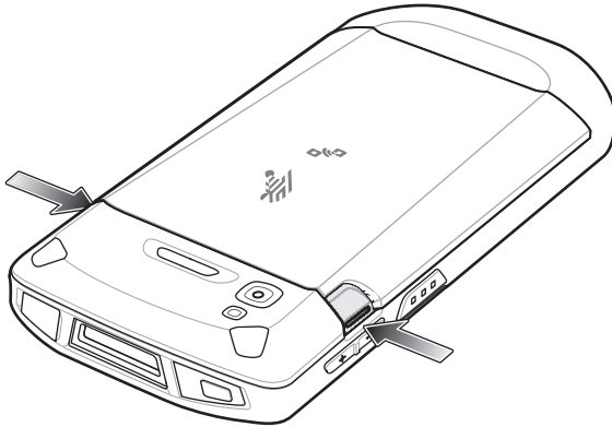
Figure 18 Press Battery Latches
