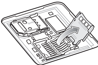
Figure 5 Lift the microSD Card Holder
