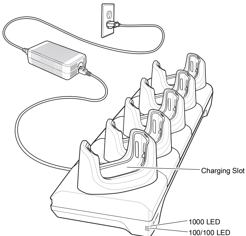
Figure 146 5-Slot Ethernet Cradle
