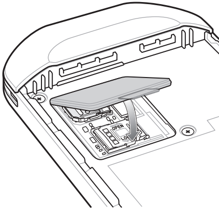
Figure 26 Replace Access Door
