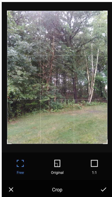
Figure 85 Cropping Tool
