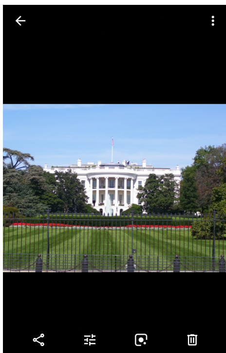
Figure 89 Photo Example
