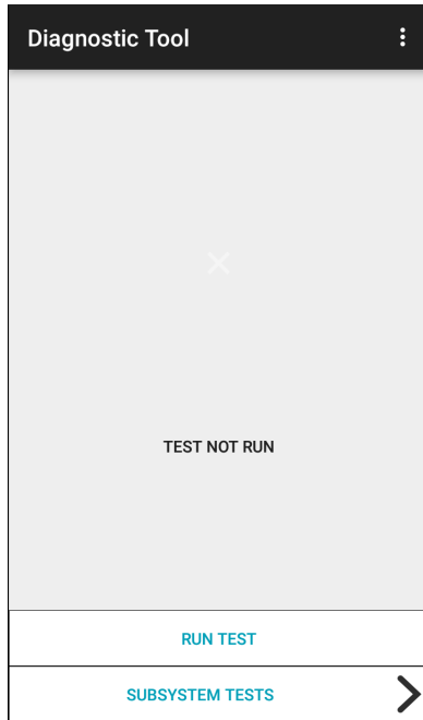
Figure 75 Diagnostic Tool
