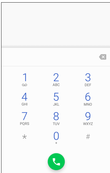
Figure 48 Dialer Screen
