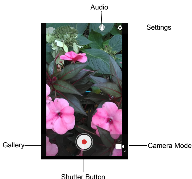
Figure 70 Video Mode
