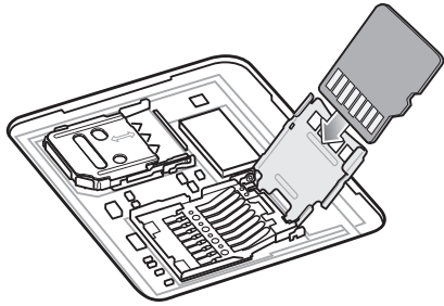
Figure 6 Insert microSD Card in Holder
