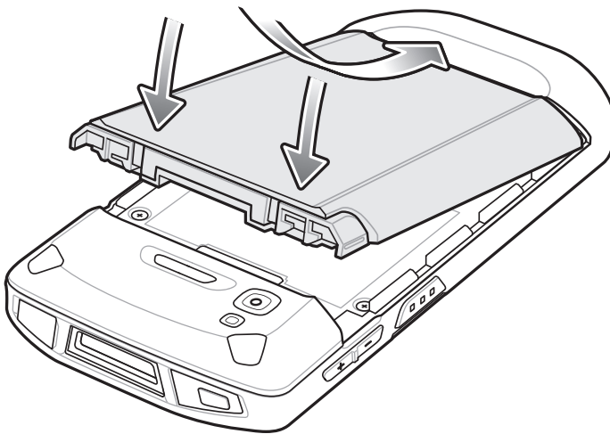
Figure 16 Insert Bottom of Battery into Battery Compartment
