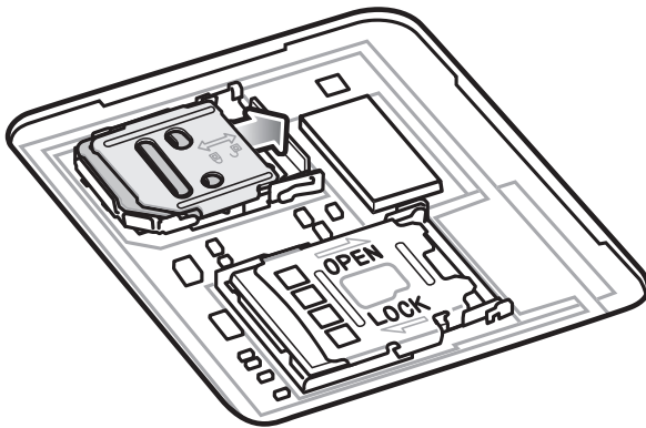
Figure 10 Unlock SIM Card Holder
