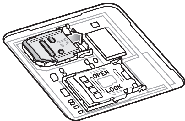
Figure 23 Unlock SIM Card Door
