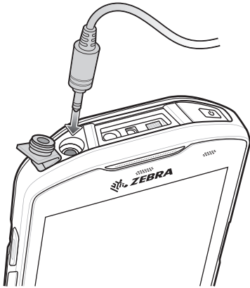
Figure 47 3.5 mm Headset Adapter
