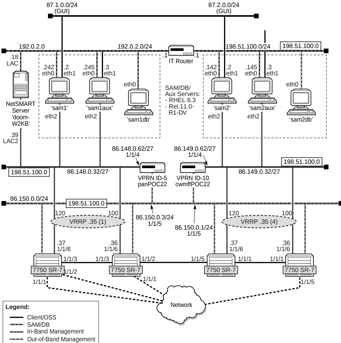
Figure 5-3 Management network
