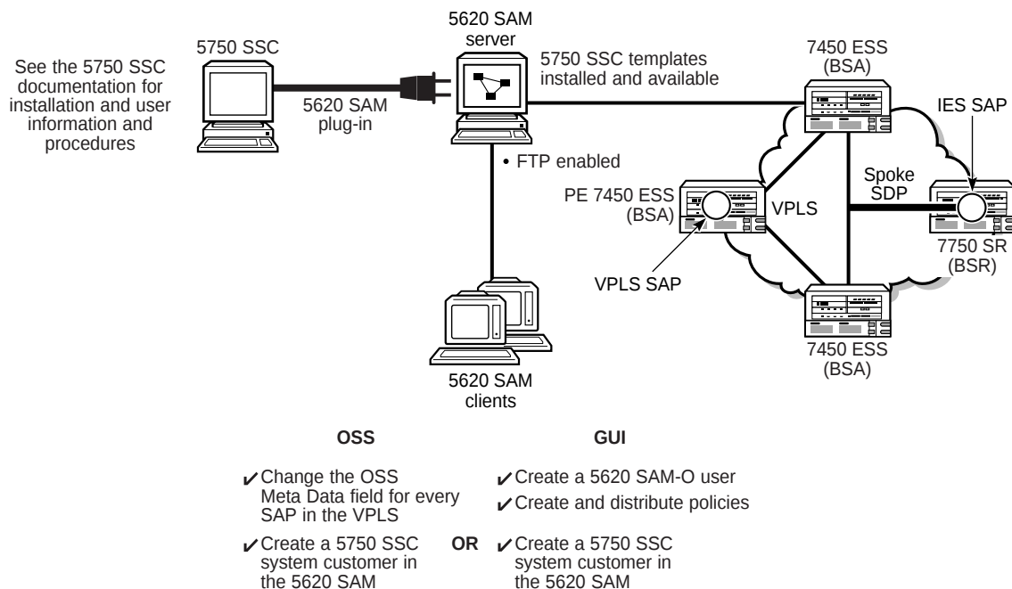
Figure 2-3 5750 SSC and 5620 SAM integration
