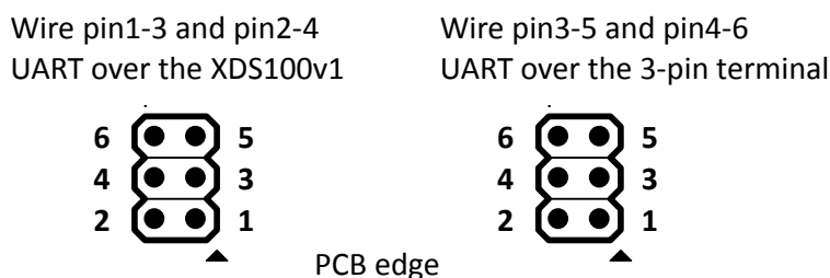
Figure 3.3: COM_SEL1 Jumper setting
