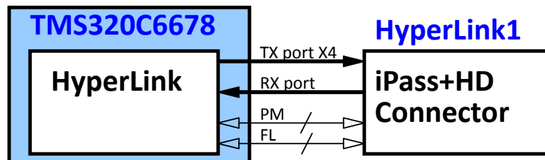
Figure 2.8: TMDSEVM6678L EVM HyperLink connections
