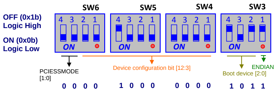
Figure 3.6 : SW3, SW4, SW5, and SW6 default settings
