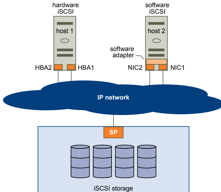
Figure 9-3. Host-Based Multipathing
