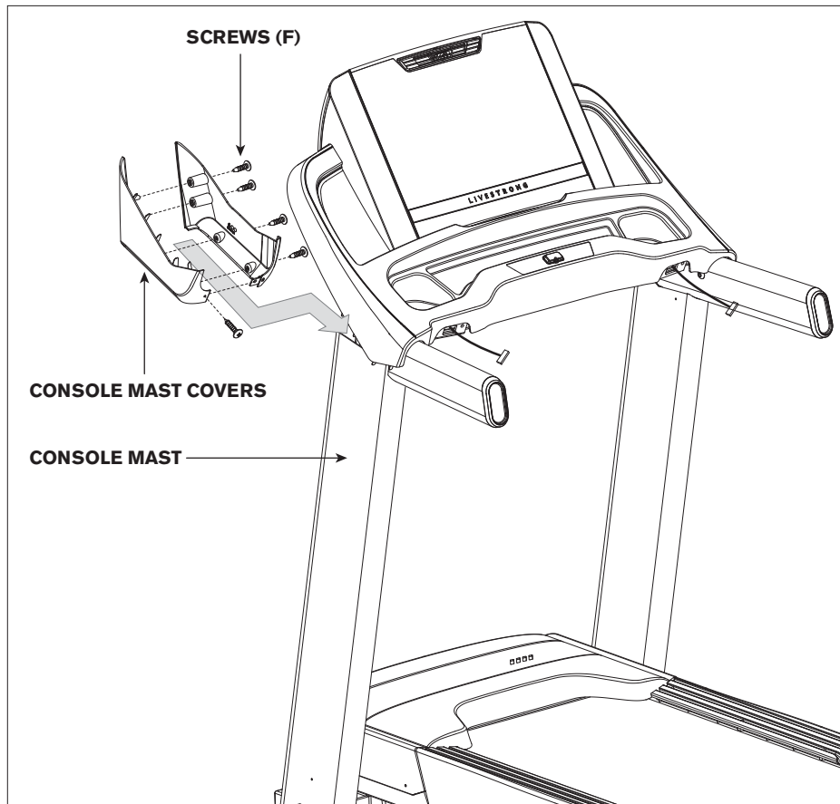
SCREW (F) 15 mm Qty: 10
