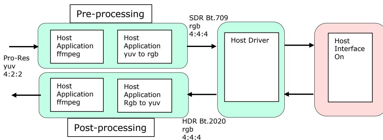
Figure 1: Software configuration
