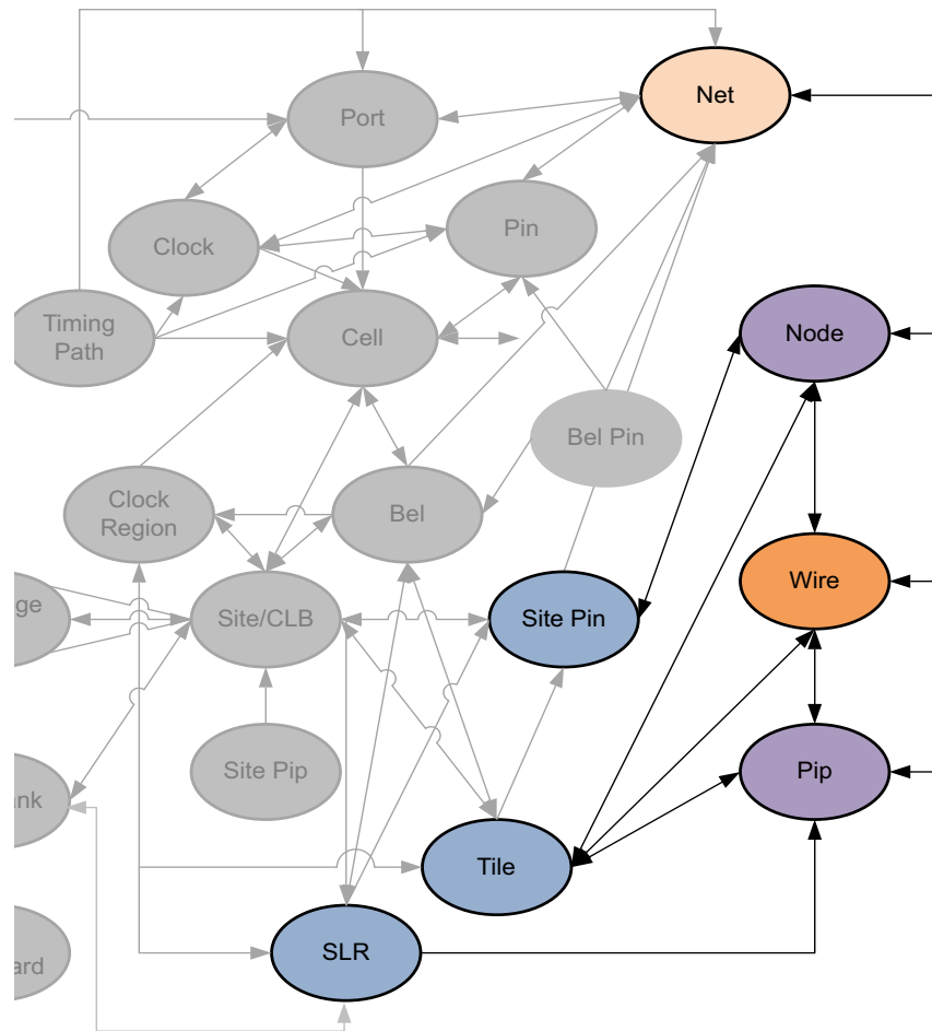
Figure 2-41: WIRE Objects
