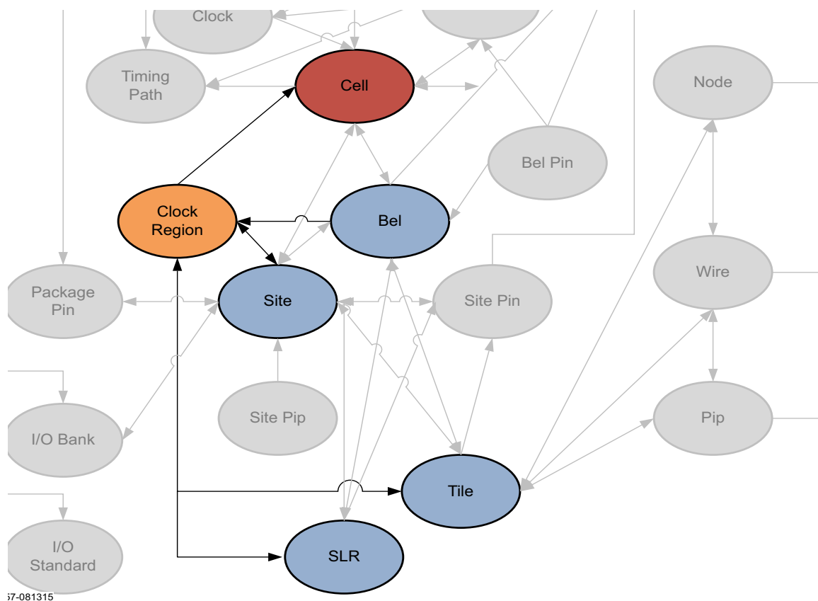
Figure 2-14: CLOCK_REGION Objects
