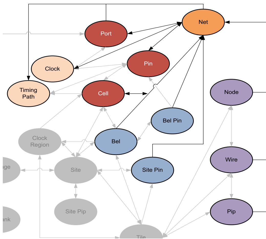
Figure 2-29: NET Objects
