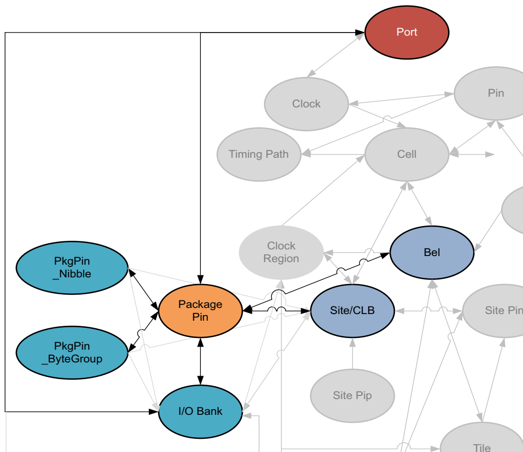
Figure 2-31: PACKAGE_PIN Objects
