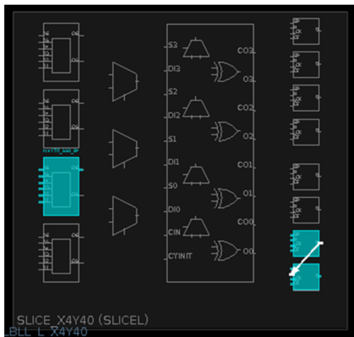
Figure 3-2: Grouping Registers
