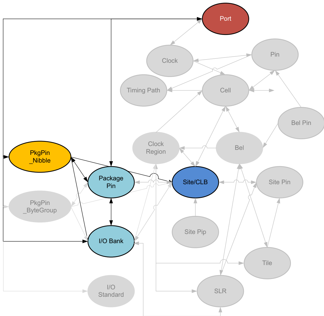
Figure 2-35: PKGPIN_NIBBLE Objects
