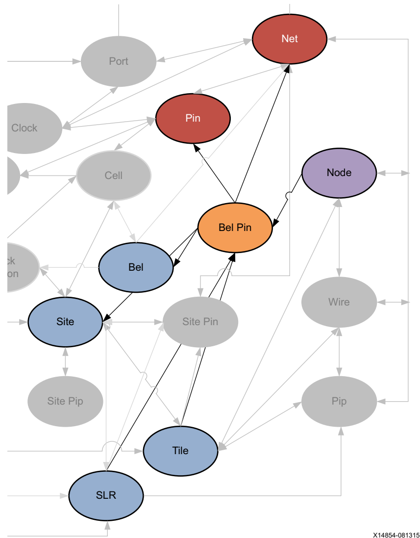
Figure 2-11: BEL_PIN Objects
