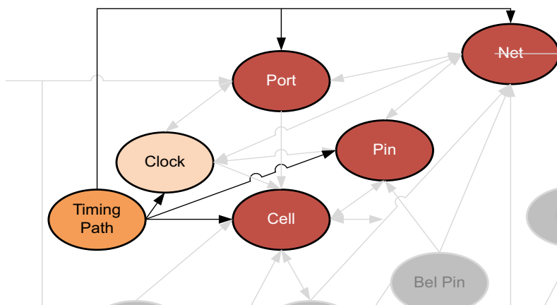
Figure 2-40: TIMING_PATH Objects
