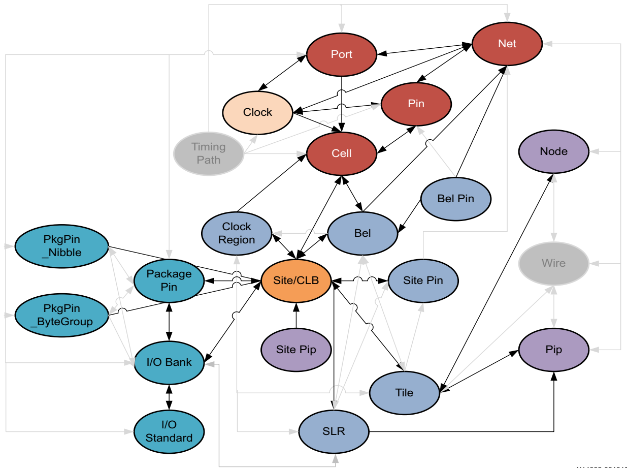
Figure 2-37: SITE Objects
