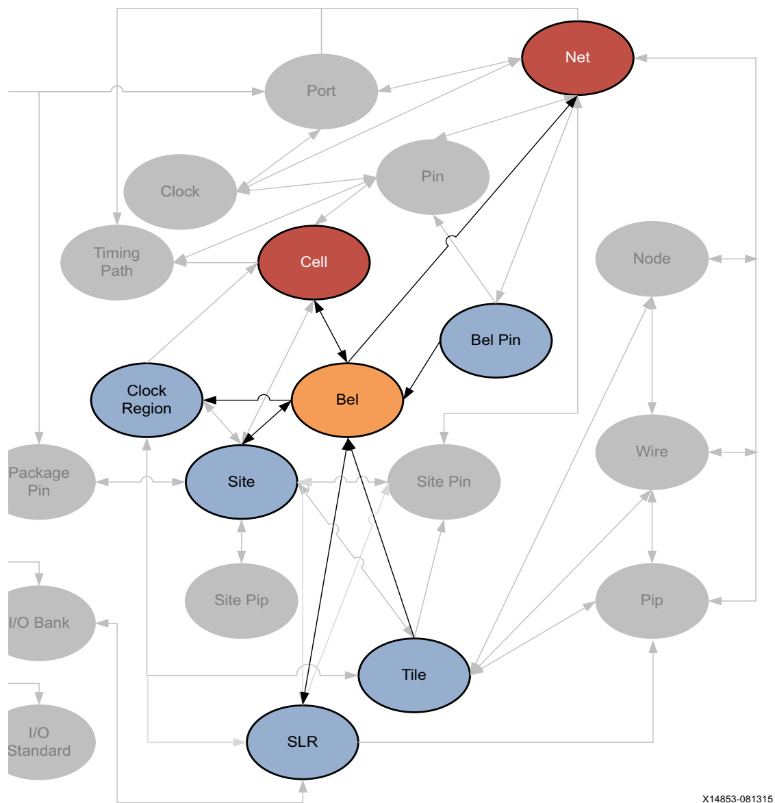
Figure 2-10: BEL Objects
