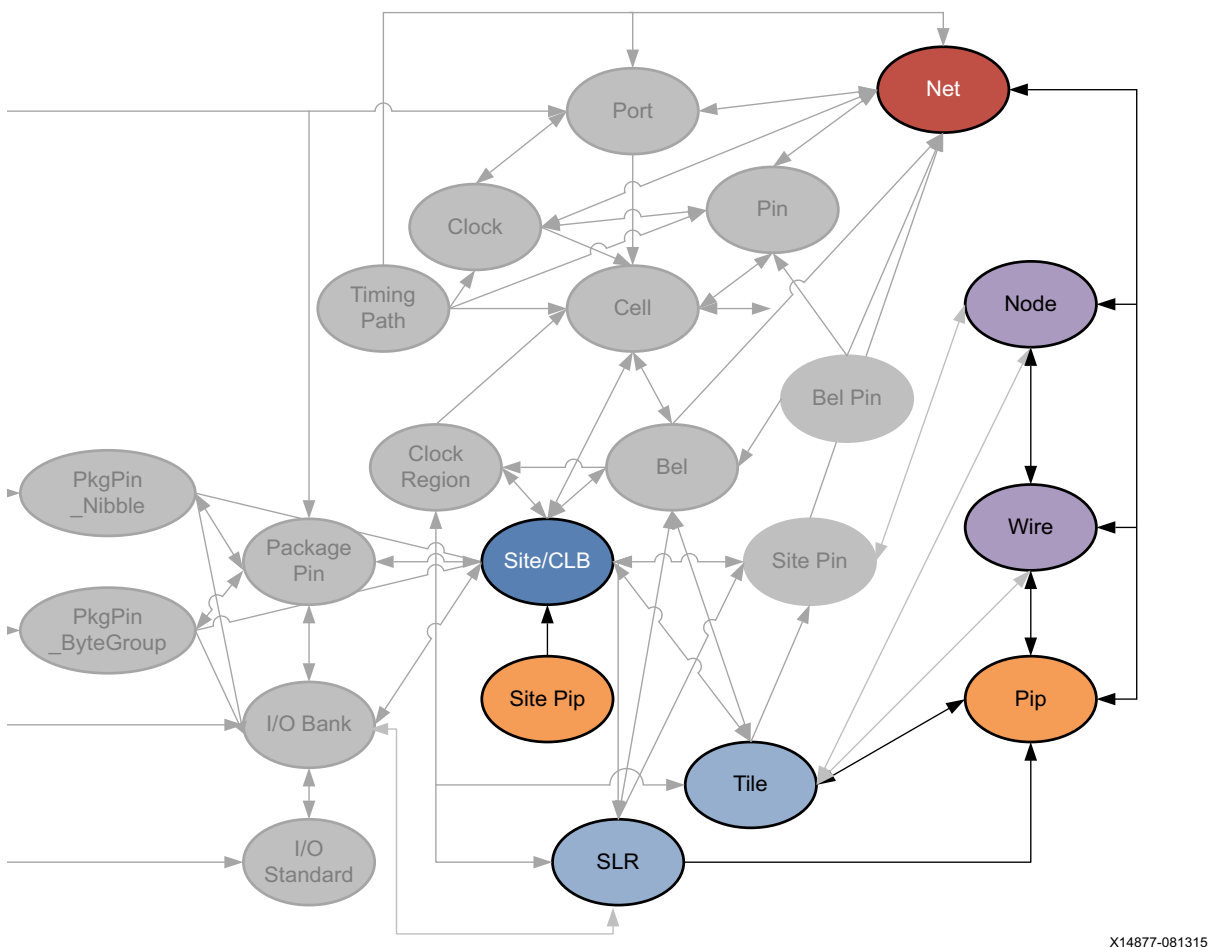
Figure 2-33: PIP Objects
