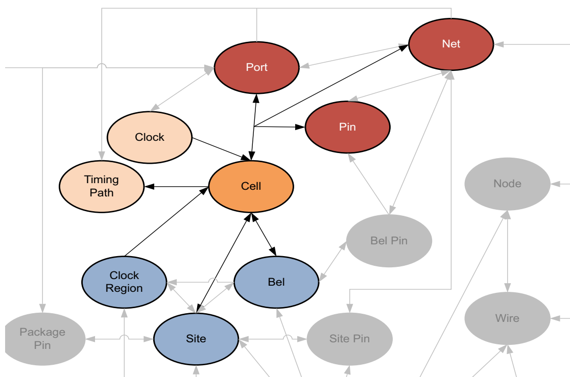
Figure 2-12: CELL Objects
