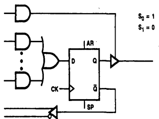
Registered/Active HIGH
