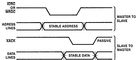
Figure 3-157.a Read AC Timing
