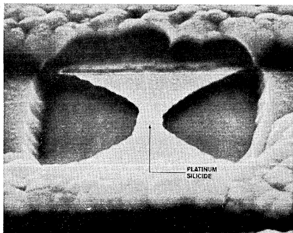
Unprogrammed Fuse
