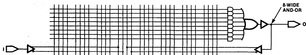
Figure 1-17.b Active-HIGH Dedicated Output
