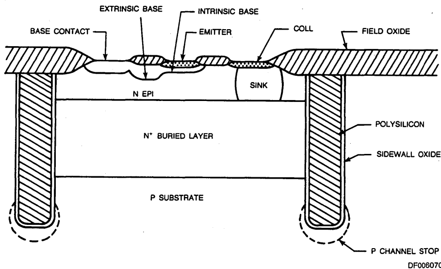
Figure 2-18. Slot Isolation
