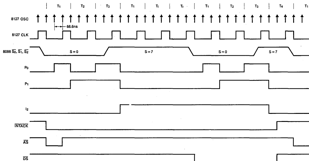
Figure 3-148. Interrupt Acknowledge Timing Diagram
