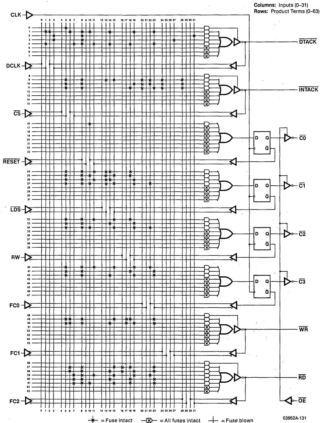
Figure 3-95. Logic Diagram for Slow Am8500 to MC68000 Using AmpAL16R4/AmpAL16R4A
