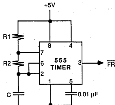
Figure 3-190. Refresh Timer Diagram
