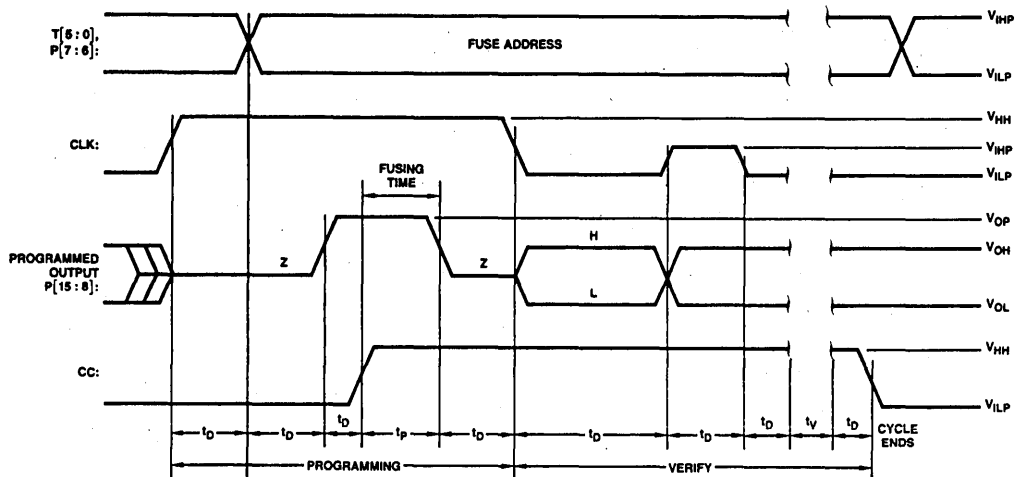
Programming Waveforms
