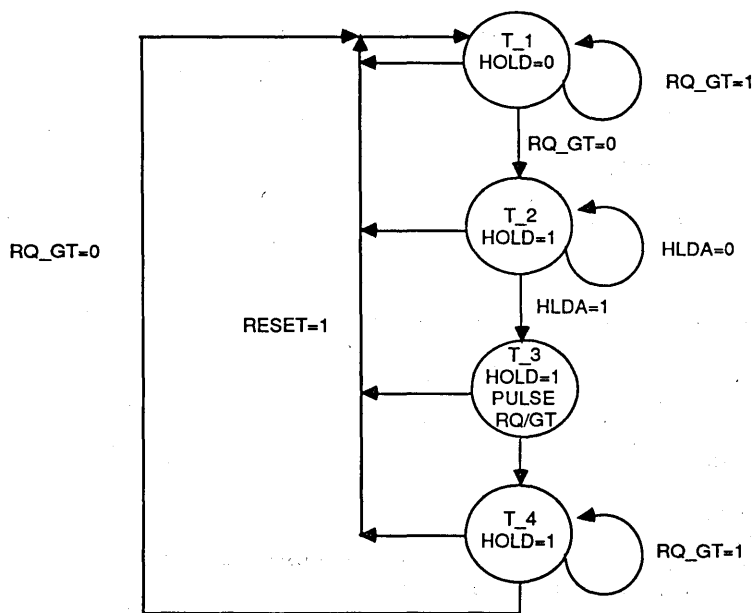
Figure 3-217. RQ/GT0-to-Hold/HLDA Converter
