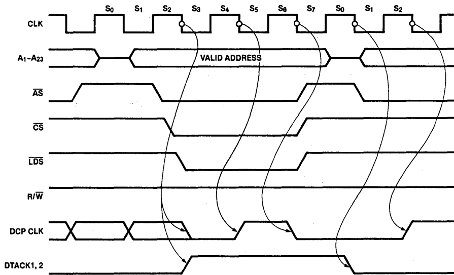
Figure 3-78. 68000-AmZ8068 Data Read Cycle ( A_1 = \text{HIGH} )
