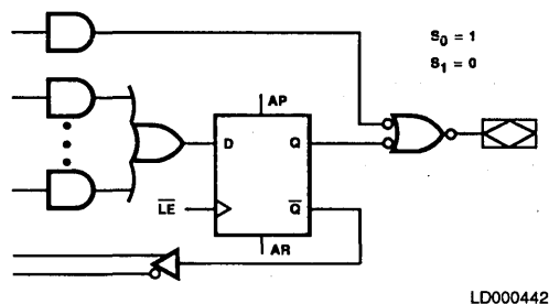
Figure 3-2. Registered/Active-HIGH
