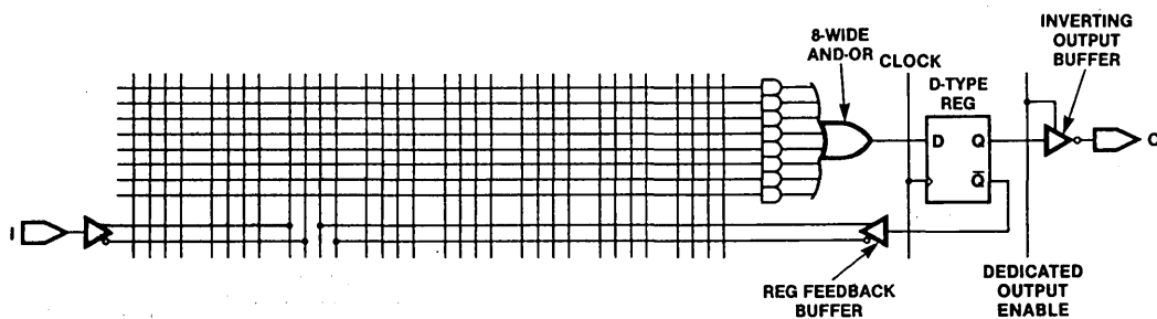
Figure 1-18 Registered Output
