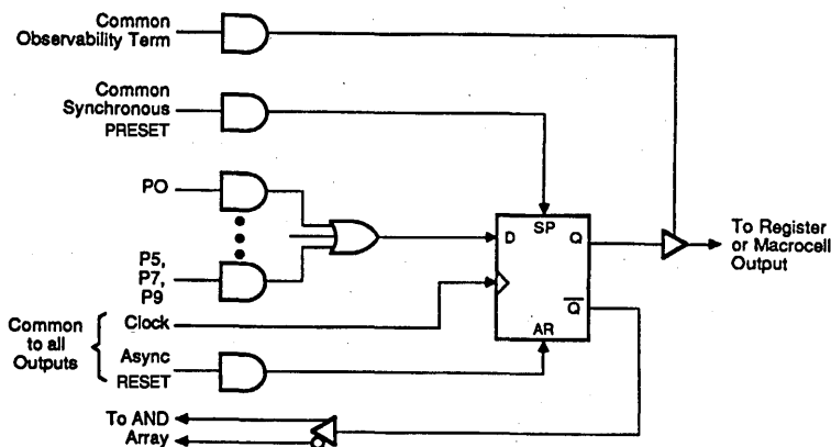
Figure 1-23. AmPAL23S8 Buried State Register
