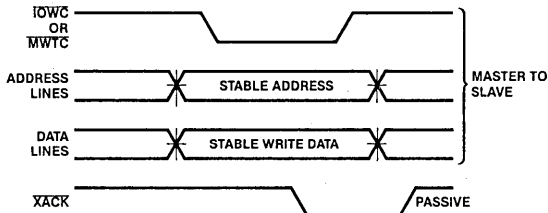
Figure 3-157.b Write AC Timing
