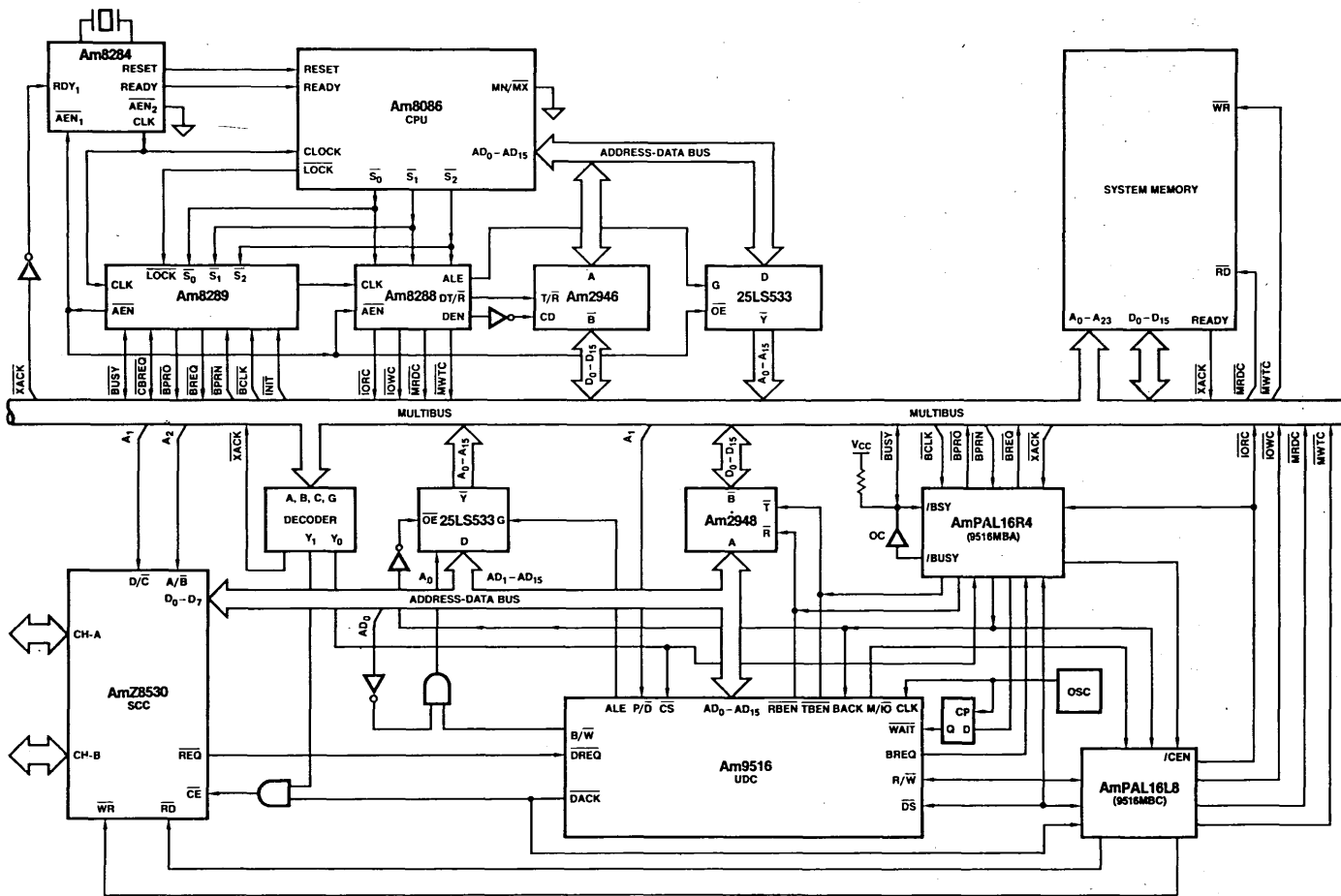
Figure 3-143. Am9516 to 8086 in a MULTIBUS® Environment
