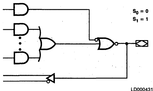
Figure 3-3. Combinatorial/Active-LOW
