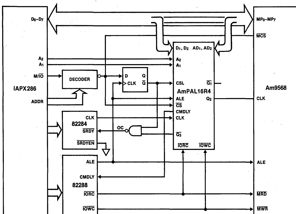
Figure 3-62. IAPX286-Am9568 Interface
