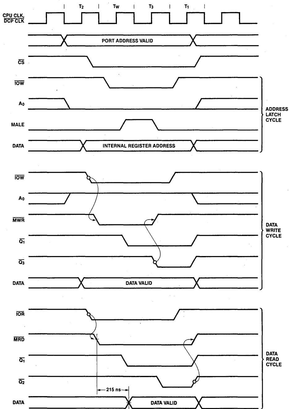
Figure 3-132. CPU-DCP Timing Diagram
