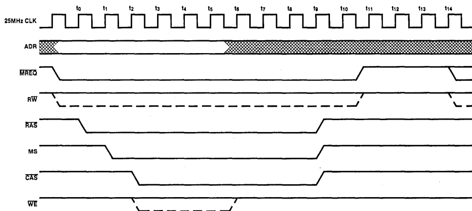
Figure 3-203. Extended Memory Cycle
