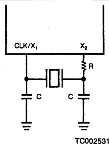
Figure 3. Fundamental Oscillator
