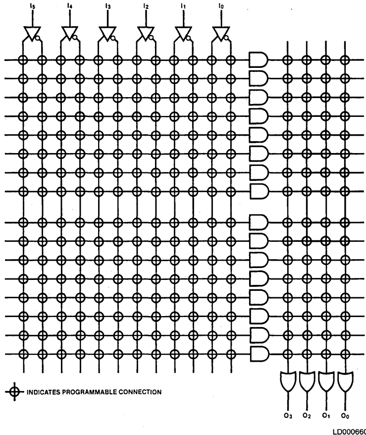
Figure 1-14. PLA Array Architecture
