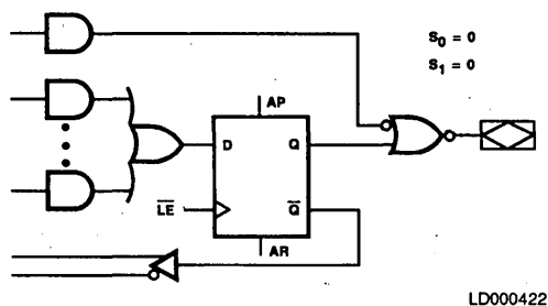
Figure 3-1. Registered/Active-LOW
