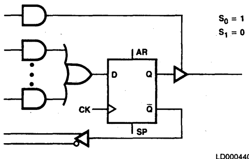
Figure 3-2. Registered/Active HIGH
