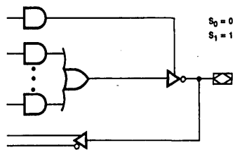
Combinatorial/Active LOW
