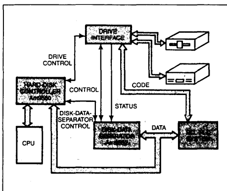
Fig 1—A complete disk controller requires only two VLSI ICs, a PLD-based encoding/decoding system, and a drive interface. The hard-disk controller and the disk-data separator provide generic disk-drive control, and the PLDs provide RLL 2,7 encoding and decoding, which increases disk storage capacity.
