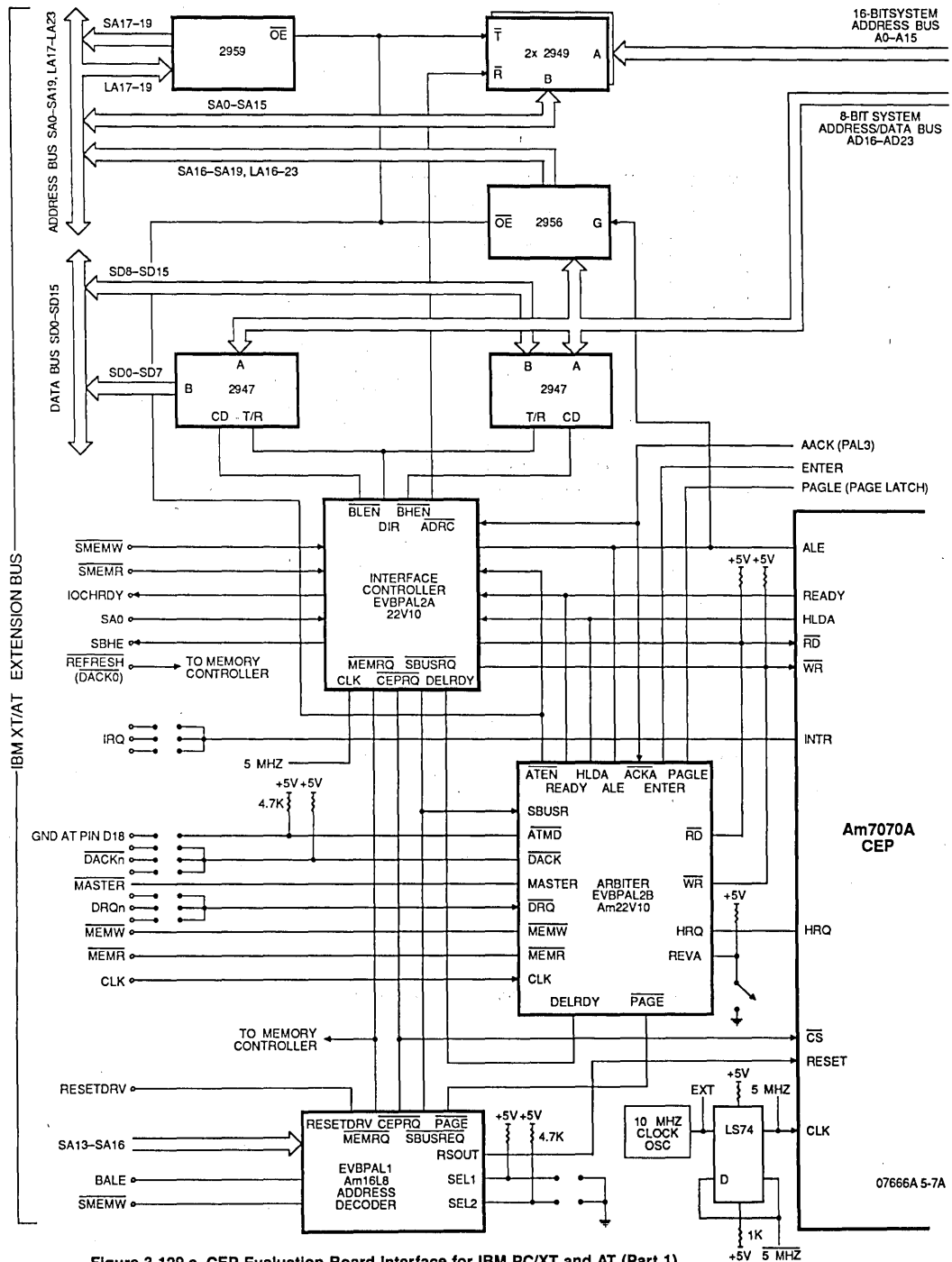
Figure 3-129.a CEP Evaluation Board Interface for IBM PC/XT and AT (Part 1)
