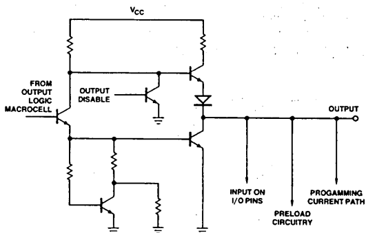
Output Circuitry
