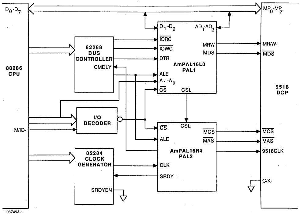
Figure 3-68. Am9518—IAPX286 Interface
