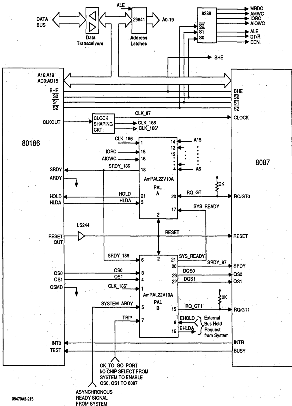
Figure 3-215. 80186 to 8087 Interface
