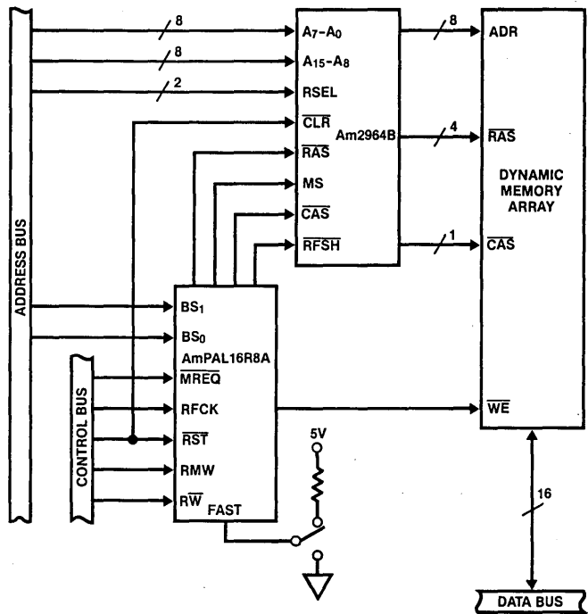
Figure 3-201. Dynamic Memory Controller 03862A-86
