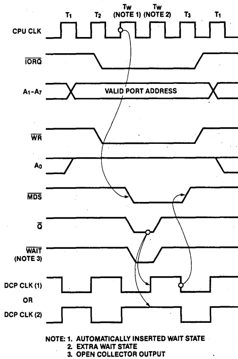
Figure 3-138. Data Write Cycle (Mode B)
