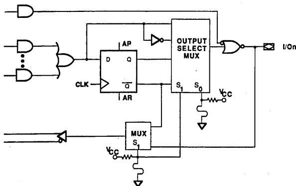
Figure 2. AmpPAL10H20EV8/AMPAL10020EV8 Output Logic Macrocell
