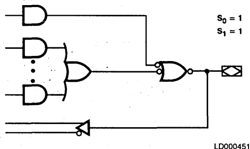
Figure 3-4. Combinatorial/Active-HIGH
