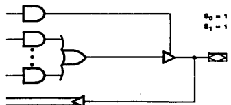
Combinatorial/Active HIGH
