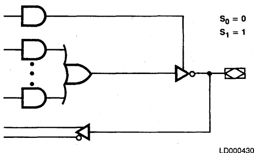
Figure 3-3. Combinatorial/Active LOW
