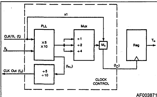
Figure 2. Clock Options
