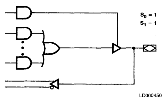
Figure 3-4. Combinatorial/Active HIGH
