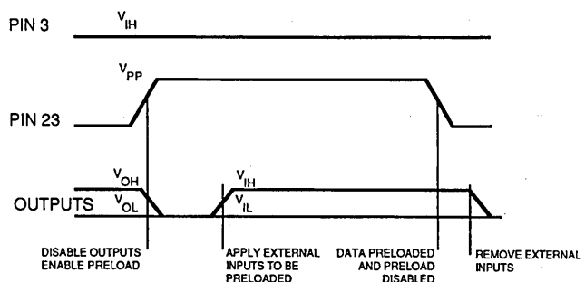
PRELOAD Timing Waveform
