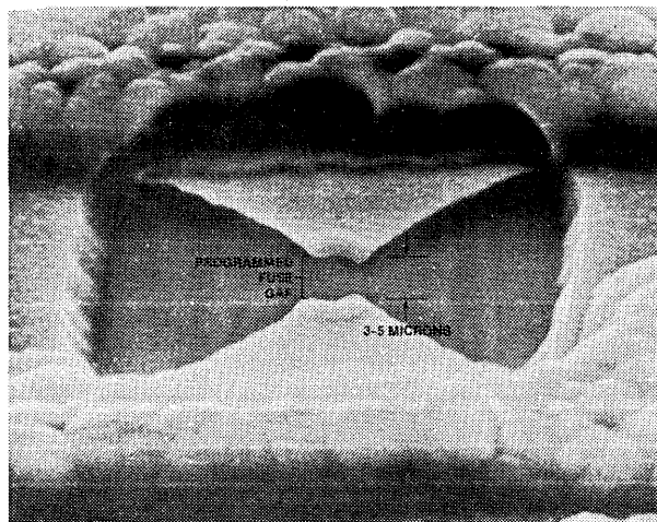
Programmed Fuse
