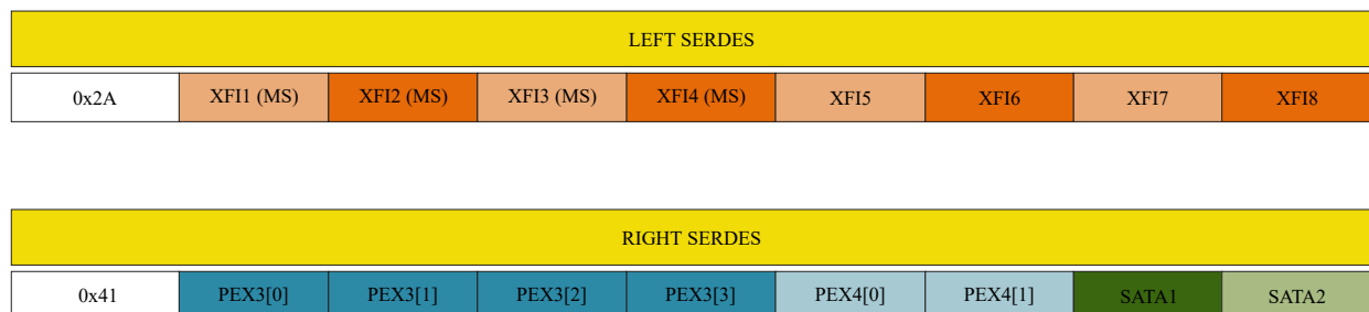
Figure 148. SERDES
