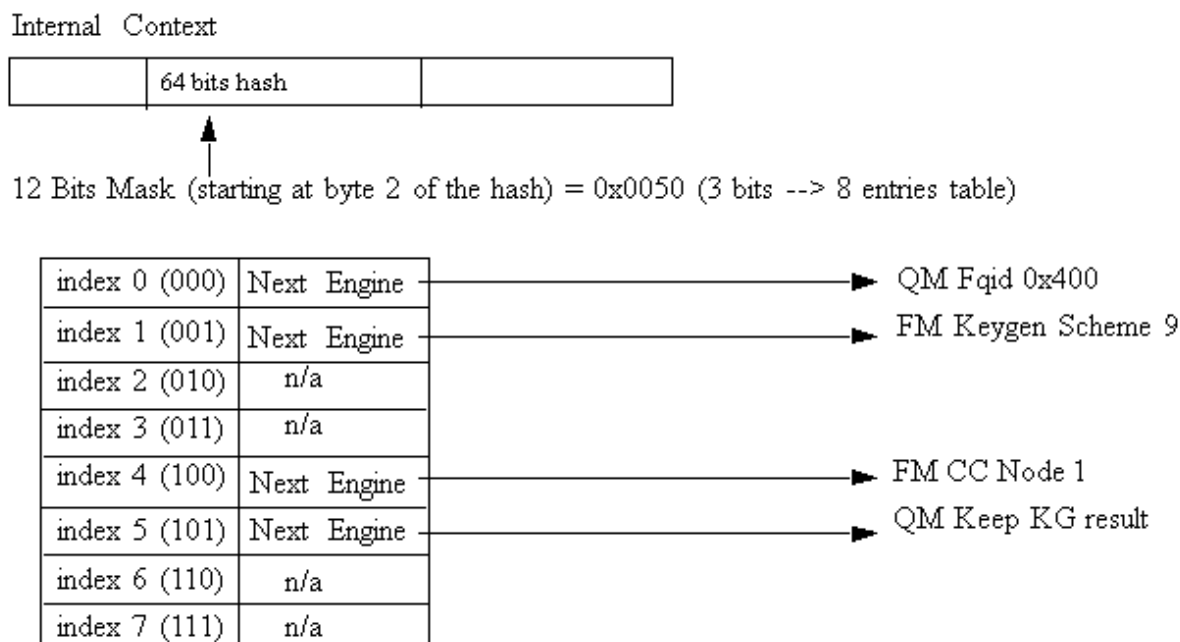
Figure 105. Indexed-Lookup node example
