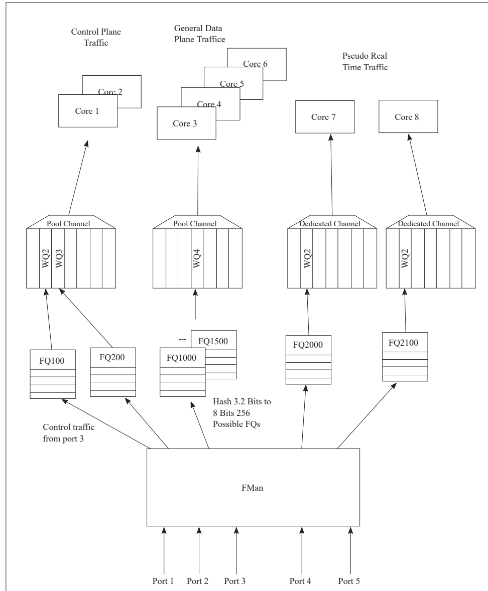
Figure 75. Ingress application map
