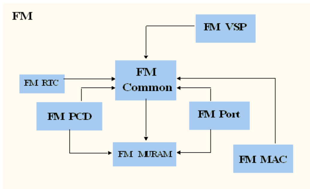
Figure 92. FMan Driver Modules (from a partition point of view)
