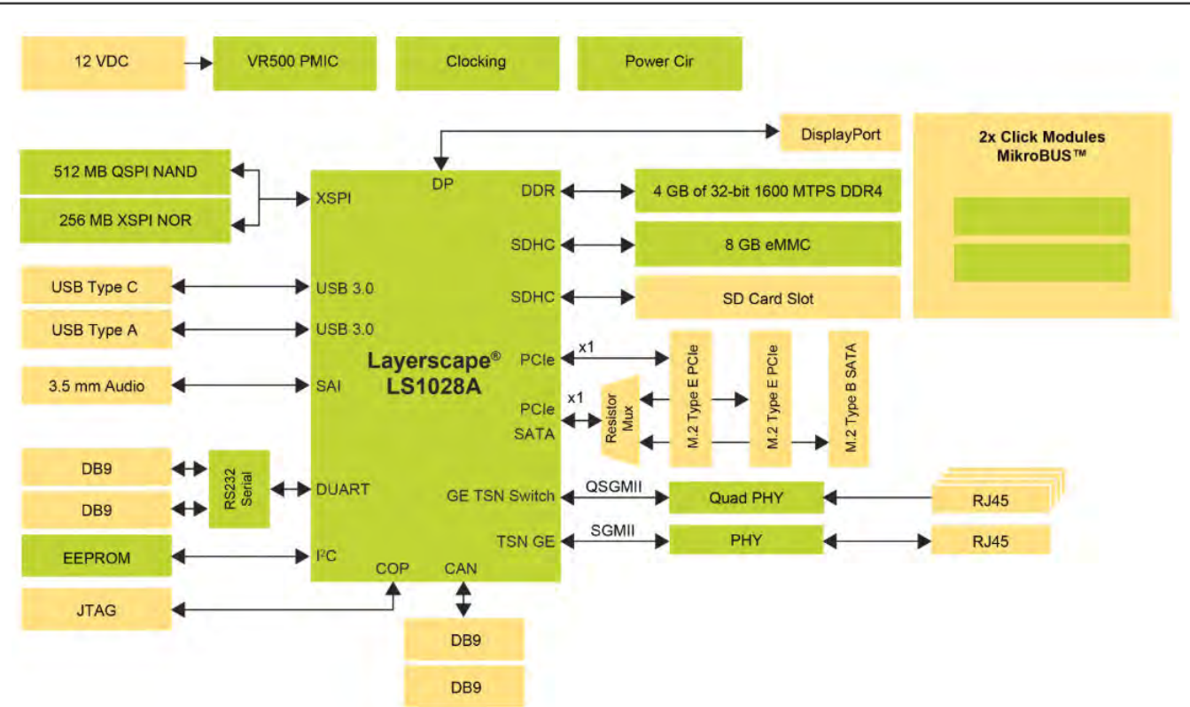
Figure 220. LS1028A architecture
