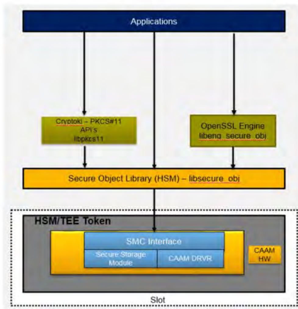
Figure 28. Block Diagram
