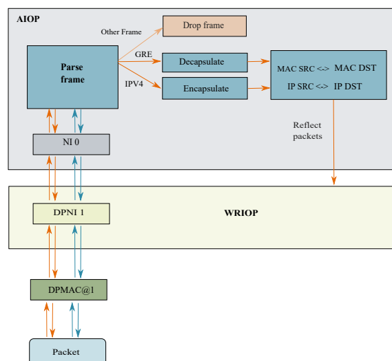
Figure 161. AIOP Header Manipulation overview
