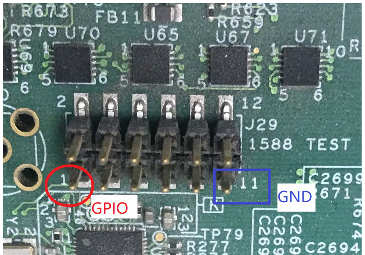
Figure 44. GPIO pin on LX2160ARDB
