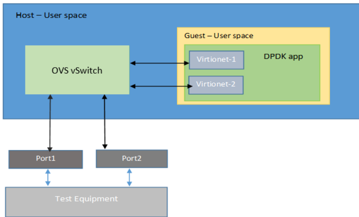
Figure 235. DPDK virtio test setup
