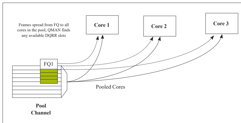
Figure 66. Avoid Blocking Scheduling
