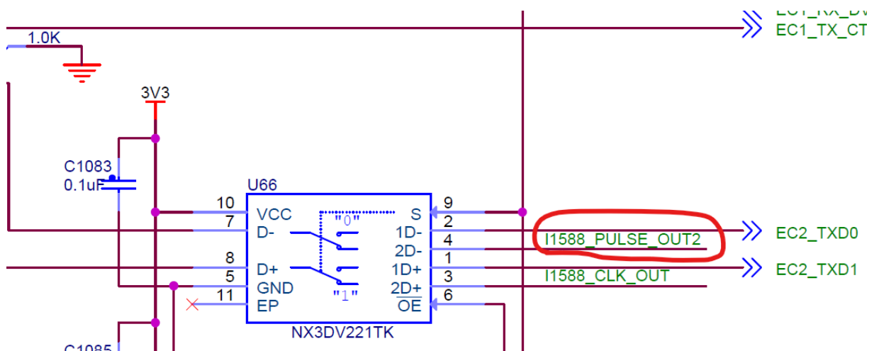
Figure 46. NX3DV221TK schematics diagram
