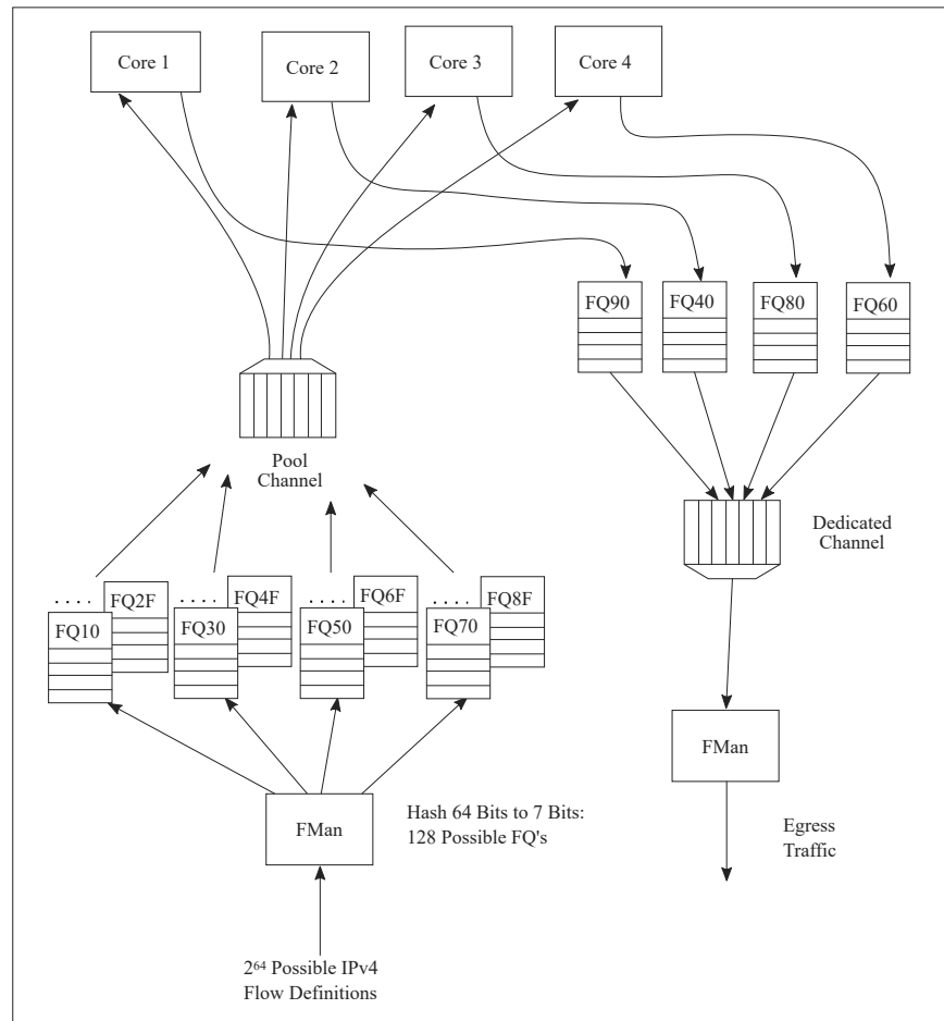
Figure 71. Using pool channel to balance processing
