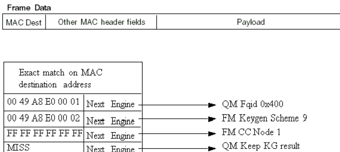
Figure 104. Exact-Match Node Example
