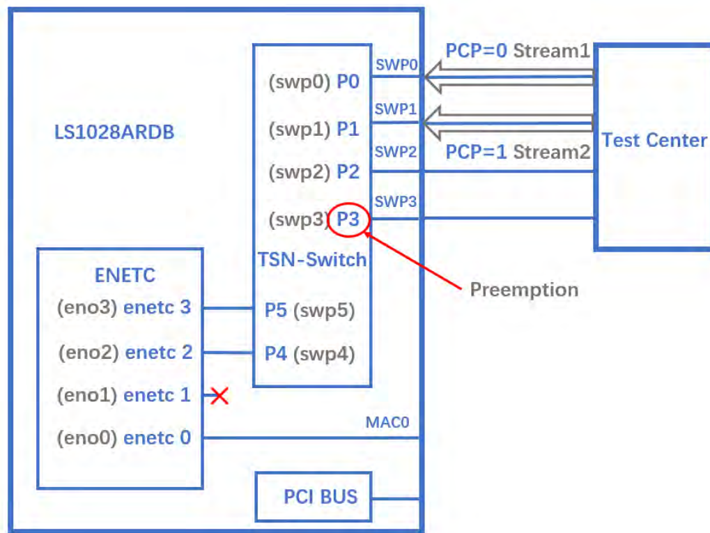
Figure 211. Qbu test on switch
