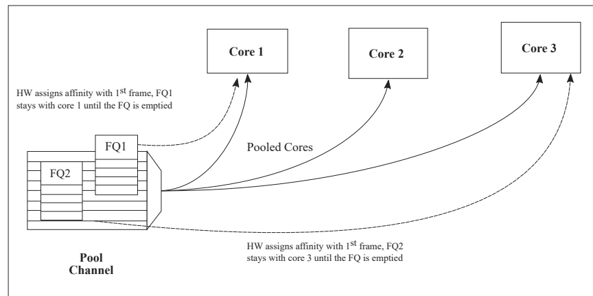
Figure 65. Hold Active Scheduling
