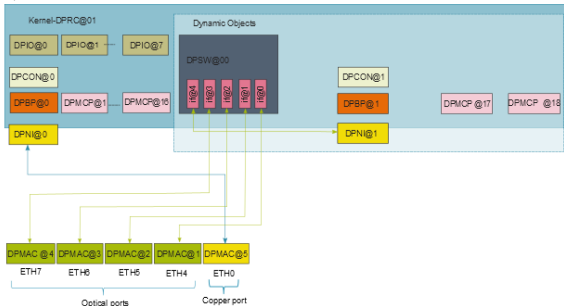
Figure 151. Dynamic DPSW demo
