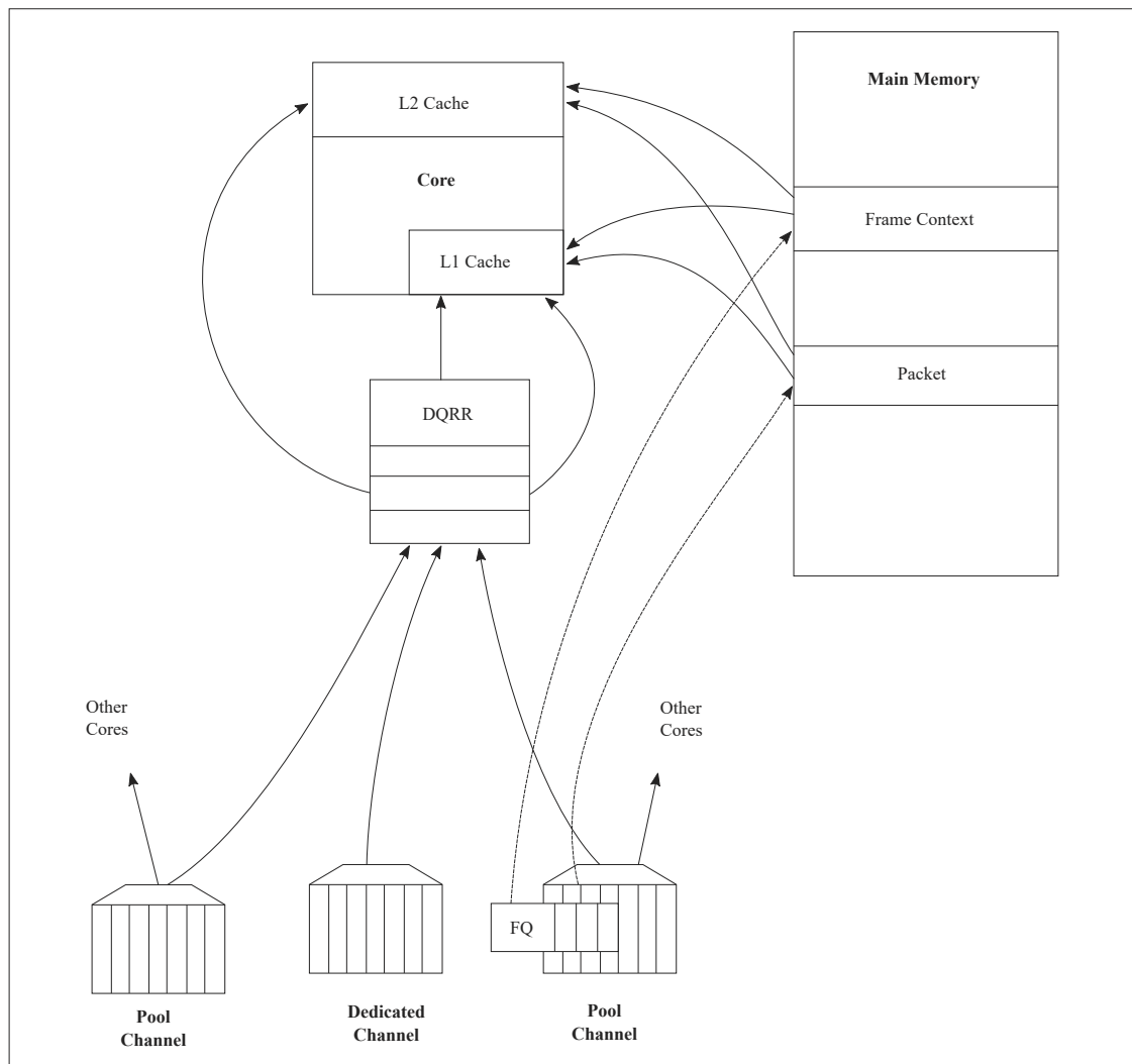
Figure 63. Cache Warming Options
