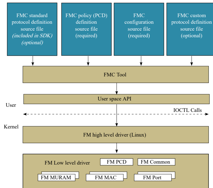
Figure 114. FMC Tool, Runtime Environment - Input XML Files / FMan Driver API Calls
