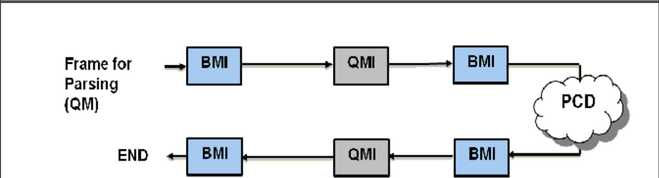
Figure 95. Default Offline Parsing Flow
