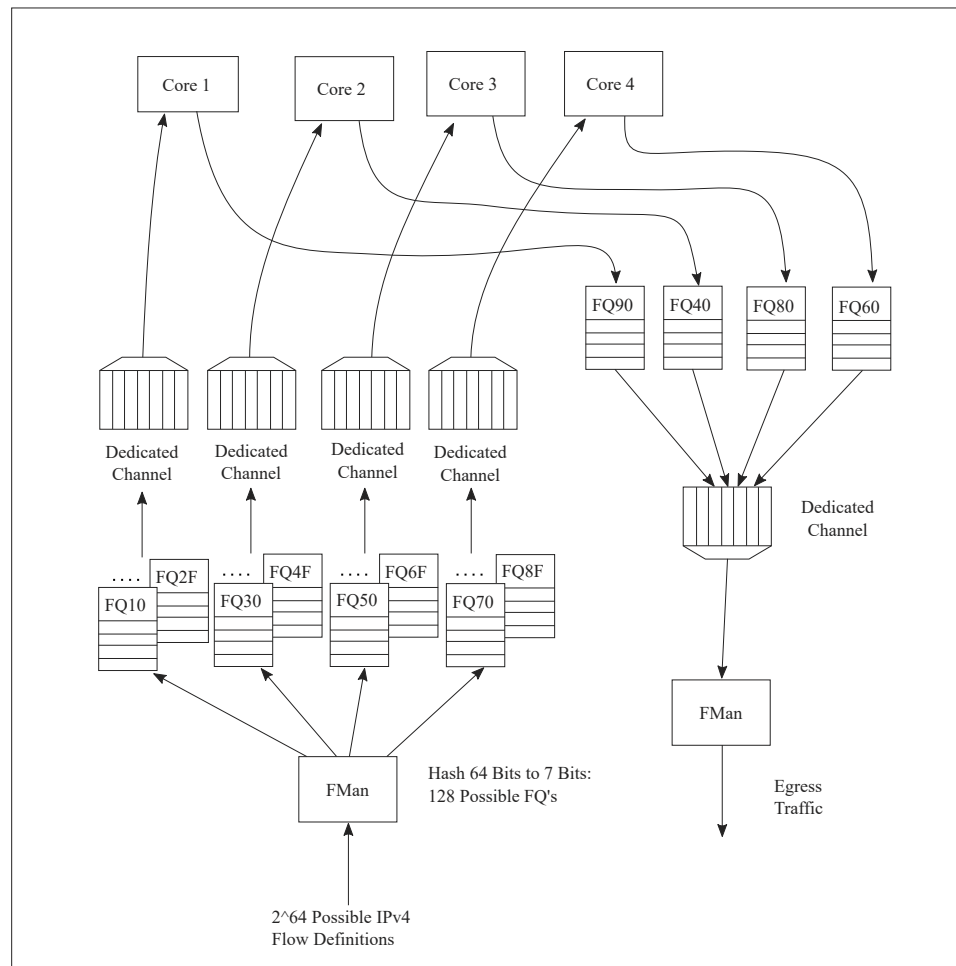
Figure 70. Using hash to assign one flow per FQ (order preserved and cache stashing effective)
