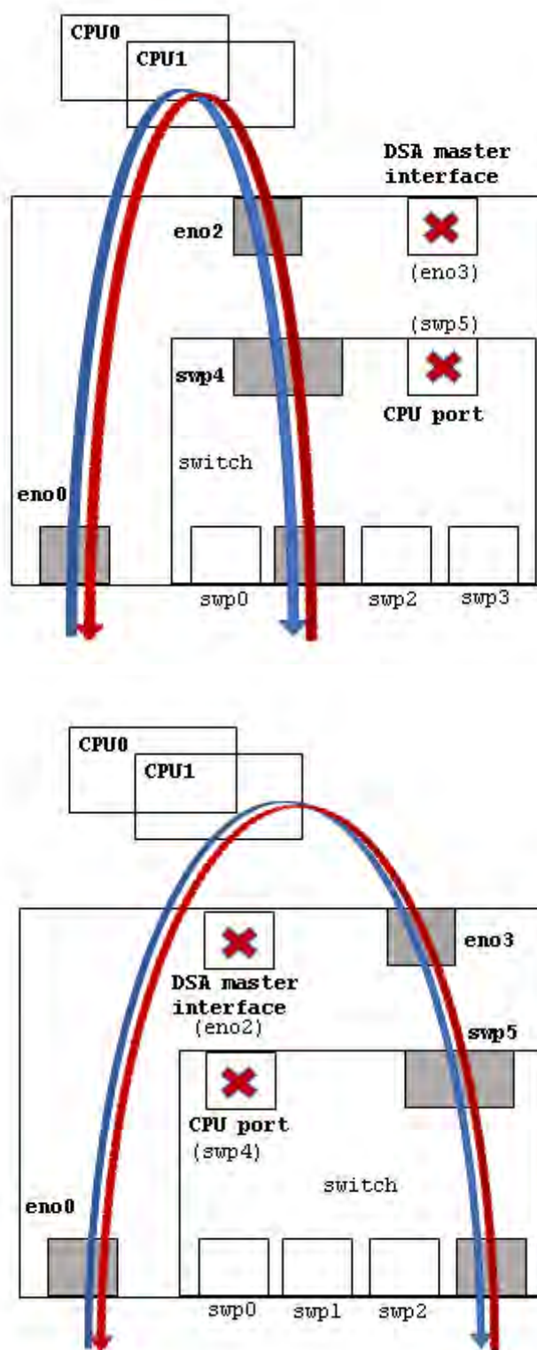
Figure 200. Packet forwarding benchmarking setups
