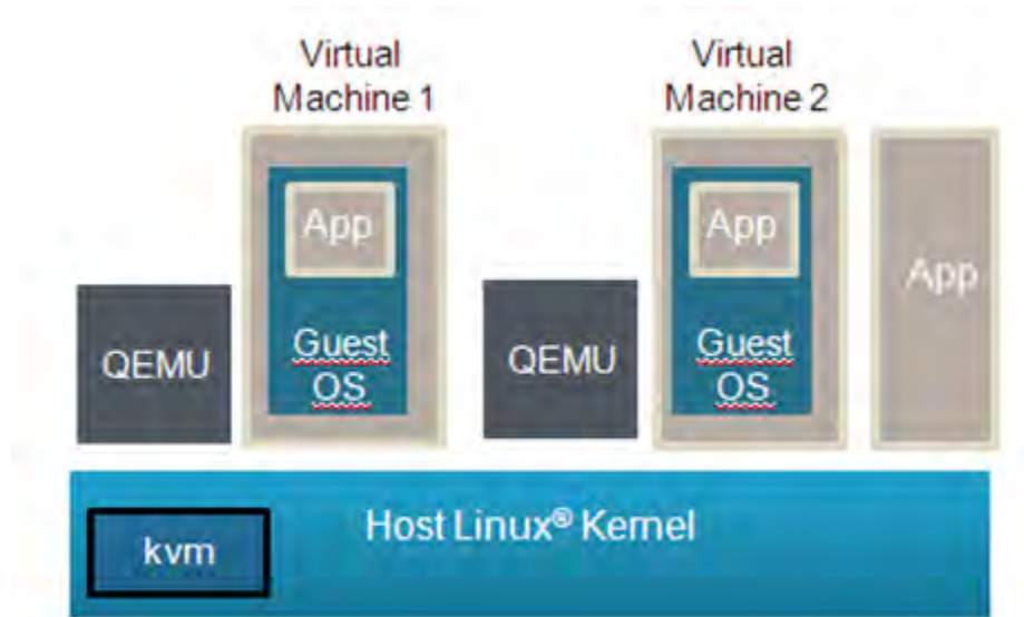
Figure 241. Kernel-based Virtual Machine
