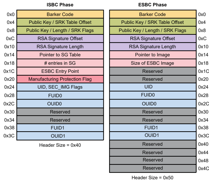
Figure 16. CSF header for LS1021A (ISBC and ESBC phase)
