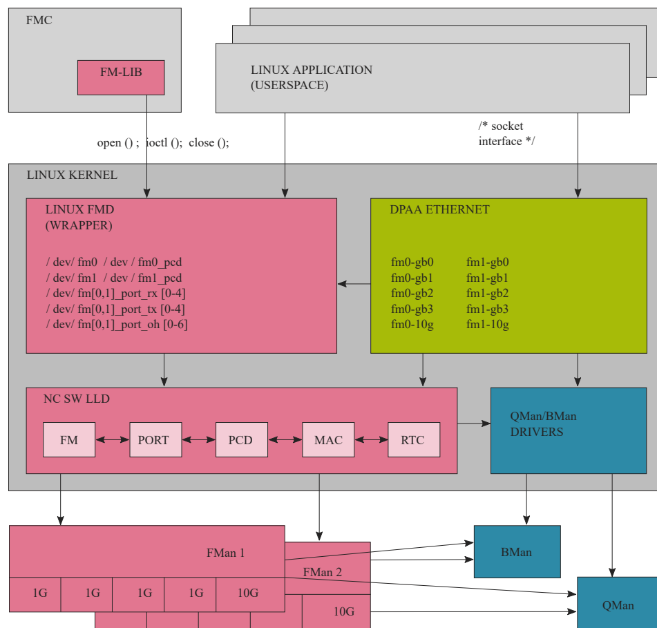
Figure 91. FMan-centric view of relationships between DPAA software and hardware blocks in the Linux environment.
