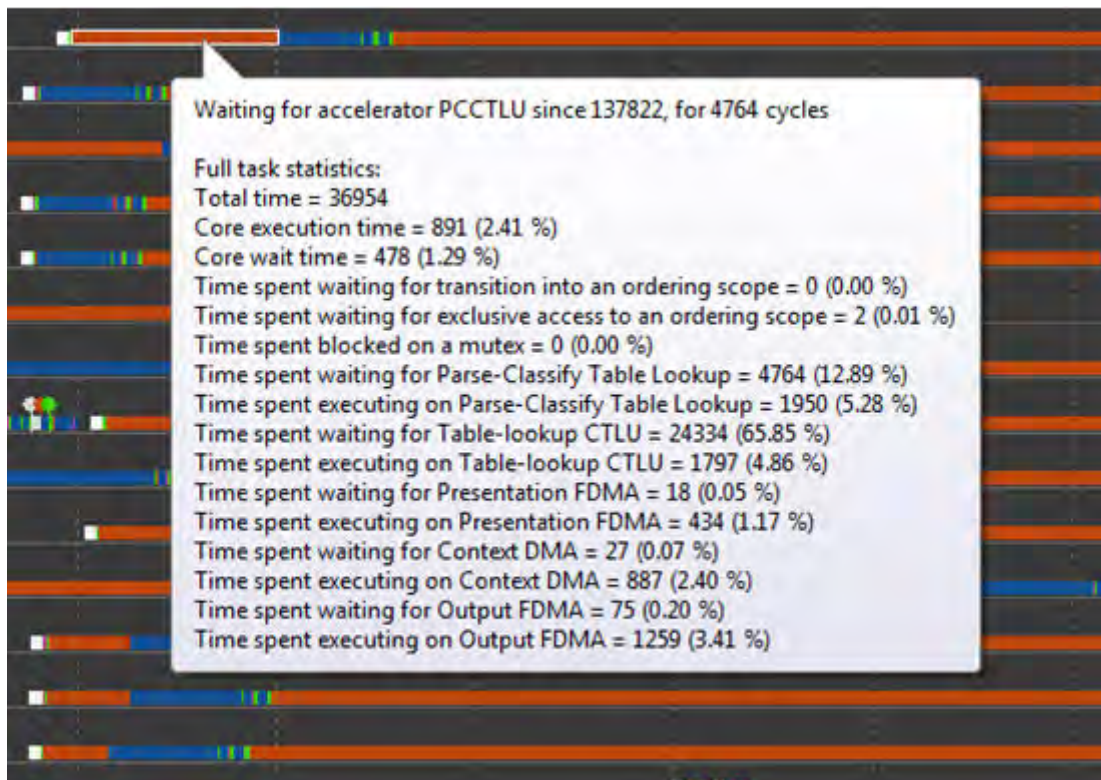
Figure 177. CTLU - Parser Bottleneck Example
