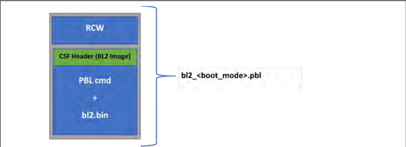
Figure 10. Secure boot bl2.pbl image (NXP CoT)
