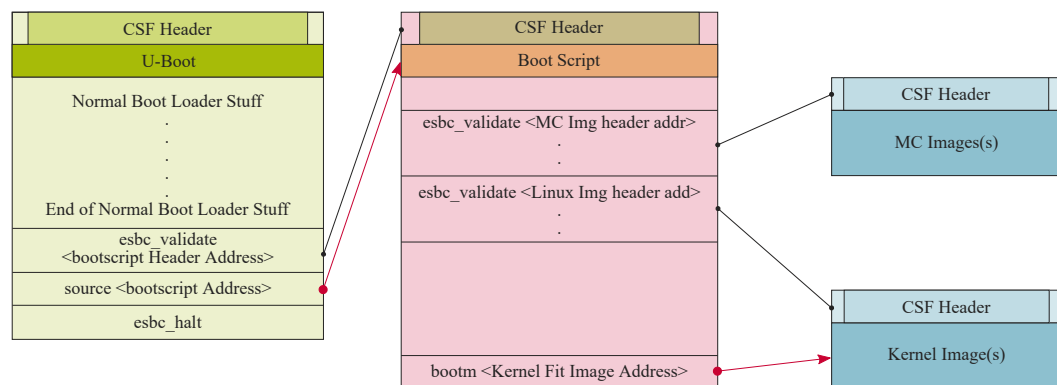
Figure 22. Secure boot flow (Chain of Trust from U-Boot)
