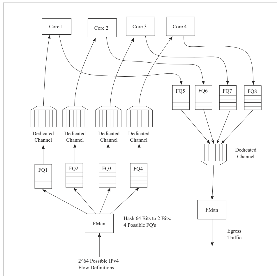
Figure 69. Simple flow distribution via hash (order preserved)
