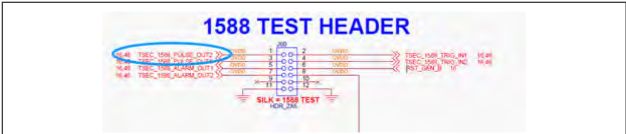
Figure 49. IEEE-1588 access header LX2160AQDS schematics diagram
