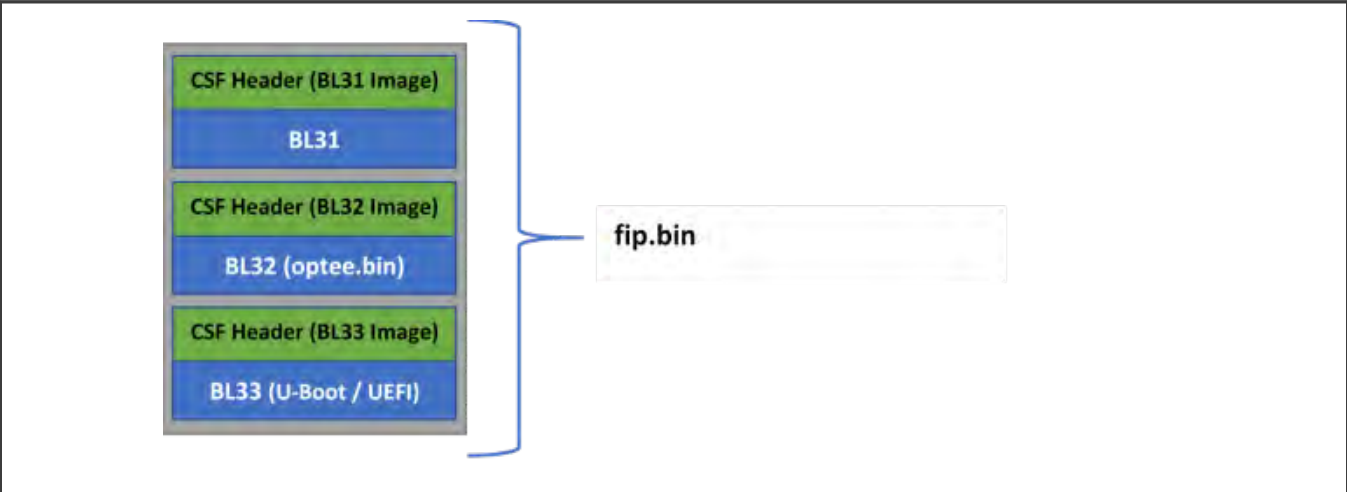
Figure 11. Secure boot fip.bin image (NXP CoT)
