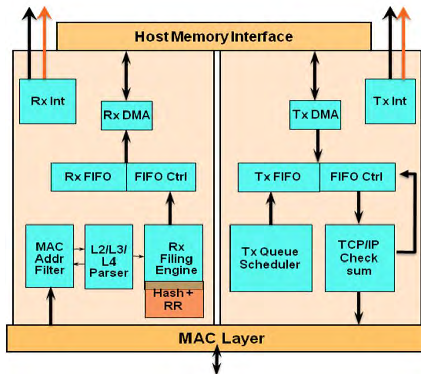
Figure 190. "Virtualized" eTSEC Block Diagram
