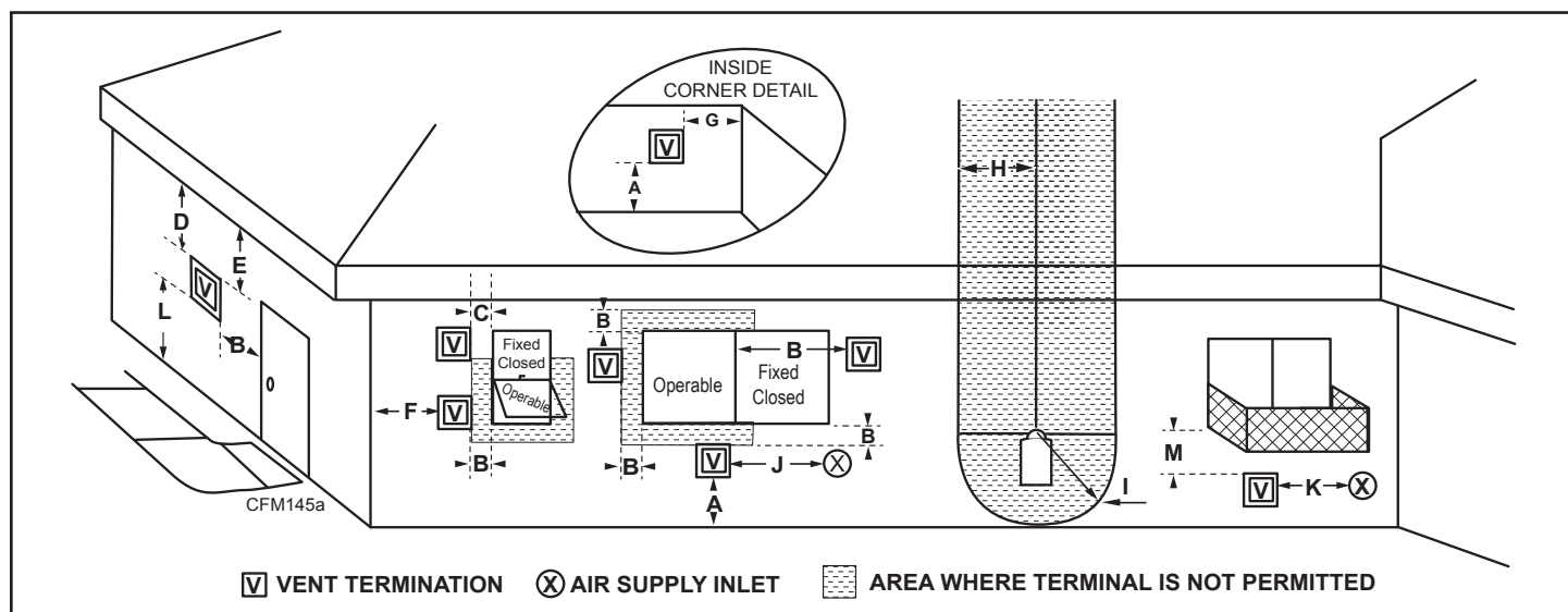
Figure 9 - Termination Locations
