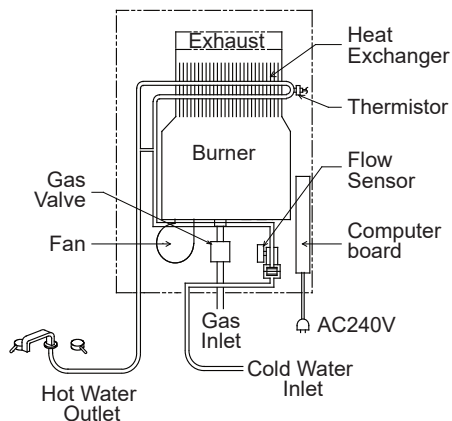
M26/M26-50 UNIT
