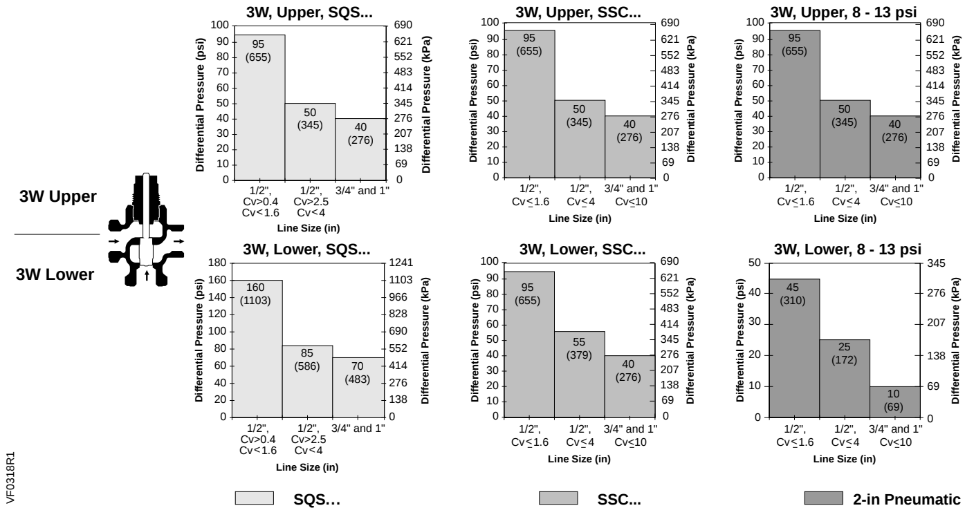
Figure 2. Close-off Pressures.
