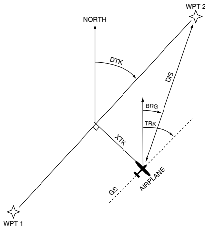
Figure 13-1 Illustrated NAV Terms
