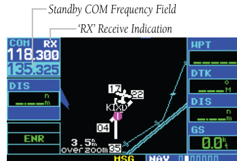
Figure 2-1 'RX' Receive Indication
