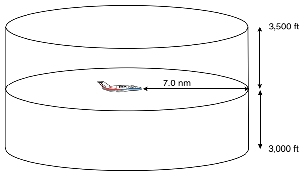
Figure 11-1 TIS Coverage Volume
