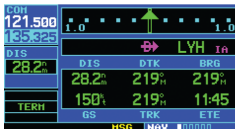
Figure 6-14 CDI Scale at 1.0 nm
