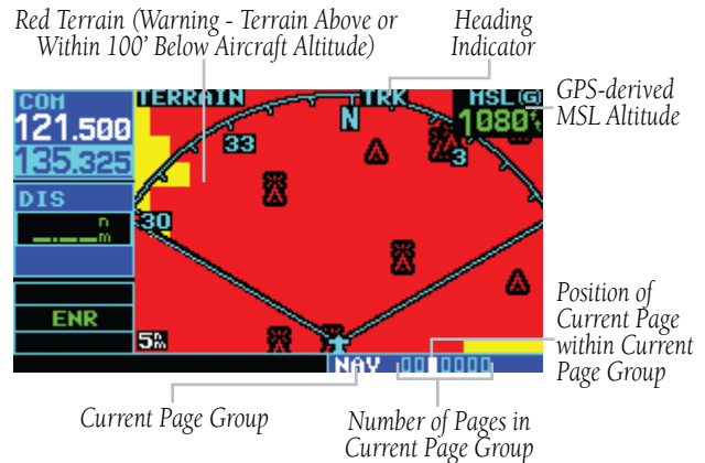
Figure 3-26 TERRAIN Page 120° View
