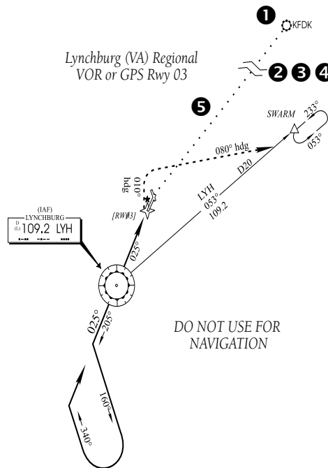
Figure 6-9 Sample Approach with Procedure Turn
