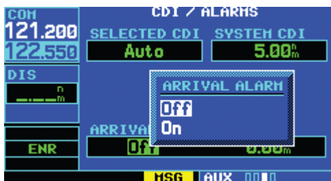
Figure 9-60 Arrival Alarm Window
