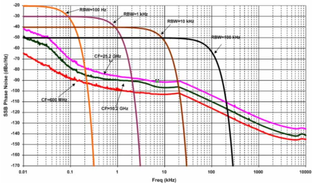
Nominal Phase Noise at Different Center Frequencies with RBW Selectivity Curves, Optimized Phase Noise, Versus Offset Frequency
