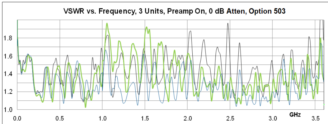
Nominal VSWR – Preamp On, Freq Option \leq 526 [Plot]
