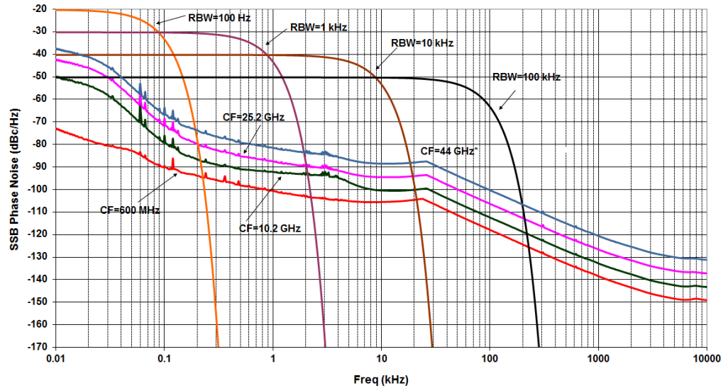
Nominal Phase Noise at Different Center Frequencies with RBW Selectivity Curves, Optimized Phase Noise, Versus Offset Frequency
