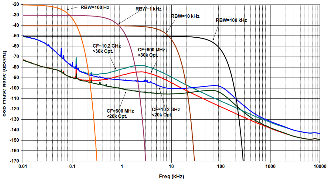
Nominal Phase Noise at Different Phase Noise Optimization with RBW Selectivity Curves, CF = 600 MHz and 10.2 GHz, Versus Offset Frequency
