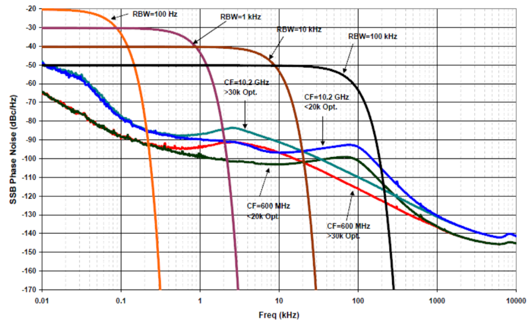
Nominal Phase Noise at Different Phase Noise Optimization with RBW Selectivity Curves, CF = 600 MHz and 10.2 GHz, Versus Offset Frequency
