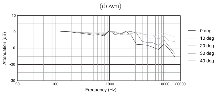
Vertical Off-Axis Frequency Response:
