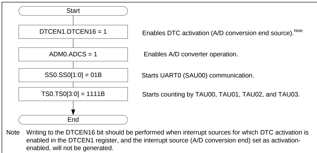
Figure 3.9 Procedure for Enabling Peripheral Functions (DTC (High-Speed Transfer) Transfer Start)
