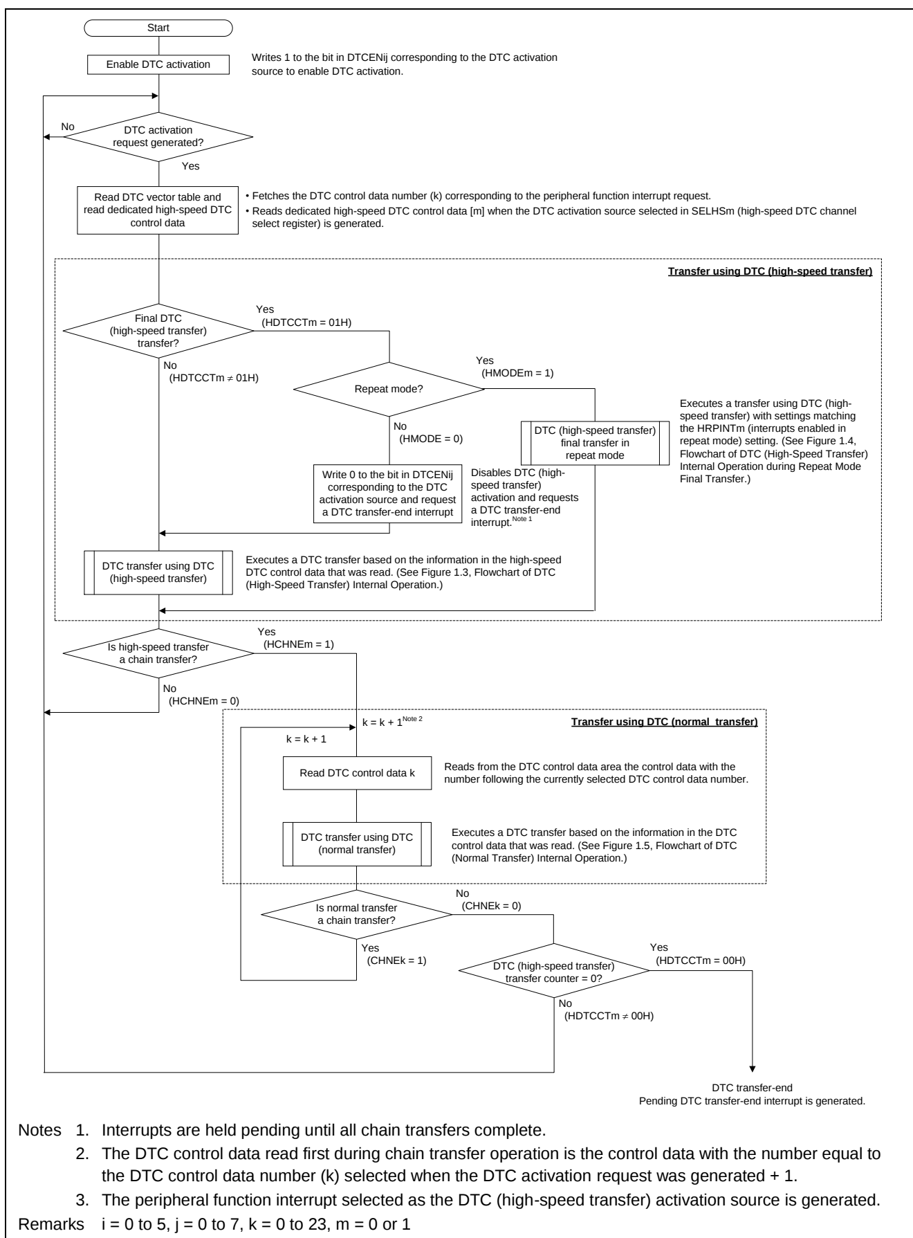
Figure 1.2 Flowchart of DTC (High-Speed Transfer and Chain Transfer) Internal Operation
