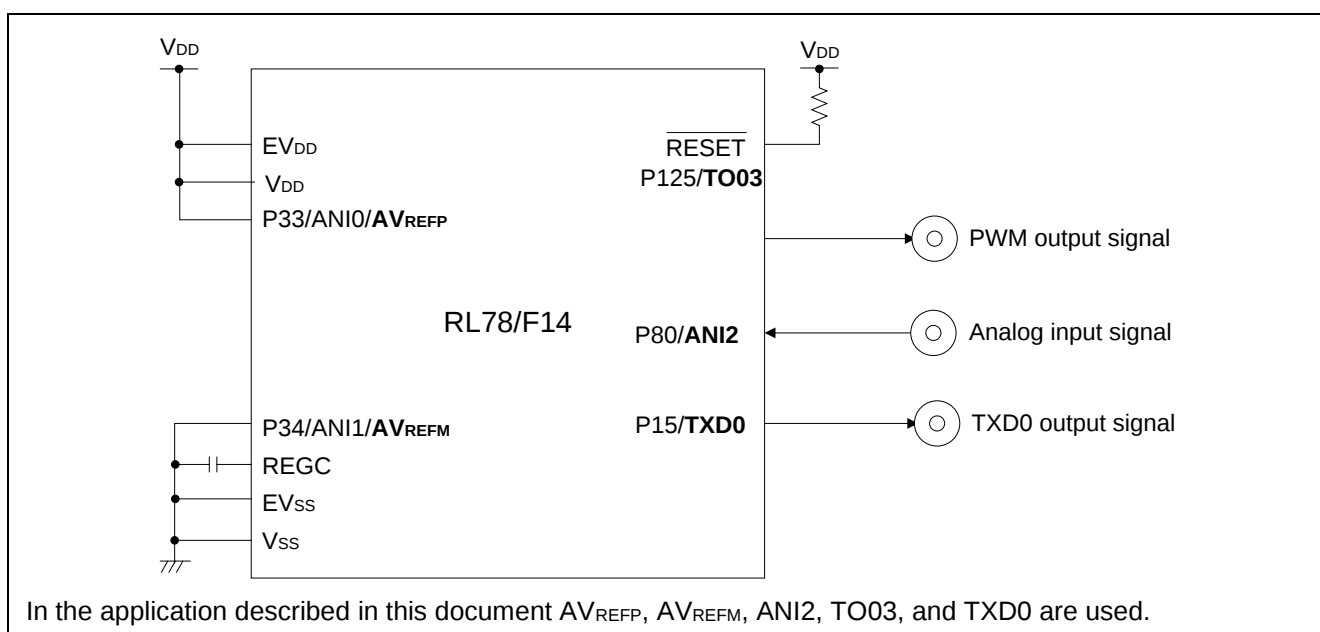
Figure 2.1 Connection Diagram of Pins Used
