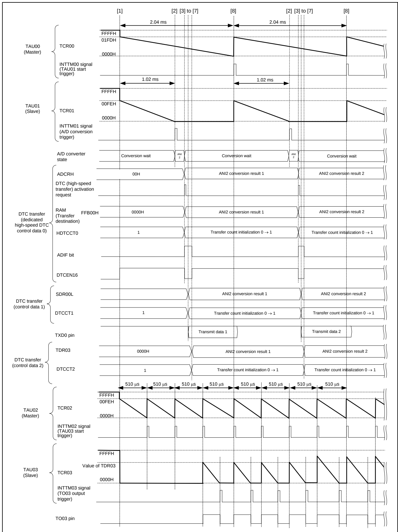
Figure 2.4 DTC Transfer Timing (1/2)
