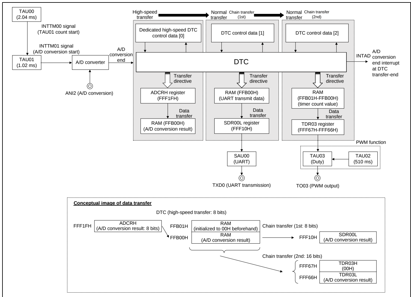
Figure 2.2 Configuration Diagram of Peripheral Functions Used
