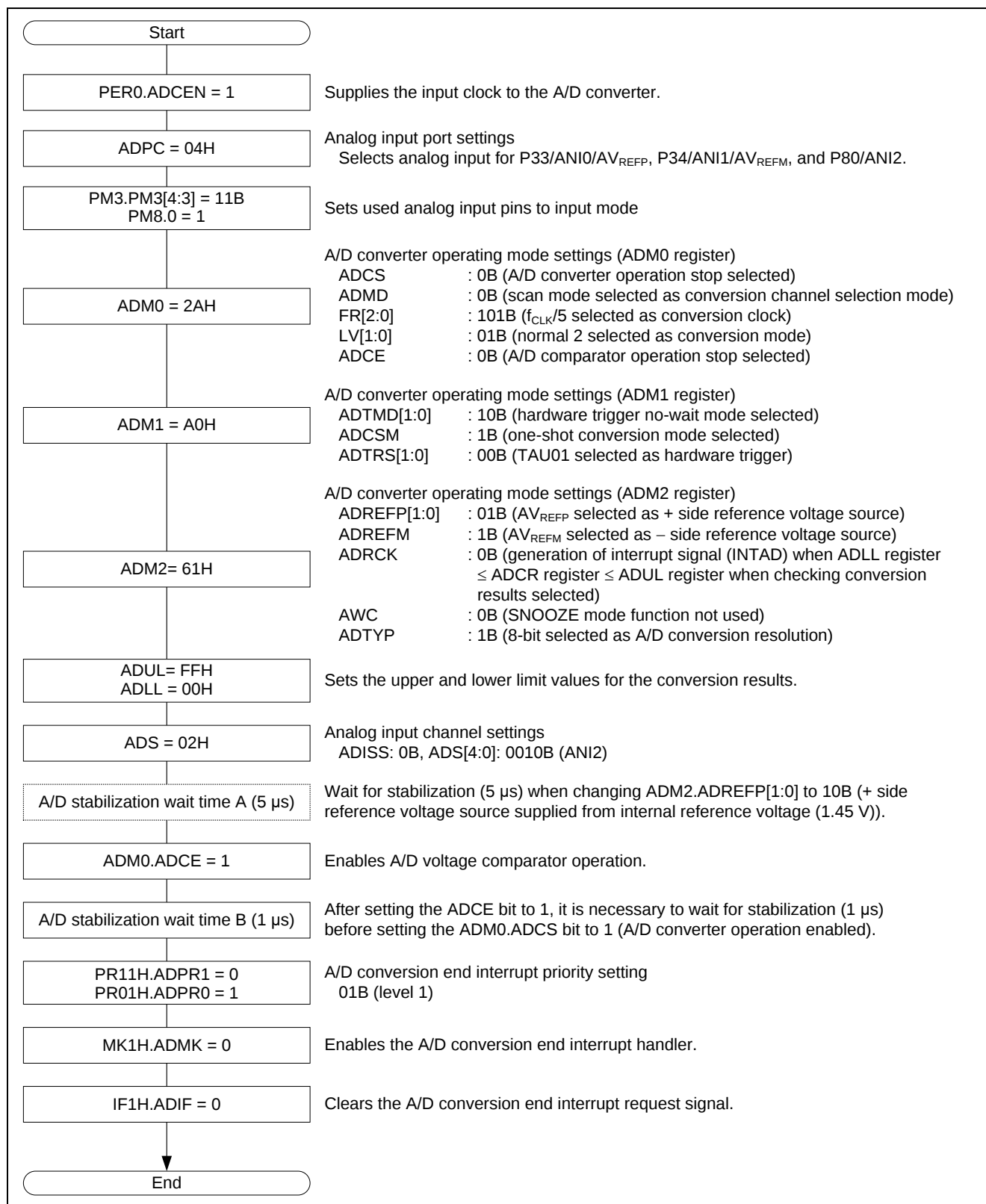
Figure 3.5 A/D Converter Initialization Procedure
