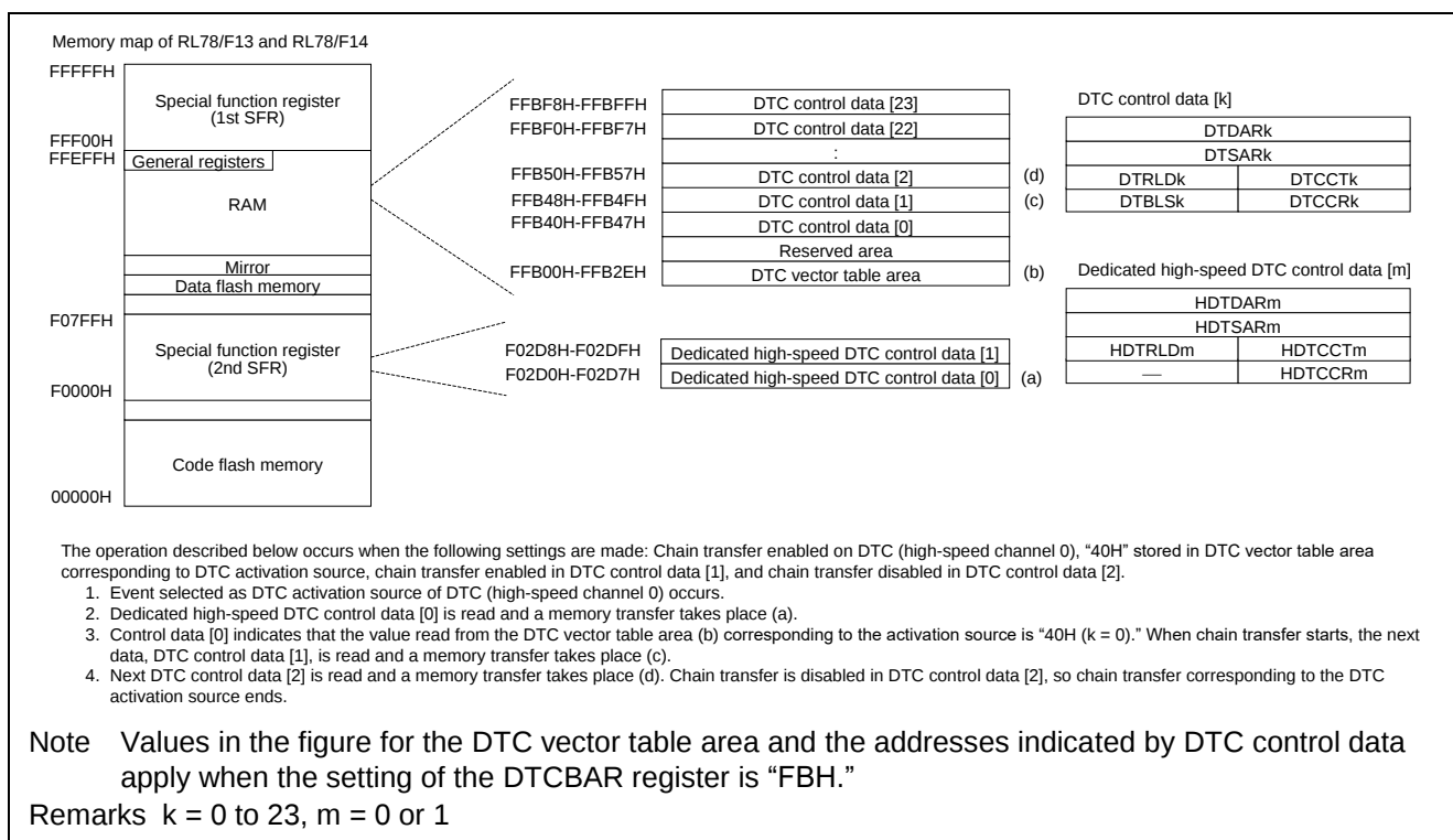
Figure 1.1 Flowchart (Outline) of DTC (High-Speed Transfer and Chain Transfer) Operation
