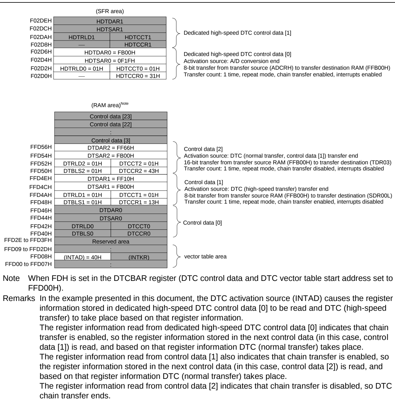
Figure 3.4 Allocation of DTC Control Data
