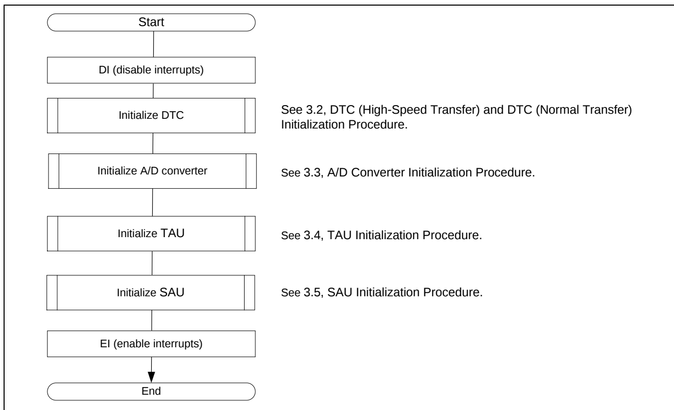
Figure 3.1 Peripheral Function Initialization Procedure
