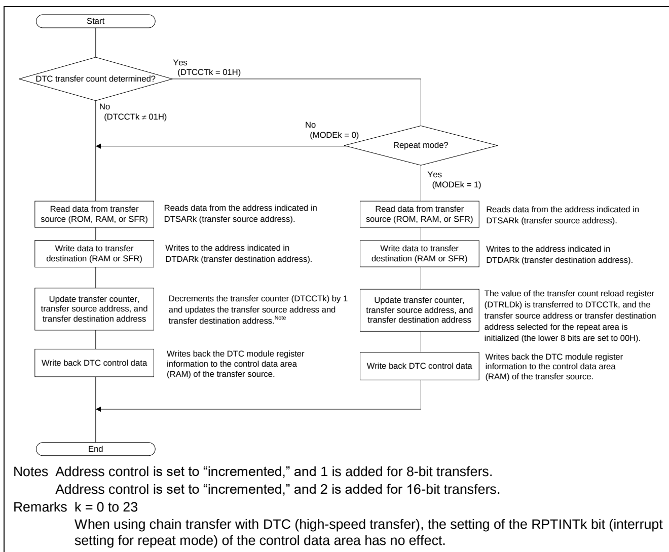
Figure 1.5 Flowchart of DTC (Normal Transfer) Internal Operation
