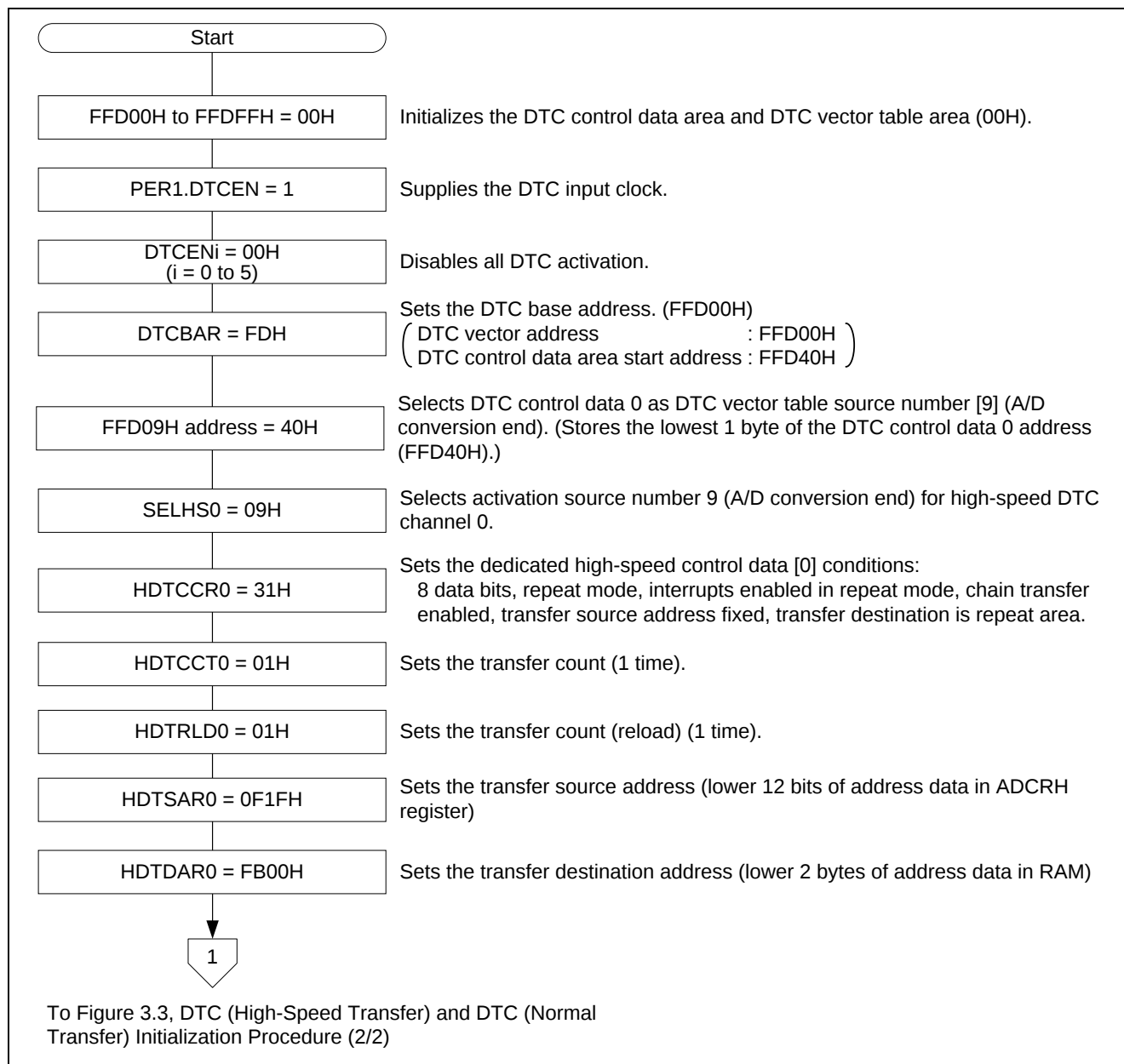
Figure 3.2 DTC (High-Speed Transfer) and DTC (Normal Transfer) Initialization Procedure (1/2)
