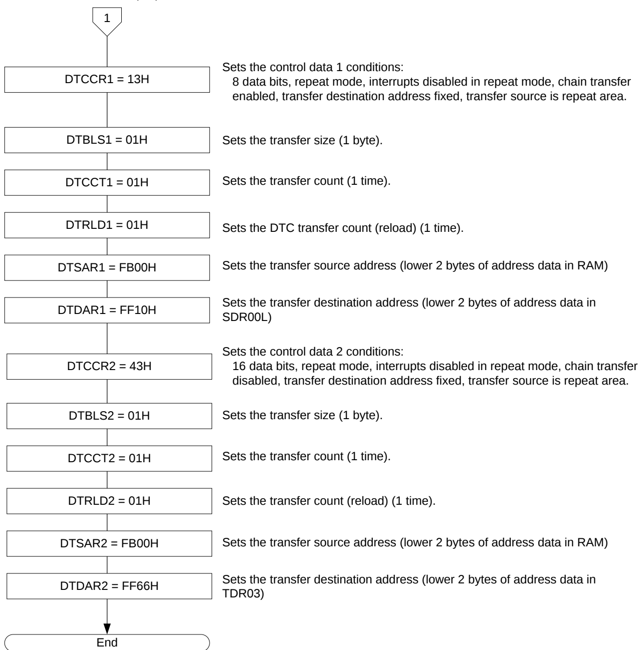
Figure 3.3 DTC (High-Speed Transfer) and DTC (Normal Transfer) Initialization Procedure (2/2)
