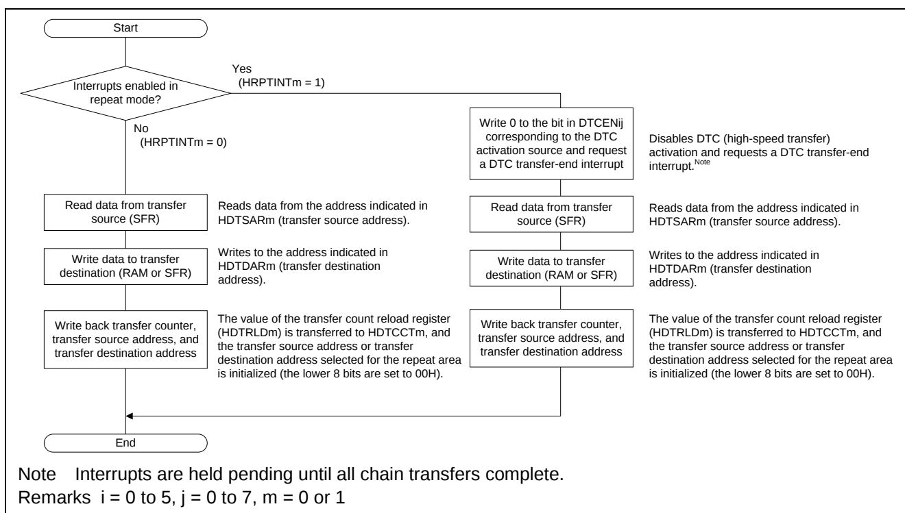
Figure 1.4 Flowchart of DTC (High-Speed Transfer) Internal Operation during Repeat Mode Final Transfer
