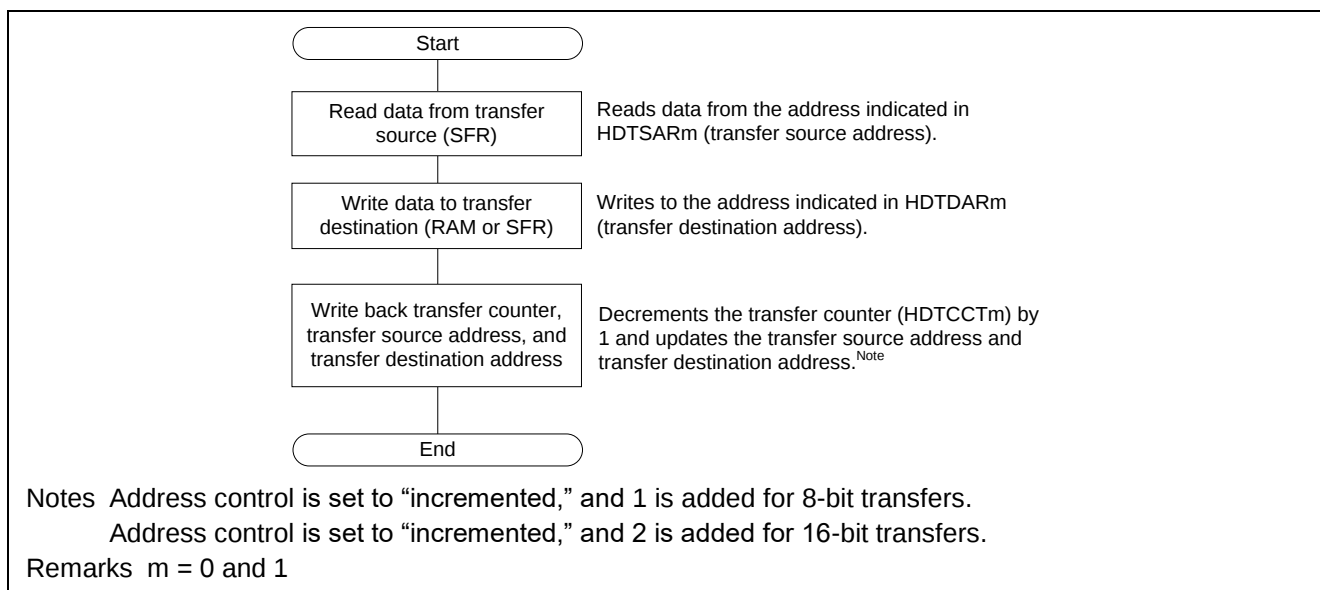
Figure 1.3 Flowchart of DTC (High-Speed Transfer) Internal Operation
