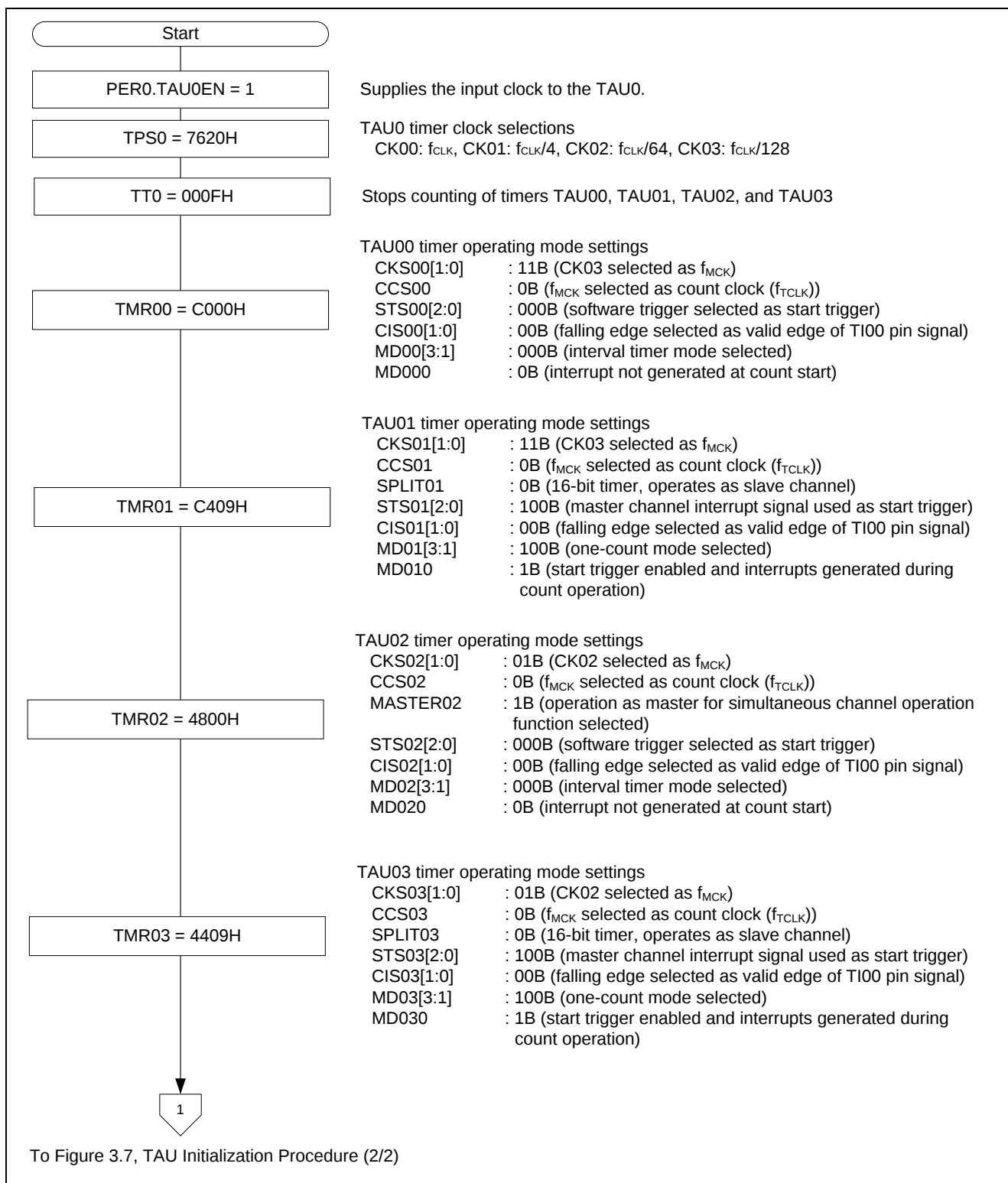
Figure 3.6 TAU Initialization Procedure (1/2)
