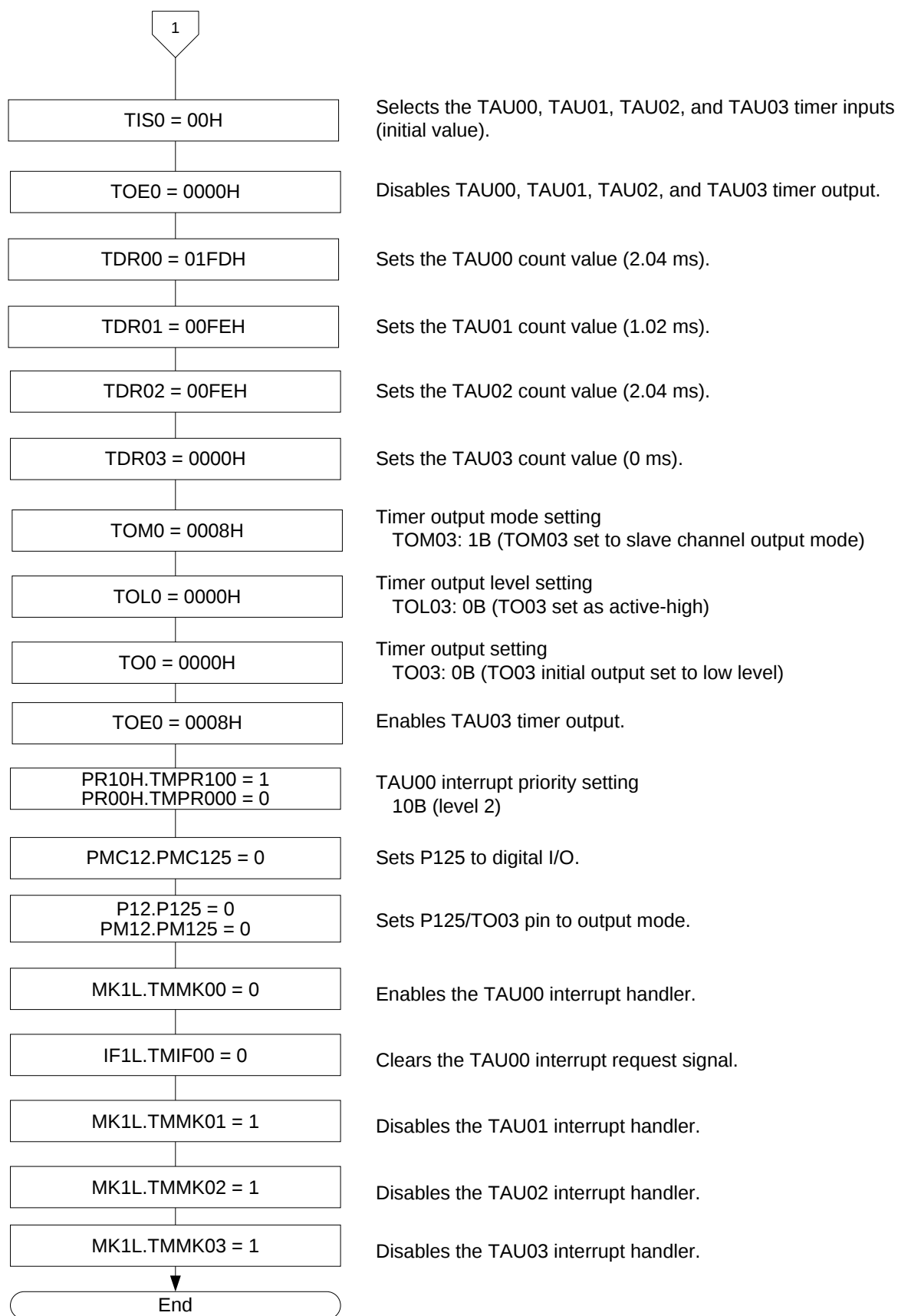
Figure 3.7 TAU Initialization Procedure (2/2)
