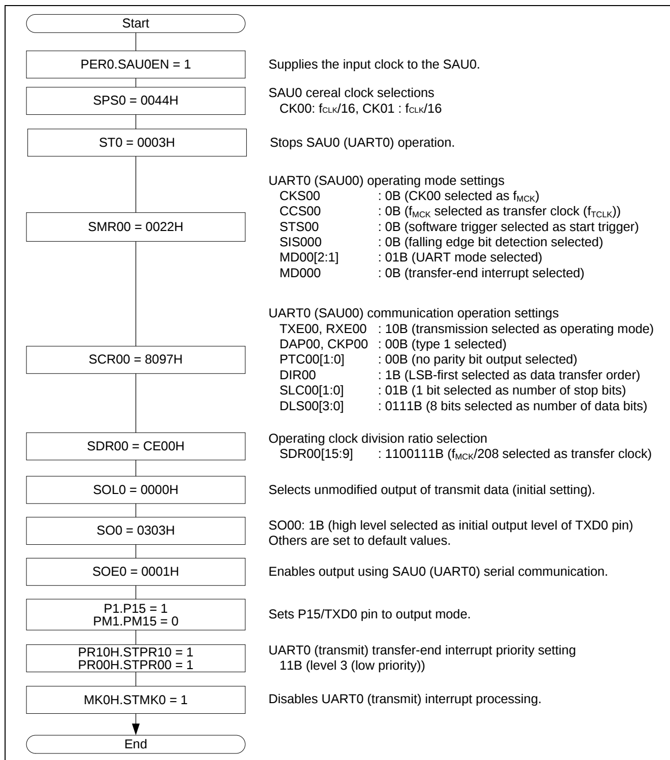
Figure 3.8 SAU Initialization Procedure
