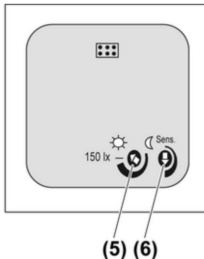
4: Adjusters on the rear
