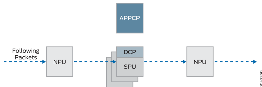
Figure 5: Fast-Path Processing
