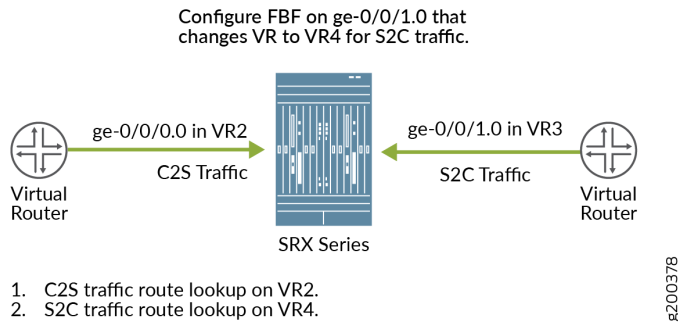
Figure 30: Reverse Route Enabled with FBF
