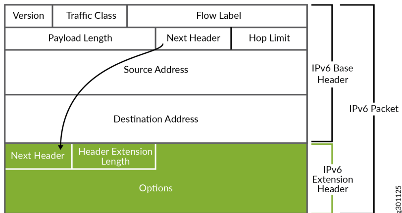
Figure 20: IPv6 Extension Header
