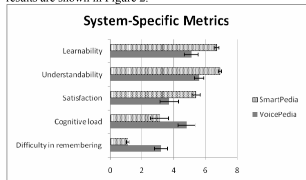
Fig 2: User ratings for VoicePedia and SmartPedia. Error bars indicate standard error. All differences were statistically significant ( p < .05 ).
