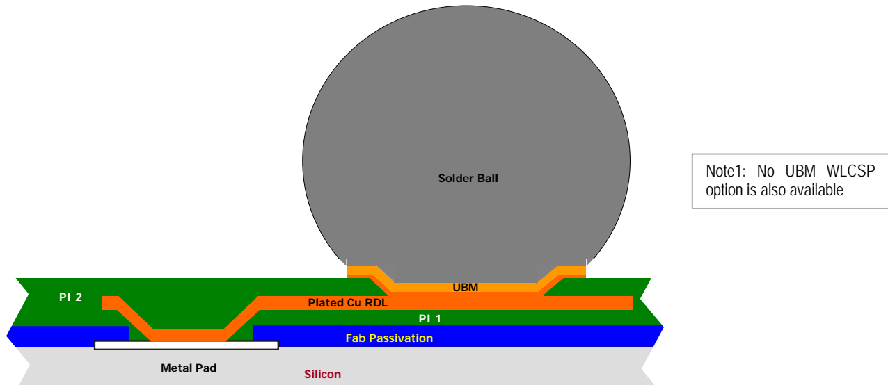
Figure 2. Cross section schematic of IDT WLCSP Package with RDL
