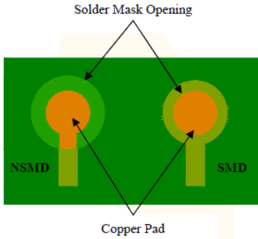
Figure 3. SMD vs. NSMD Copper Pads
