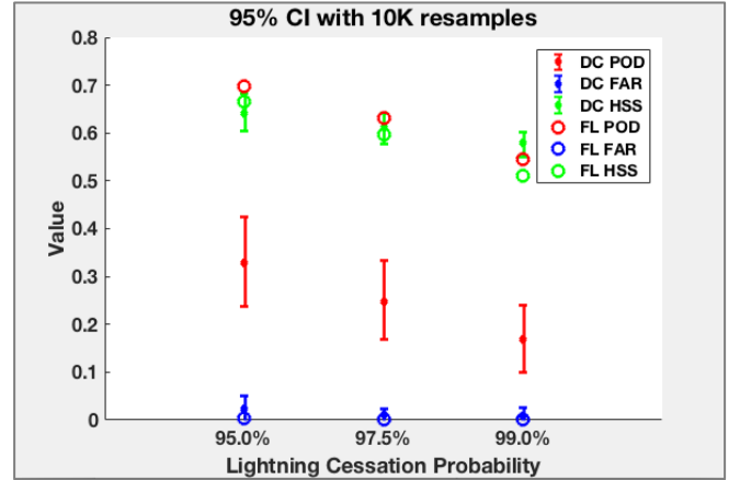
Fig. 6. POD, FAR, and HSS performance statistics for Patton's GLM in Washington, D.C. and central Florida. Washington, D.C. performance statistics and bootstrapped results utilizing the 95th percentile are depicted by the diamonds and error bars, respectively. Central Florida performance statistics are overlaid in circles.
