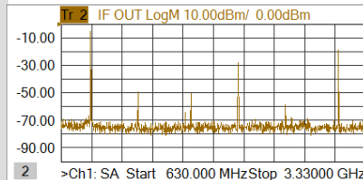
Output spectrum on IF port
