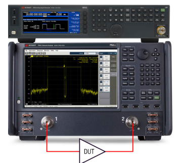
Classic NPR measurement with PNA-L and UXG
