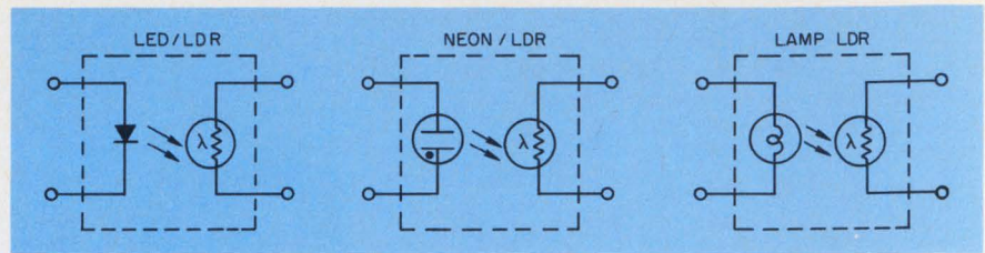
2. Photo-isolators with photoresistor (LDR) outputs use light sources of visible LEDs, neon lamps and tungsten lamps. The bidirectionality of the LDR units makes them useful in applications using ac voltages.
