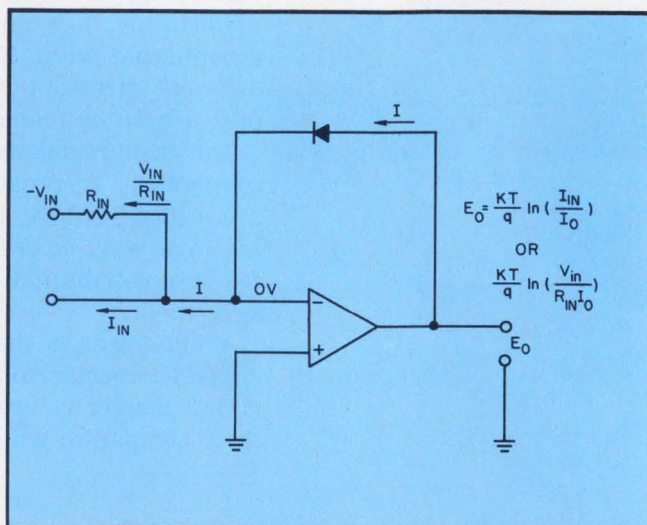
1. The ideal diode log circuit delivers an output voltage proportional to the log of the input current divided by a reference current.
