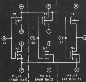
CA3600E schematic diagram
