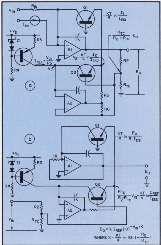
11. By using a controlled current reference, the temperature-compensated log circuit performs ratio calculations referred to I_{REF} (a). When some of the leads are reconnected as shown here the log circuit produces an antilog output (b).
