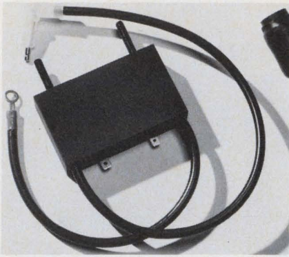
Special isolators are designed for high voltages. These units, by Sigma Instruments, are rated at 15 kV rms (left) and 1 kV (right). The 15 kV unit is a tungsten lamp/photoreistor device. The other has a LED.
