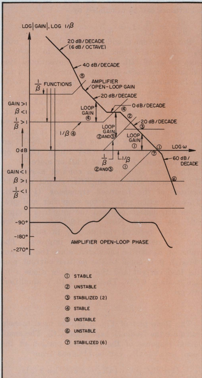
7. The Bode plot for stability analysis shows stable and unstable loop gain ( A\beta ) situations.
