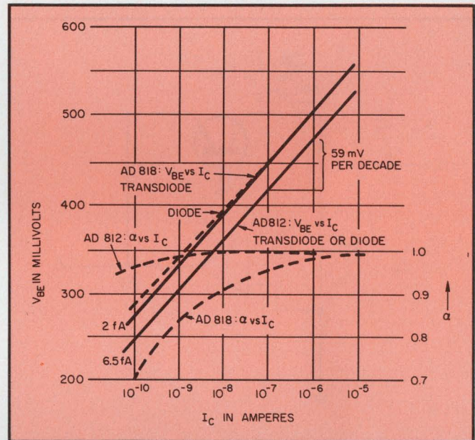
3. Some matched transistor pairs used as transdiodes and diodes are compared for \alpha vs I_C and V_{be} vs I_C .
