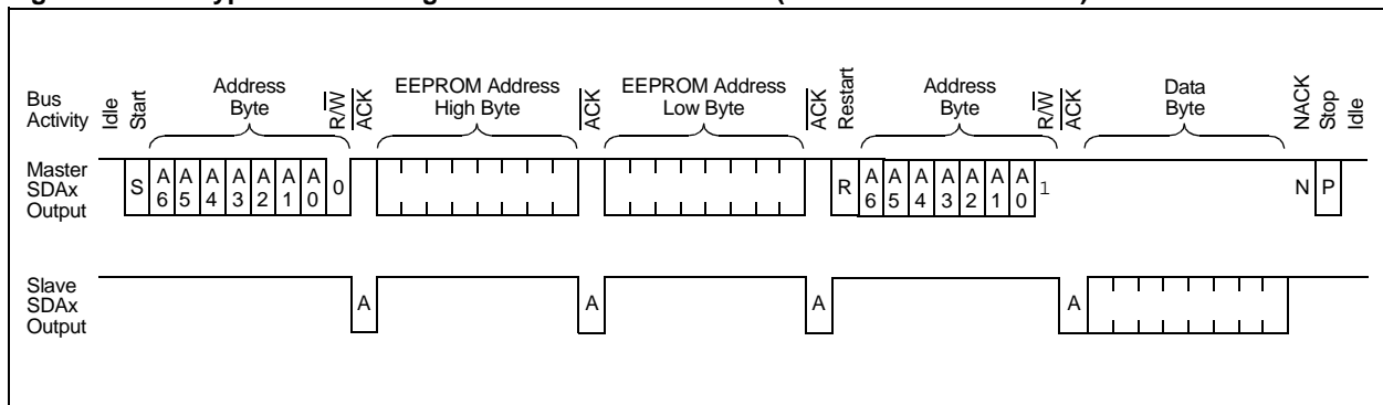
Figure 24-7: Typical I 2 C Message: Read of Serial EEPROM (Random Address Mode)
