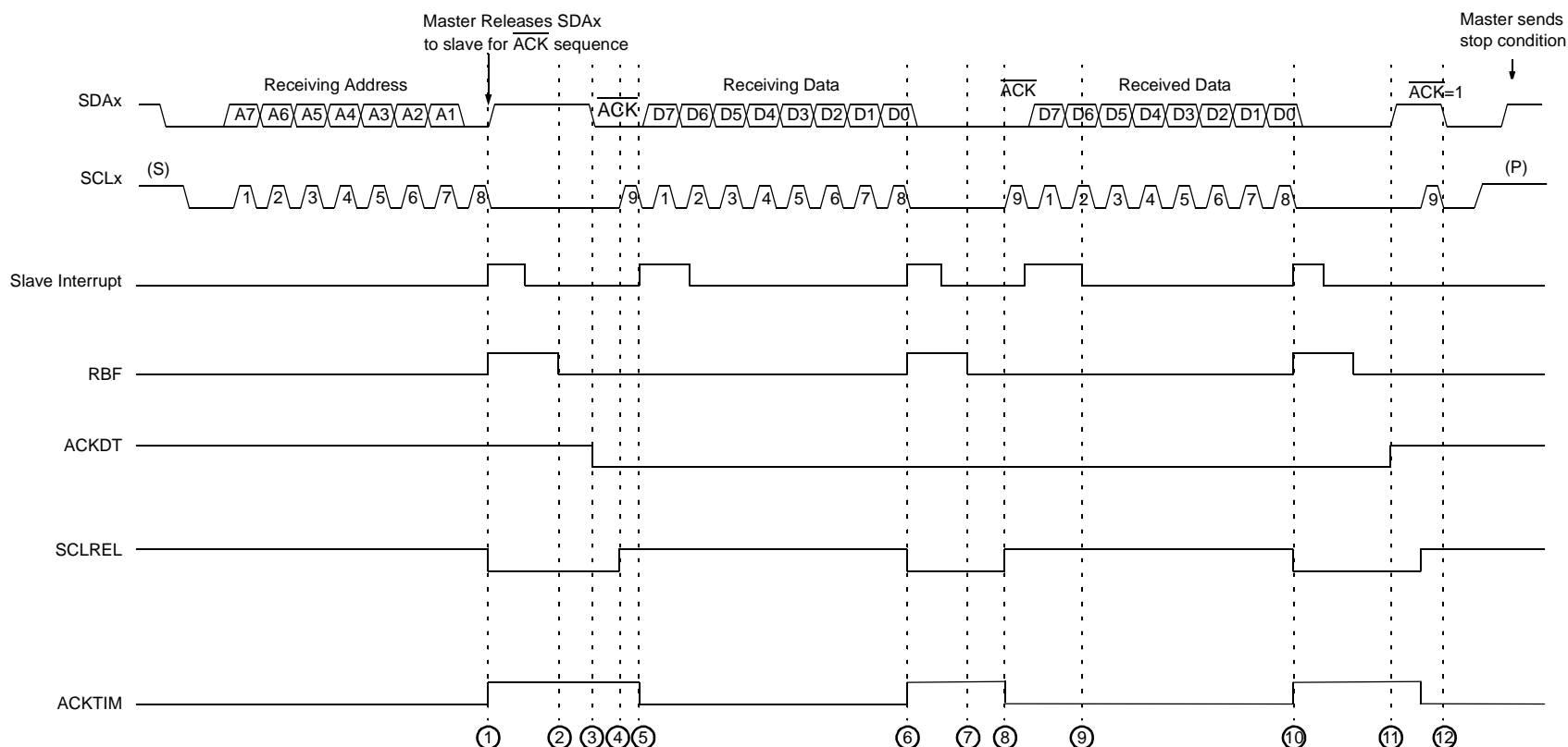
Figure 24-23: Slave Read with AHEN = 1 AND DHEN = 1
