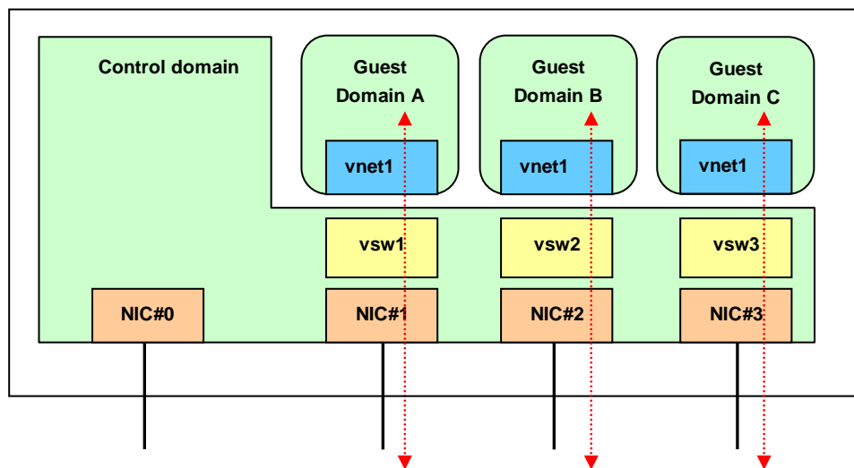
Figure 3.9 Allocation of the virtual switch (vsw) or virtual network device (vnet)
