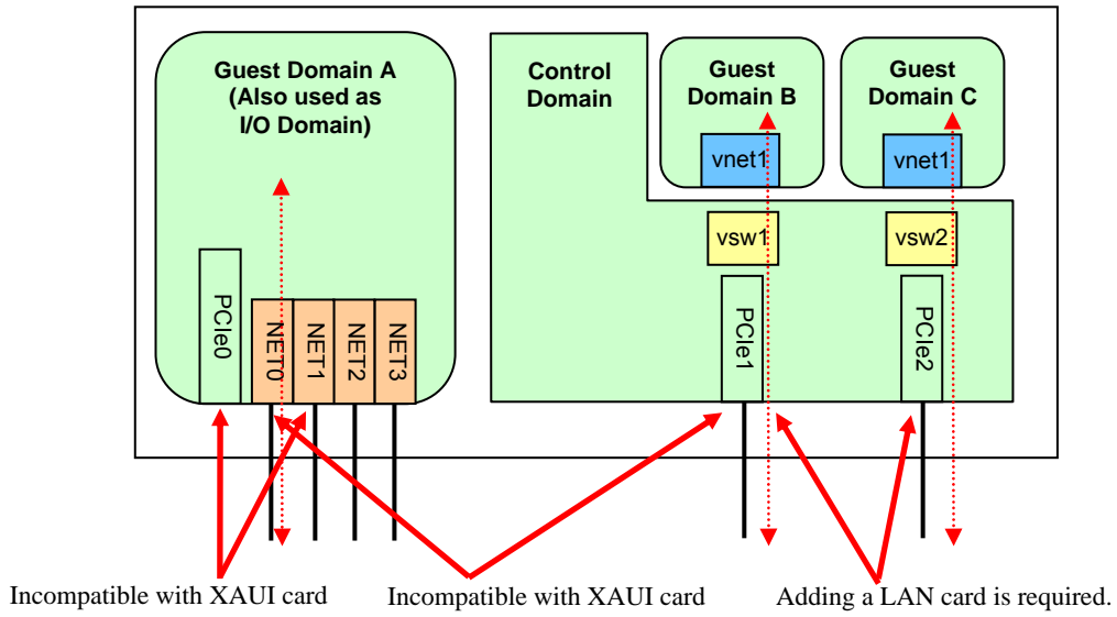
Figure 10.1 In case of SPARC Enterprise T5140
