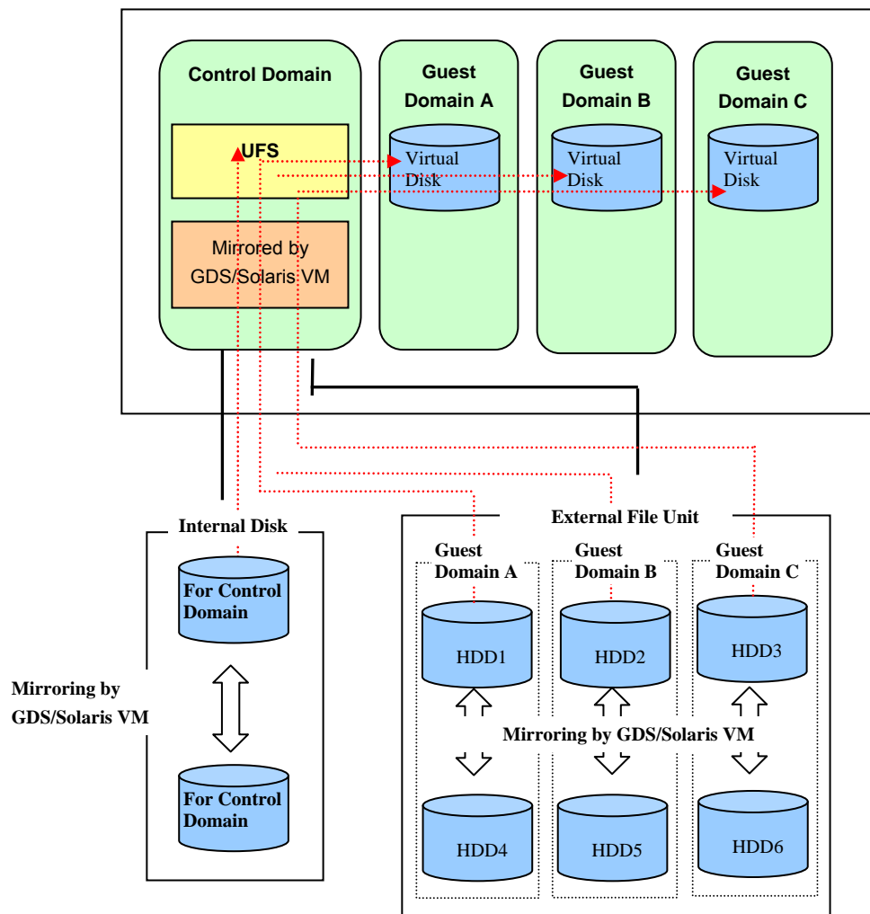
Figure 3.3 Example 1 Configuration when building the LDomS using direct I/O
