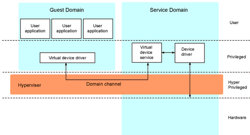
Figure 1.2 Operation modes of Ultra SPARC T2/T2 Plus processors
