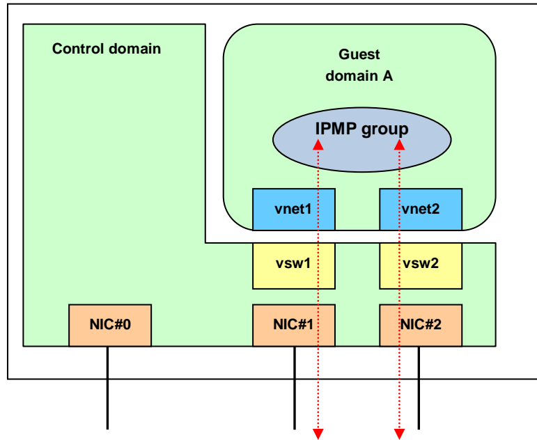
Figure 3.11 Multi-path configuration with Guest Domain
