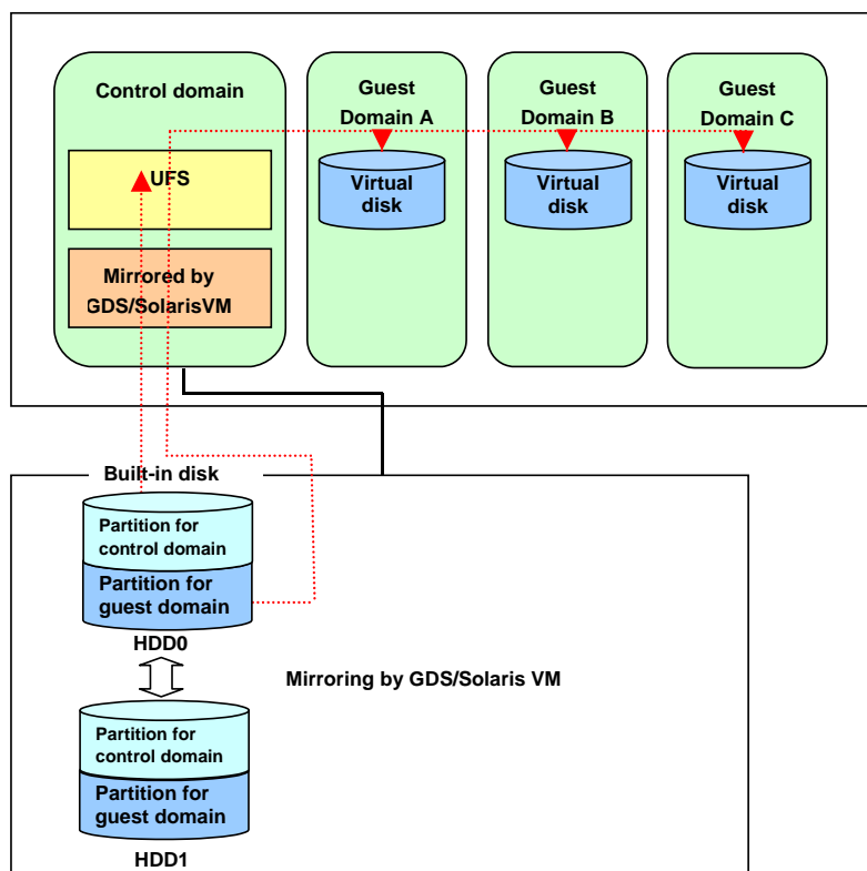
Figure 3.2 Example 2 Configuration when building the LDomS in the internal disk
