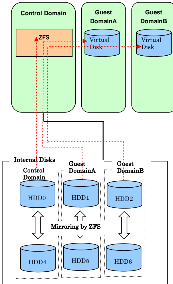
Figure 3.8 Example 3 Configuration when building the LDoms in the internal disk
