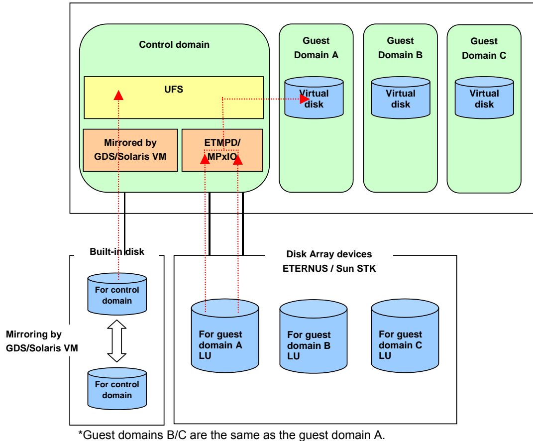
Figure 3.5 Example 3 Configuration when building the LDomS using direct I/O
