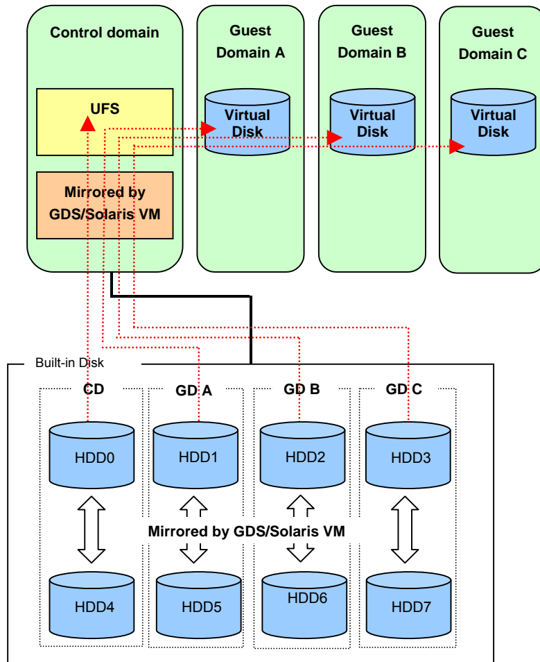
Figure 3.1 Example 1 Configuration when building the LDomS in the internal disk
