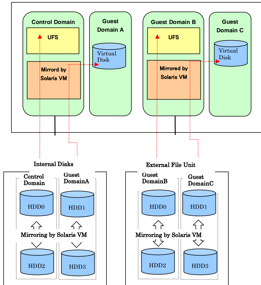
Figure 3.7 Example 5 Configuration when building the LDomS using direct I/O
