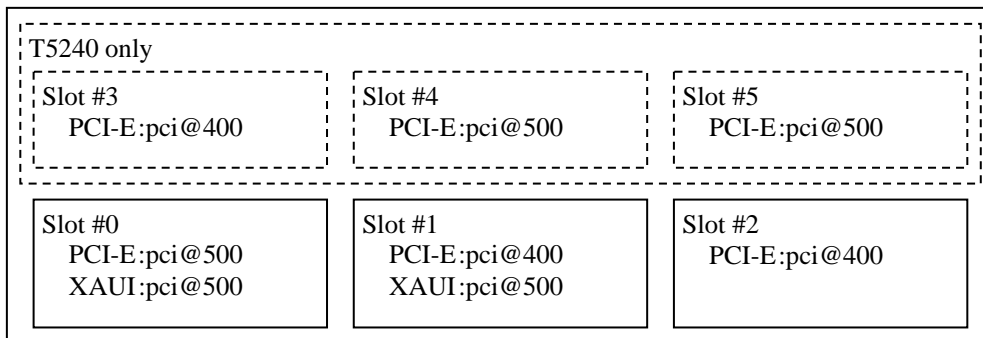
Figure 10.3 Slot location and I/O devices on SPARC Enterprise T5140/T5240
