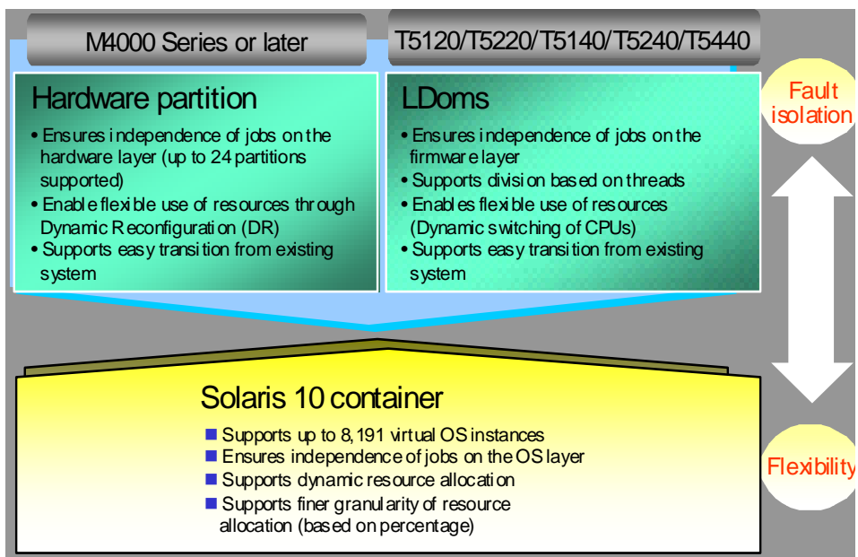
Figure 2.1 Partitioning methods
