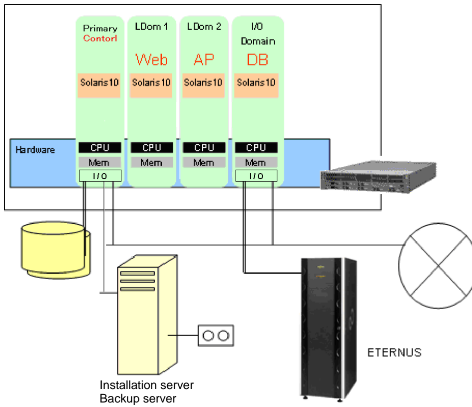
Figure 2.5 Example of configuration for migration from DB servers of previous Solaris servers
