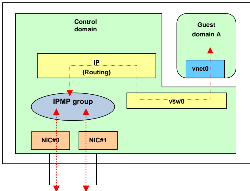
Figure 3.12 Multi-path configuration with Control Domain
