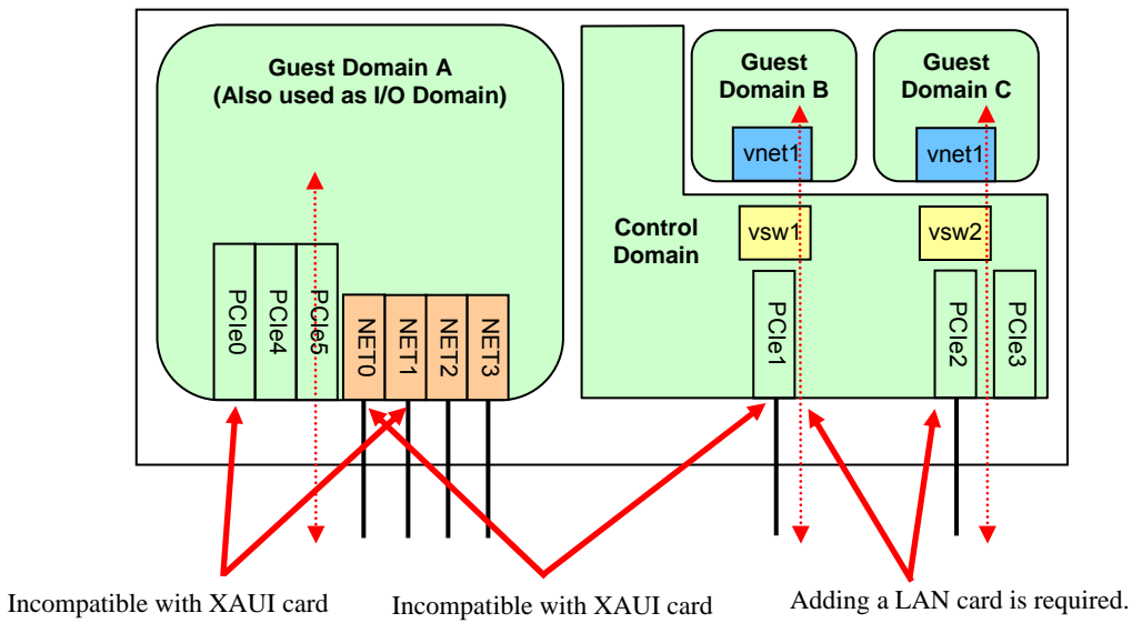
Figure 10.2 In case of SPARC Enterprise T5240
