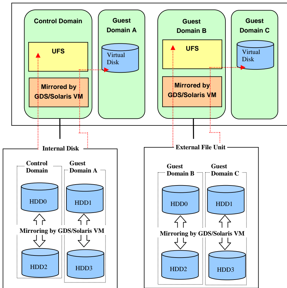
Figure 3.4 Example 2 Configuration when building the LDoms using direct I/O
