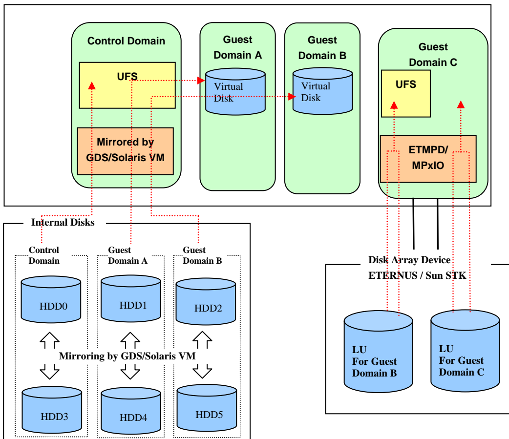
Figure 3.6 Example 4 Configuration when building the LDomS using direct I/O
