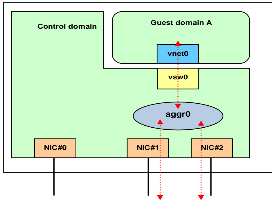
Figure 3.10 Link Aggregation configuration with Control Domain
