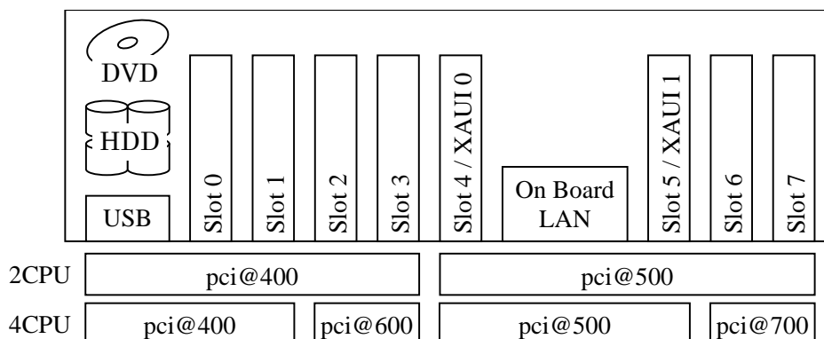
Figure 10.4 Slot location and I/O devices on SPARC Enterprise T5440
