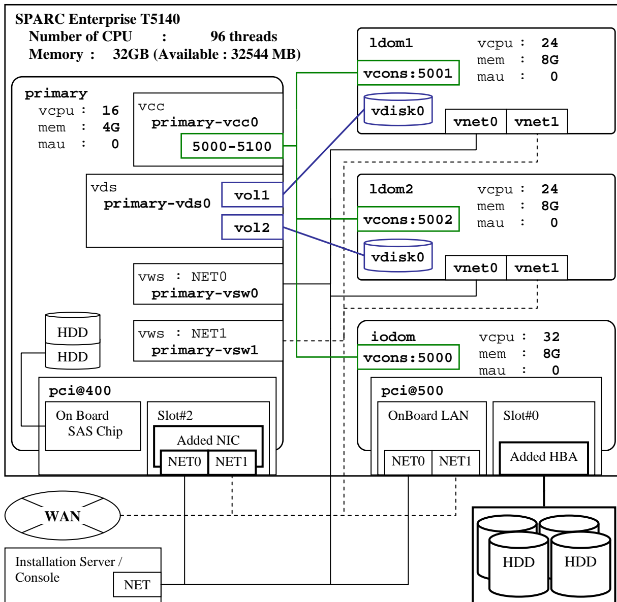
Figure 5.1 Example of configuration on SPARC Enterprise T5140
