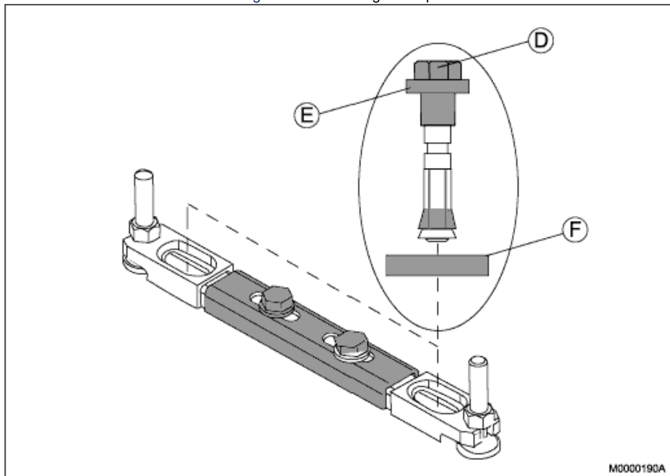
Figure 3.18: Installing the Expander Screw
