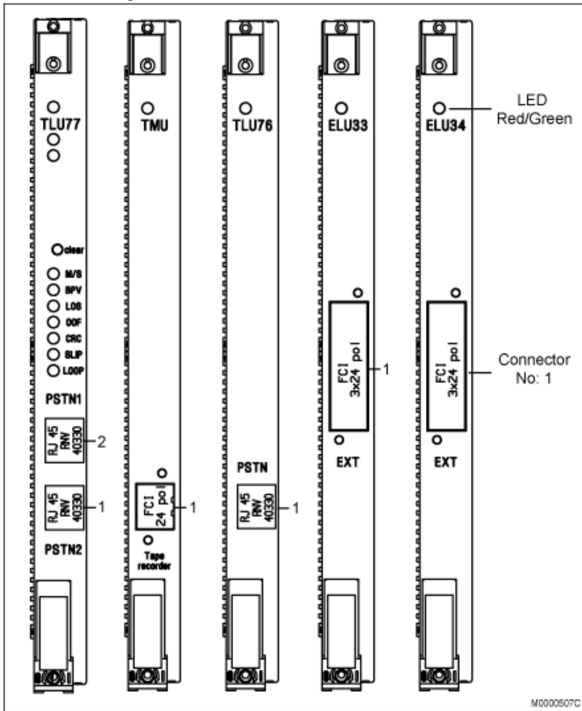
Figure 3.46: TLU77, TMU, TLU76, ELU33, and ELU34 Board Fronts
