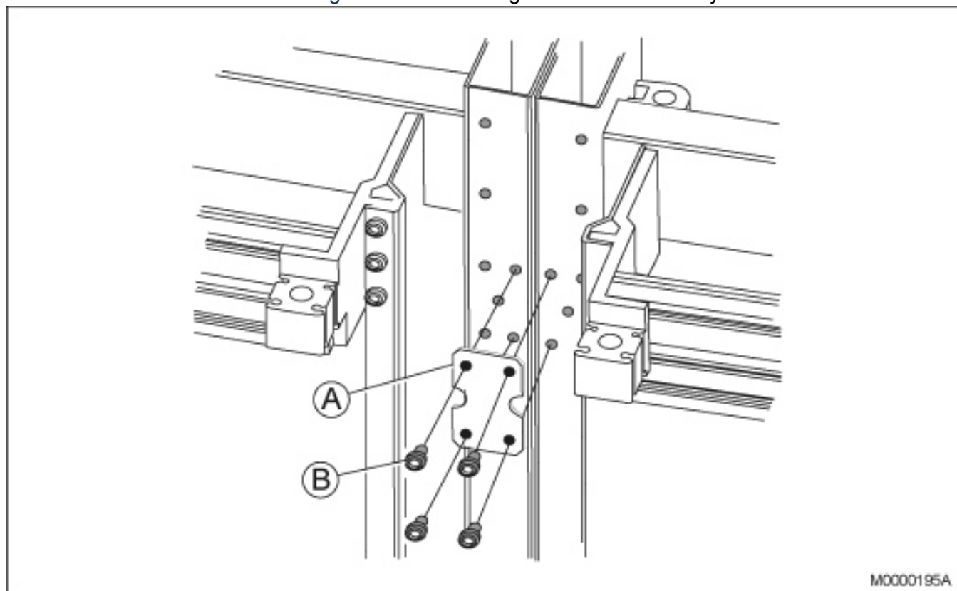
Figure 3.21: Fastening the Cabinets Side-by-Side
