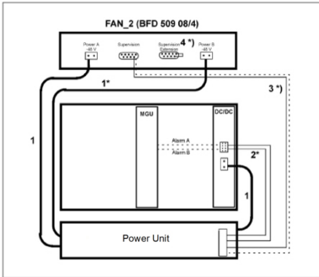
Figure 3.57: Single cables to the Fan Unit BFD50908/4 and to 7U chassis
