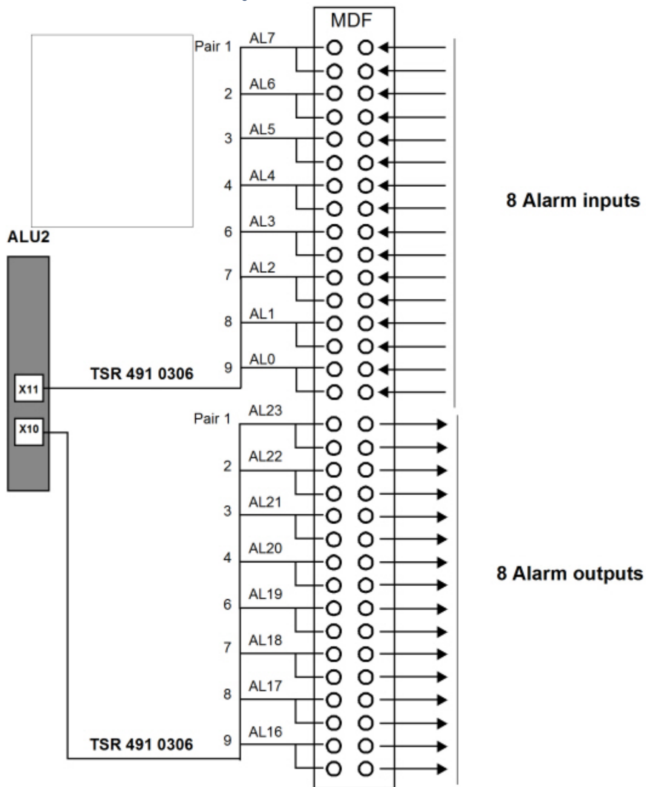
Figure 3.75: ALU2 - MDF connections
