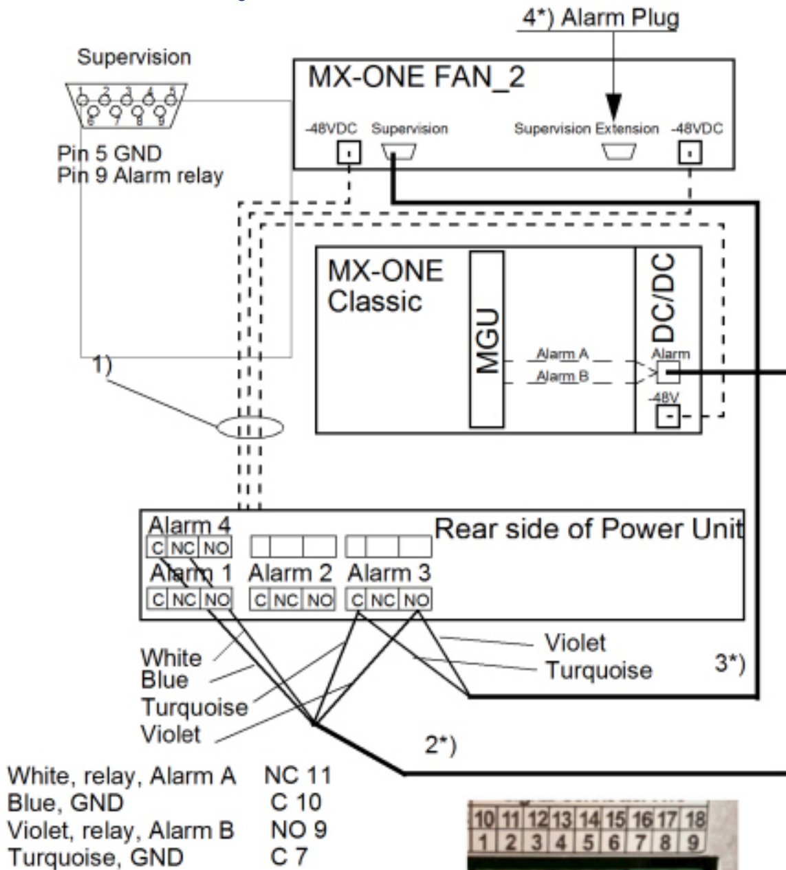
Figure 3.78: Power and Fan alarm in Classic chassis
