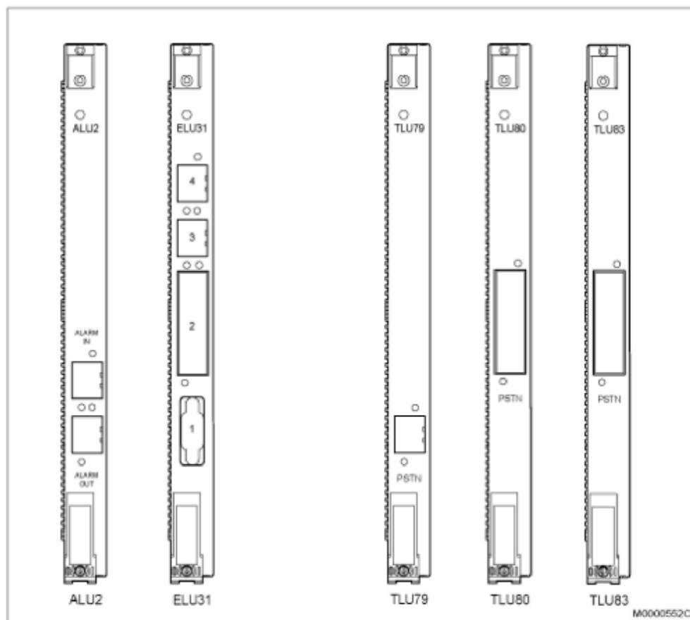
Figure 3.49: ALU2, ELU31, TLU79, TLU80 and TLU83 Fronts
