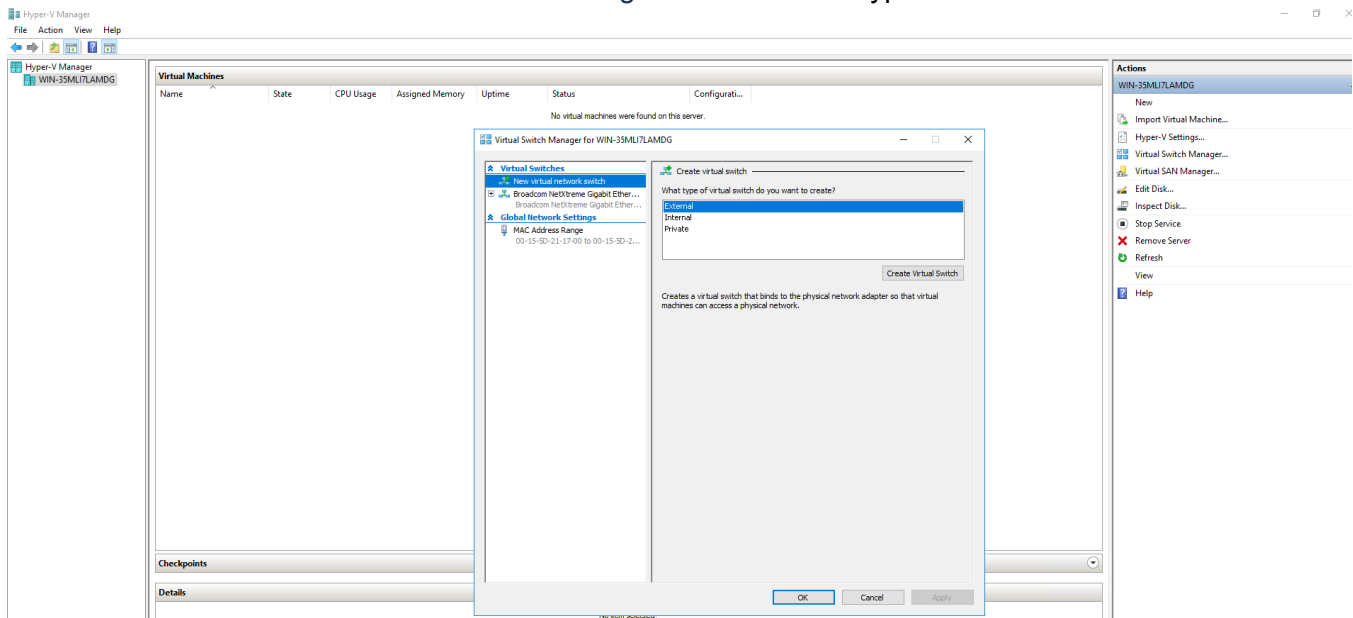
Figure 4.18: Switch Type
