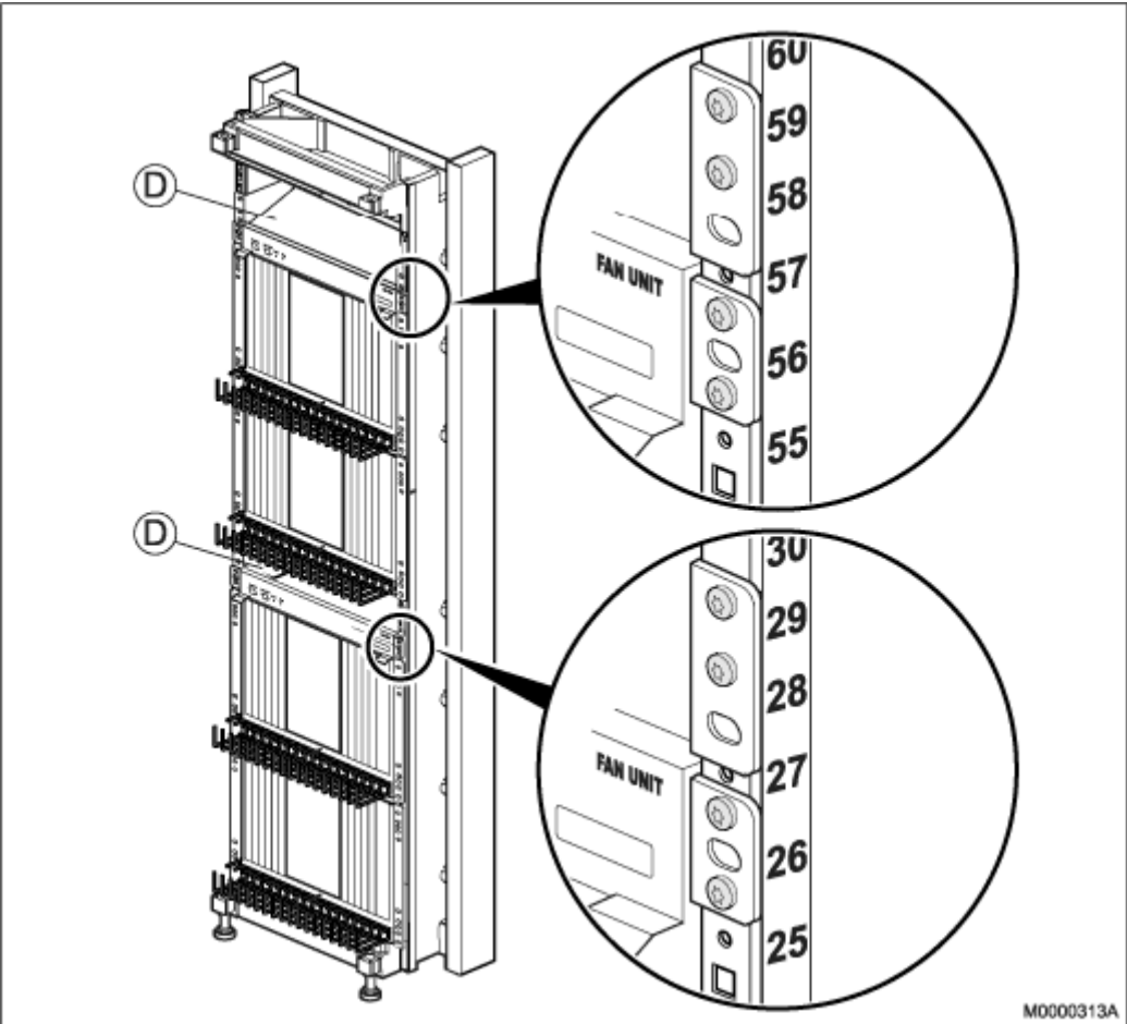
Figure 3.36: A four MX-ONE Classic Rack
