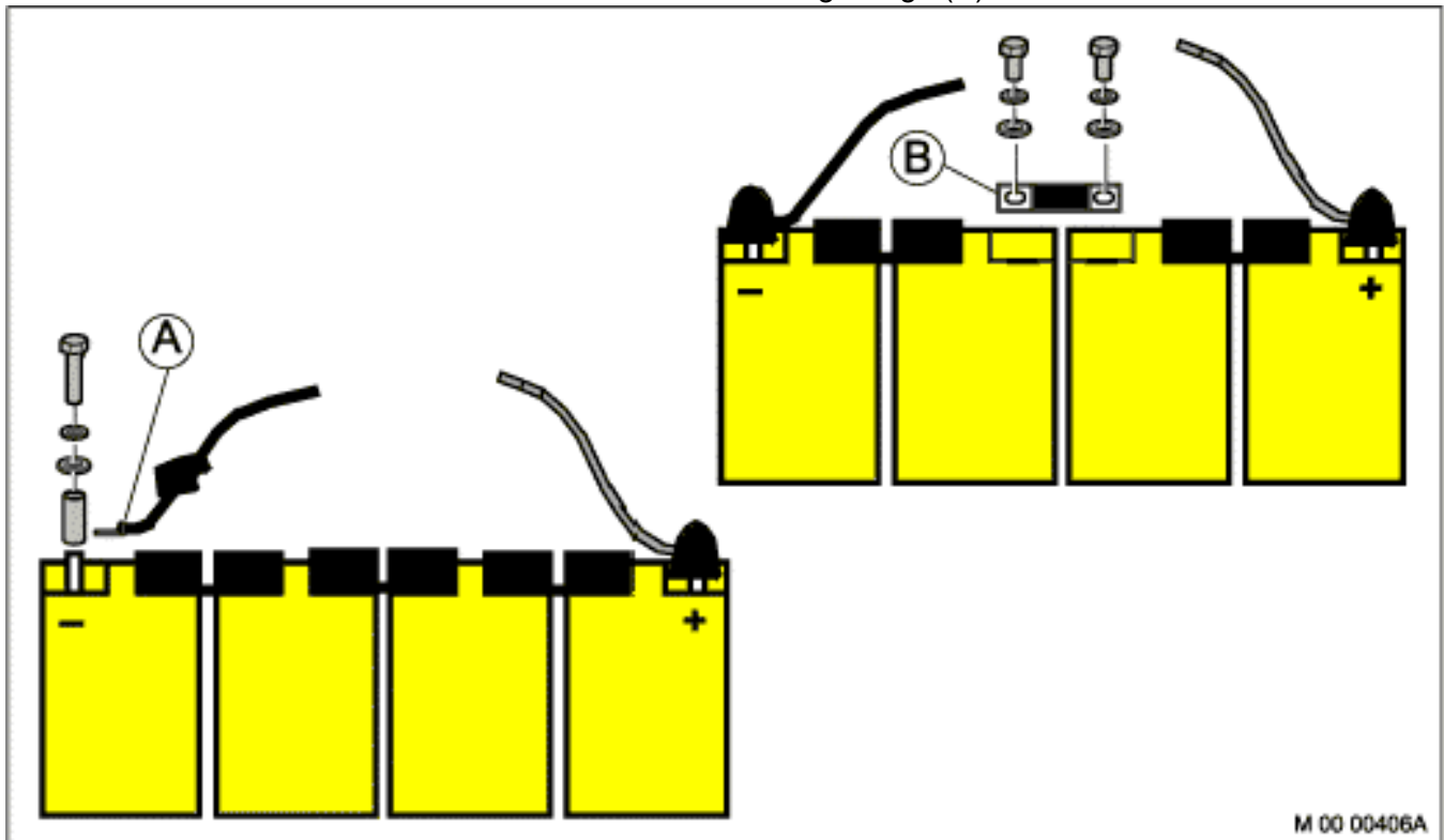
Figure 3.56: Connecting the Batteries
