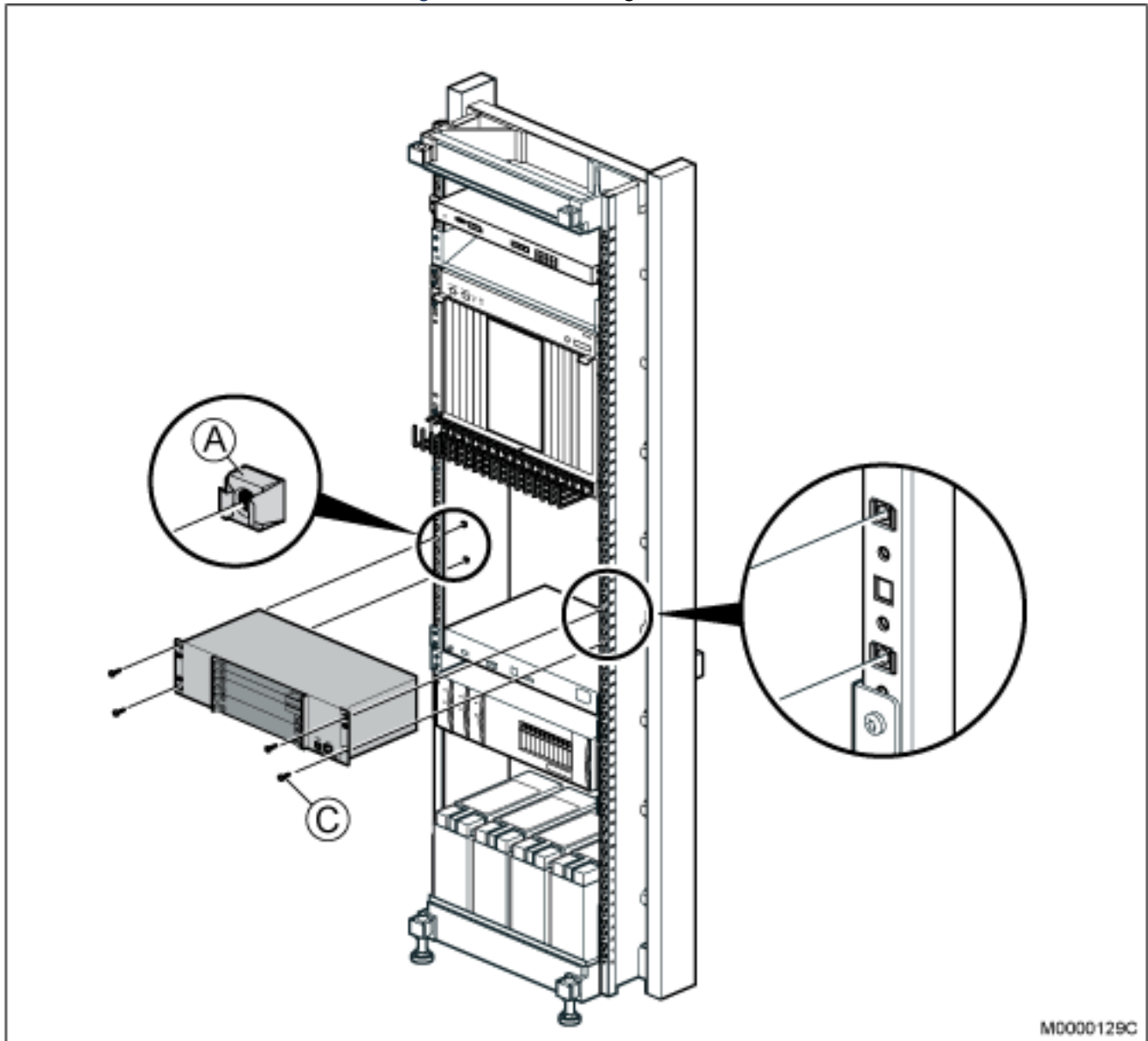
Figure 3.41: Installing MX-ONE Lite subrack
