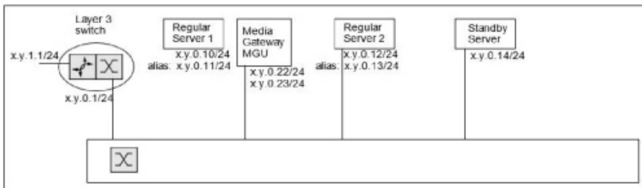
Figure 1.29: Server redundancy without network redundancy
