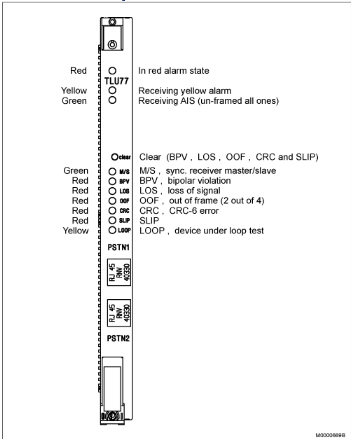
Figure 3.50: TLU77 Front Connectors and LEDs
