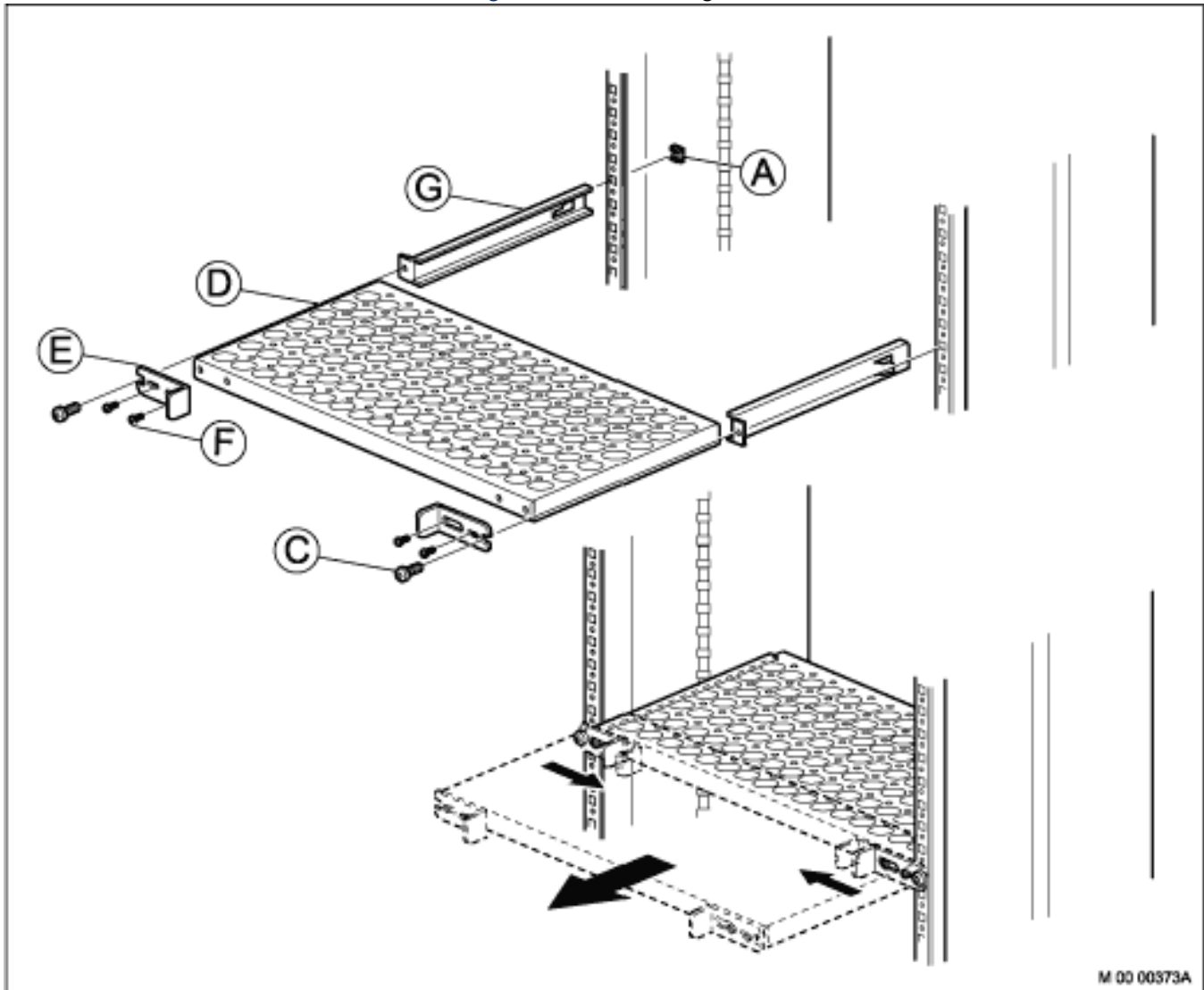
Figure 3.42: Installing Cabinet Shelf
