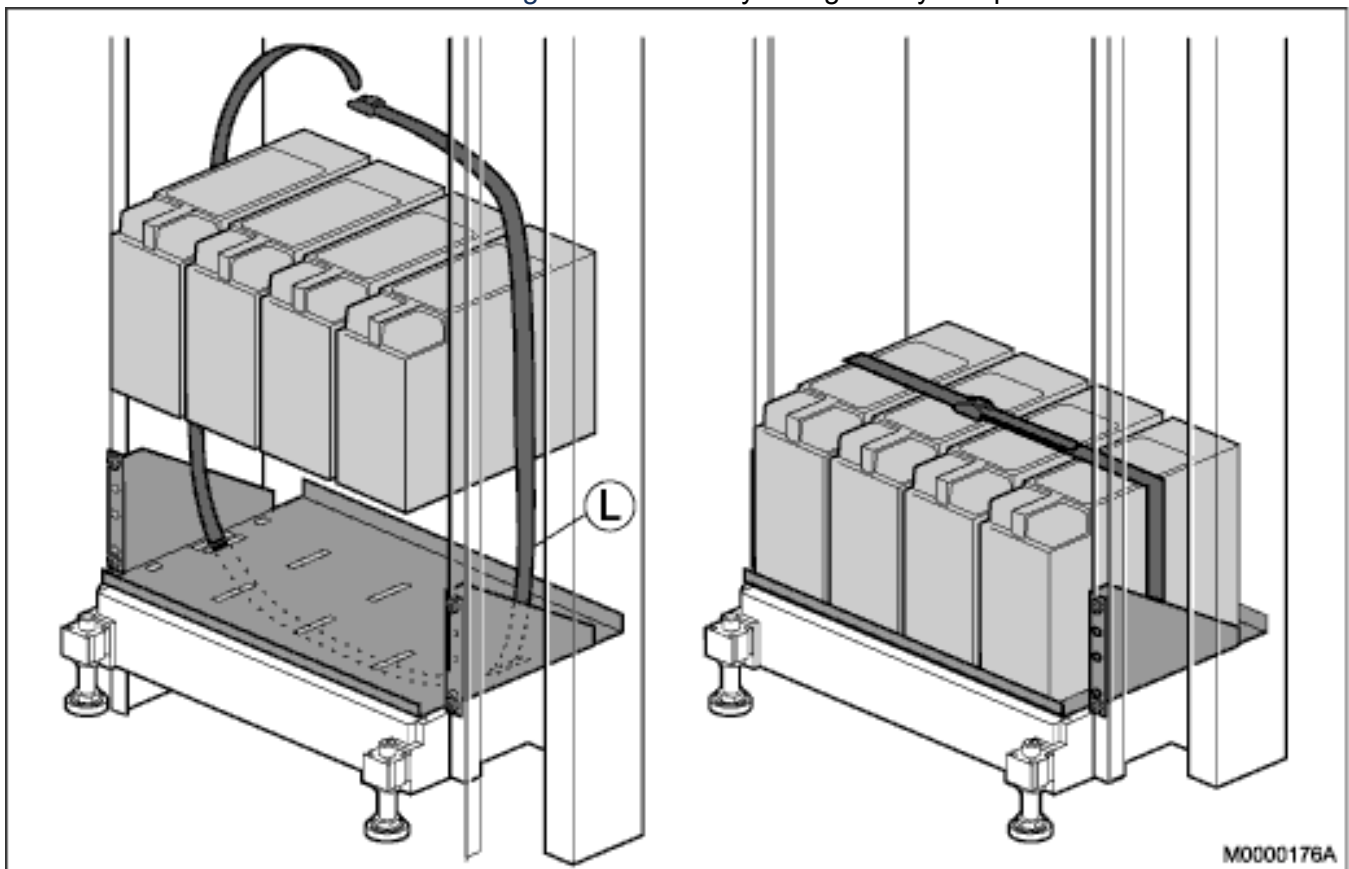
Figure 3.26: Battery String Safety Strap
