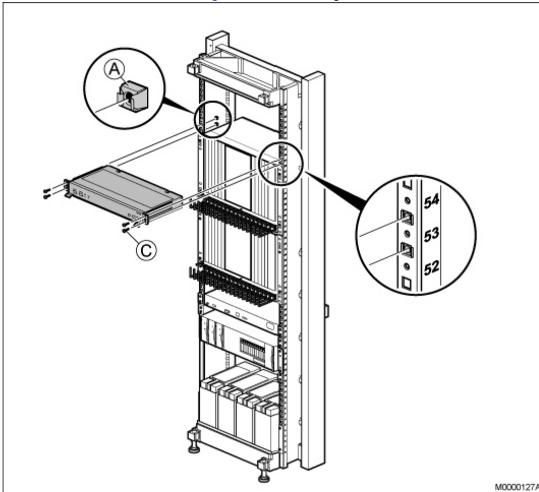
Figure 3.38: Installing the Fan Unit
