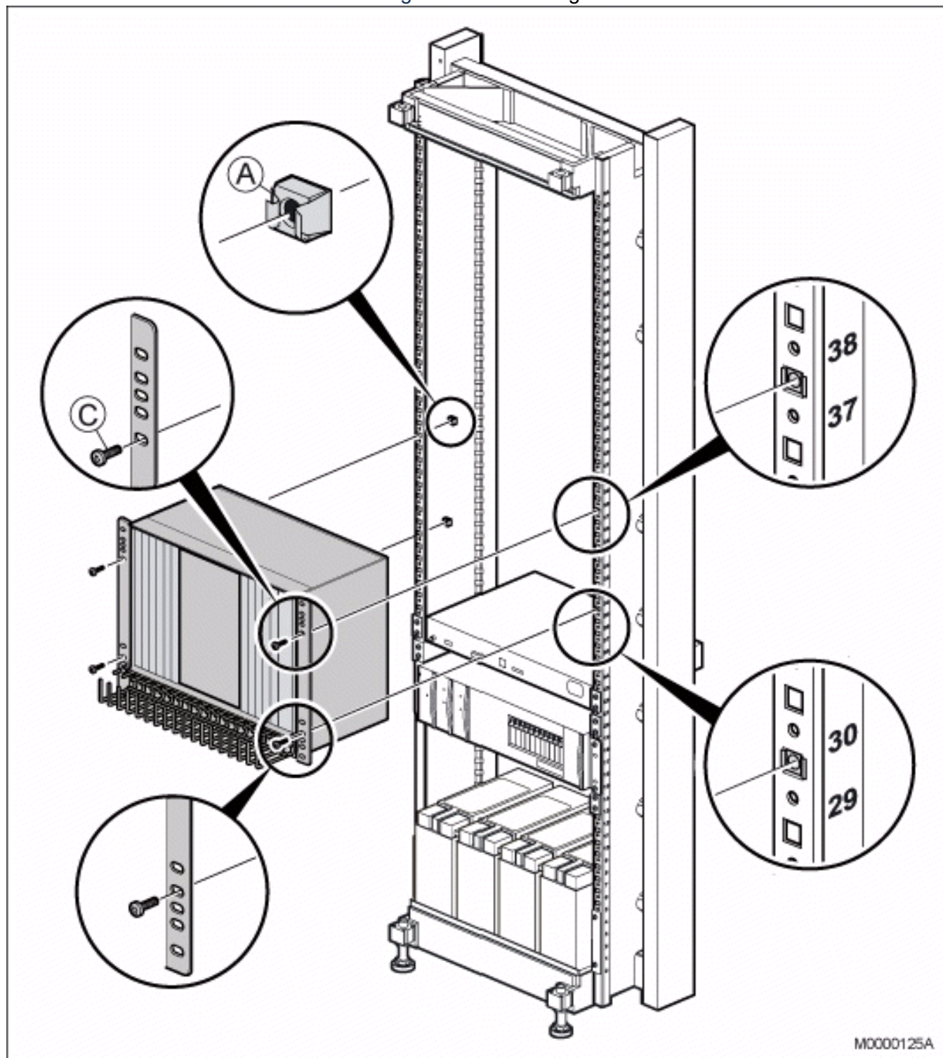
Figure 3.31: Installing Subrack B
