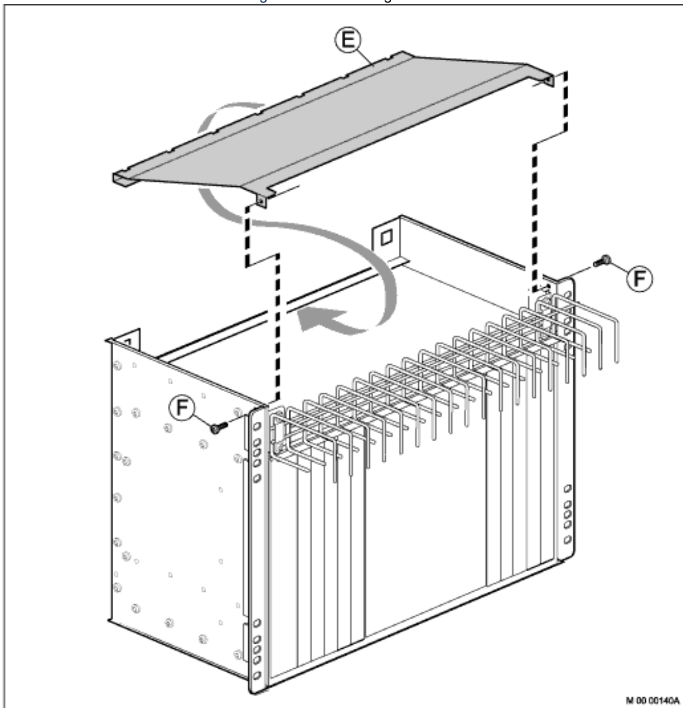
Figure 3.30: Mounting the Lower Air Plate
