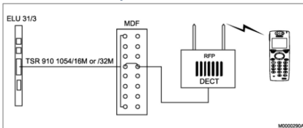
Figure 3.67: ELU31/4 MDF - RFP
