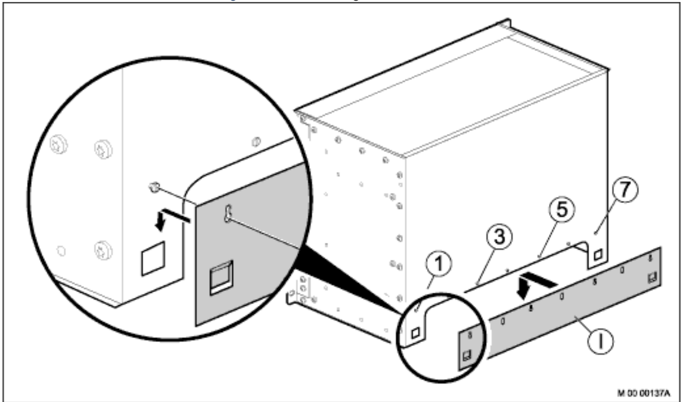
Figure 3.33: Mounting Rear Air Plate in Subrack A
