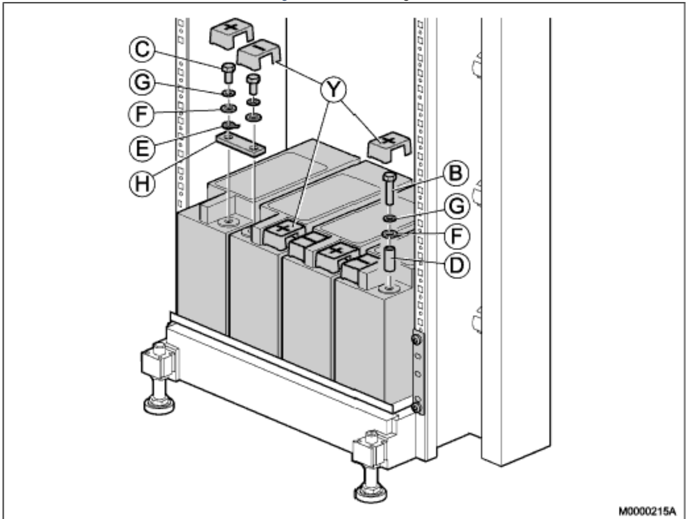
Figure 3.25: Installing the Batteries
