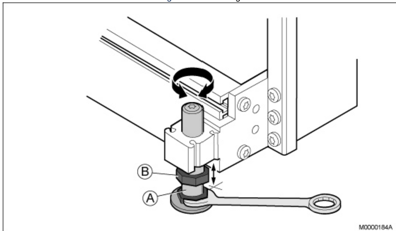
Figure 3.13: Leveling the Cabinet
