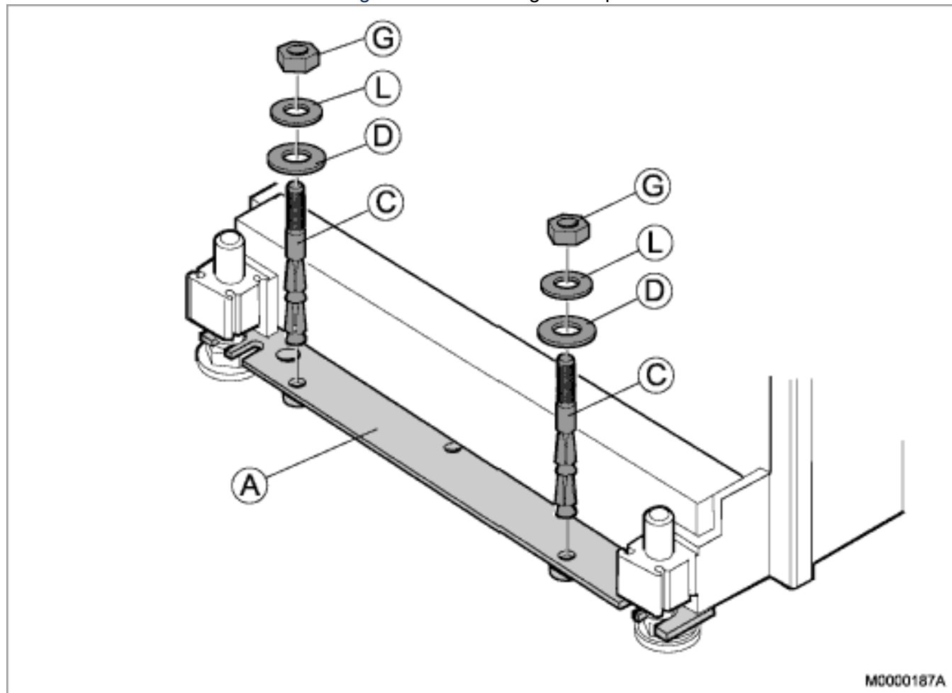
Figure 3.15: Installing the Expander Screw
