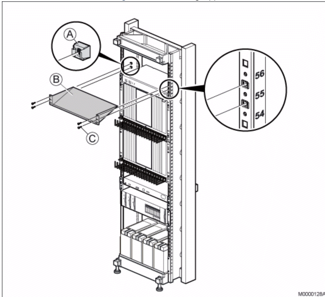
Figure 3.35: Installing Upper Air Plate
