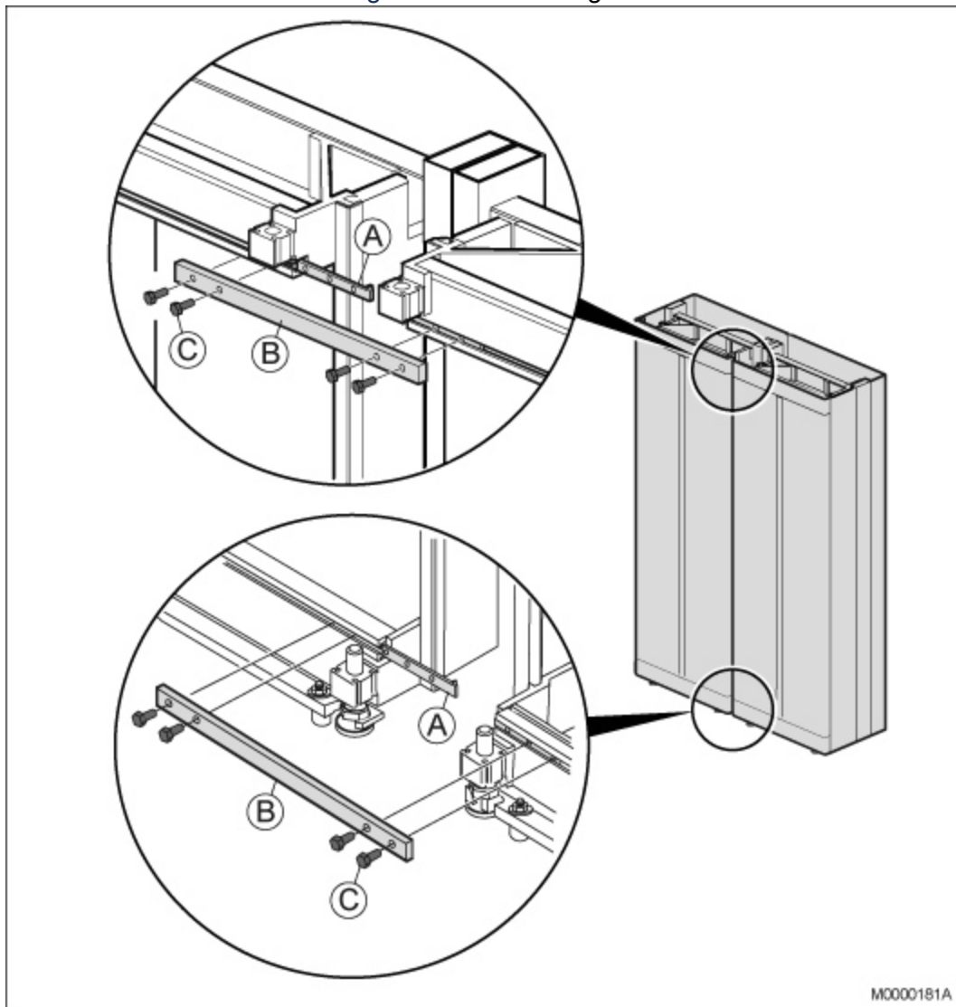
Figure 3.11: Mounting the Earth Bar
