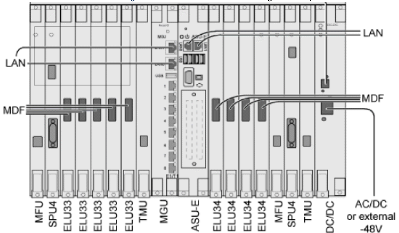
Figure 3.59: Cable Connections Configure Example
