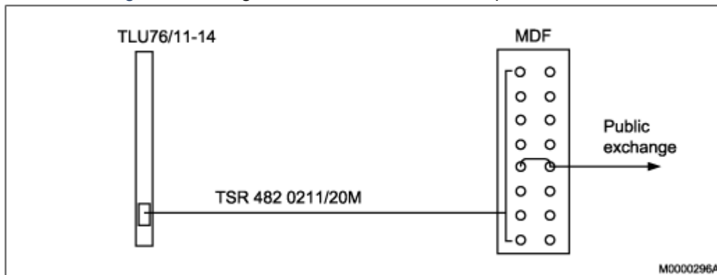
Figure 3.71: Digital external lines 120 ohm pair cable, TLU76/11 - /14
