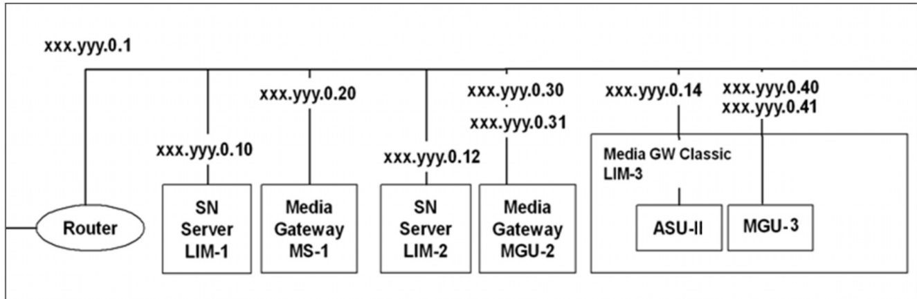
A non-redundant scenario with MGU and MS media gateways
