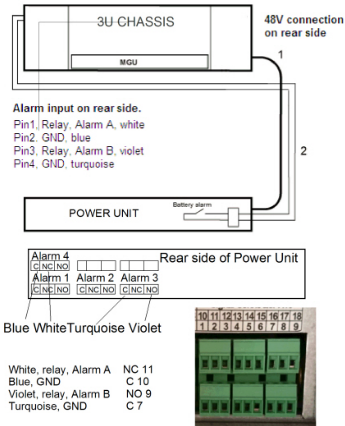
Figure 3.77: MGU Power Alarm Detection in MX-ONE Lite
