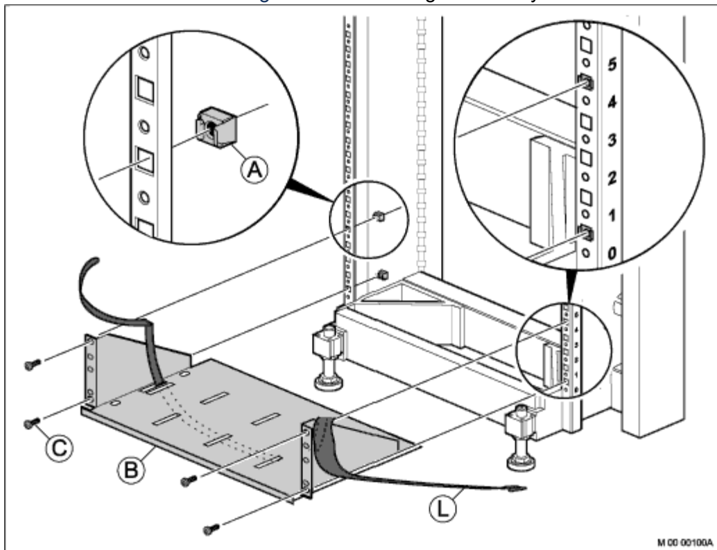
Figure 3.23: Installing the Battery Shelf
