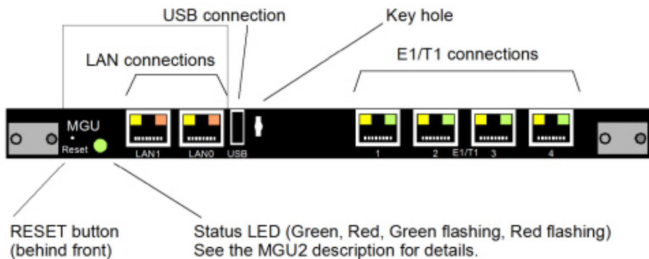
Figure 3.51: MGU2 with 20mm front
