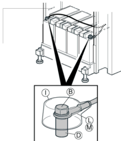
Figure 3.56: Connecting the Batteries
