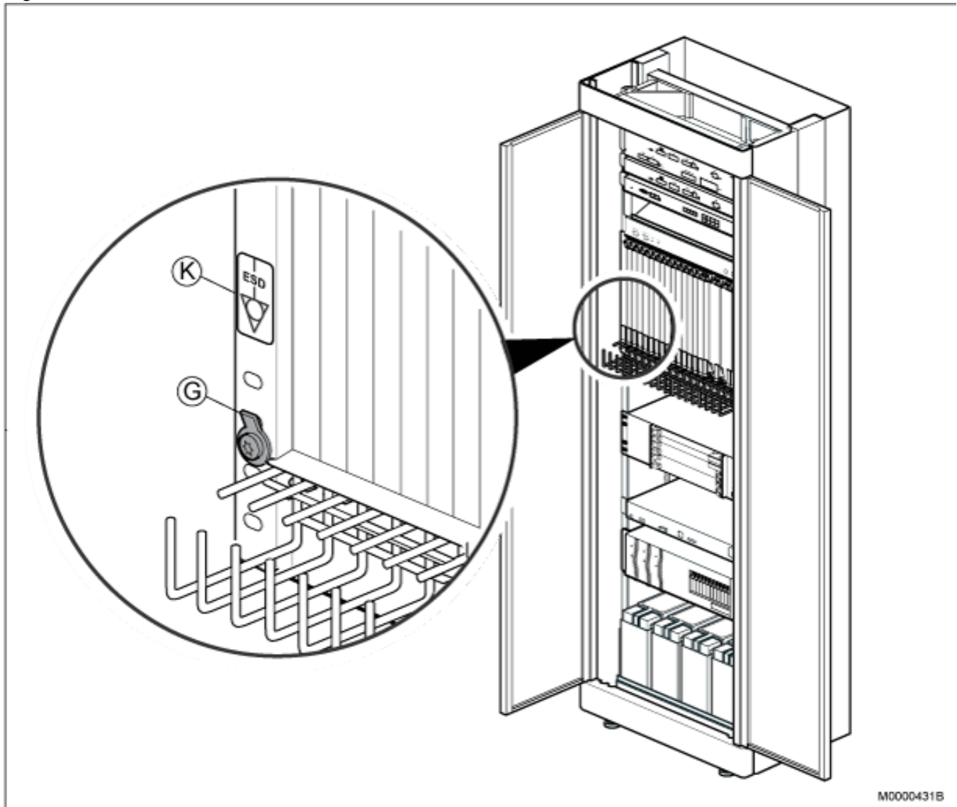
Figure 1: ESD-earth Points in BYB 501
