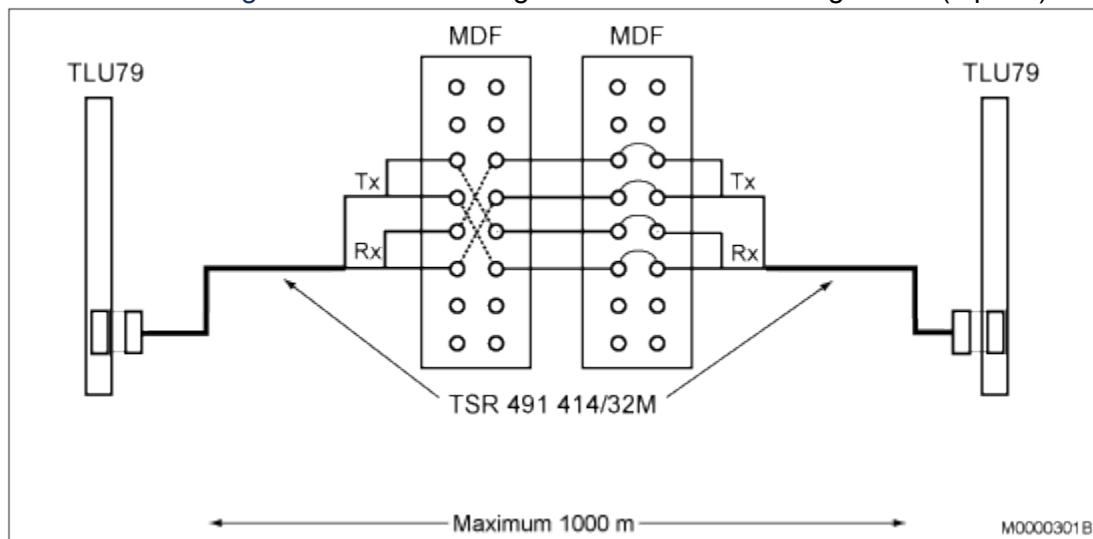
Figure 3.73: Connecting TLU79 to TLU79 through MDF (8 pairs)
