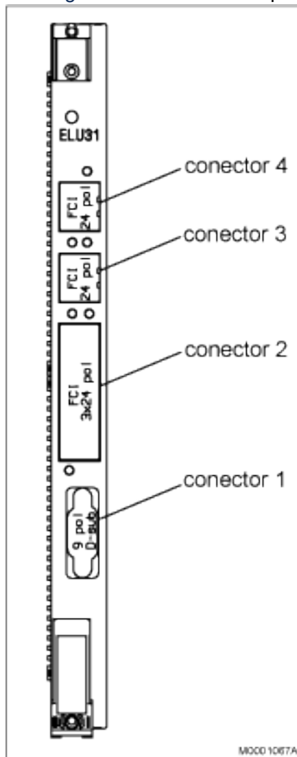
Figure 3.52: Connectors positioning
