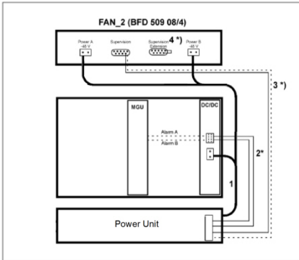
Figure 3.58: Splitter Cable to the Fan Unit BFD50908/4 and to 7U chassis
