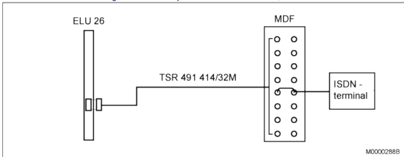
Figure 3.66: Example with an ISDN-terminal, 4-wire connection
