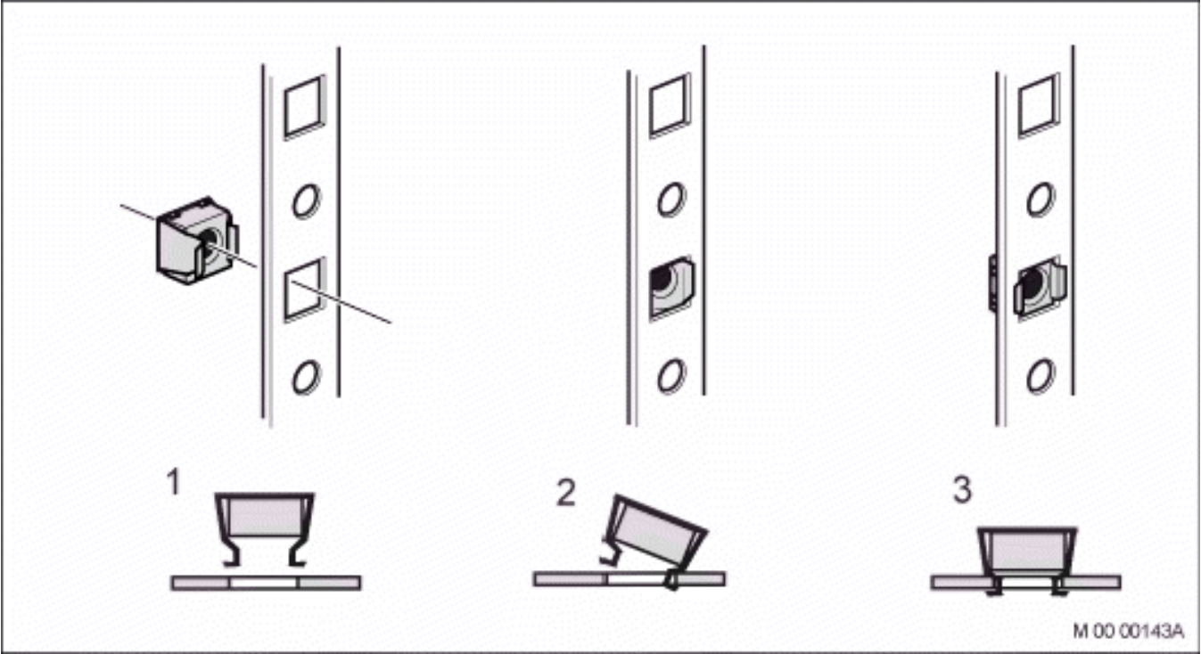
Figure 3.22: Mounting the Captive Nuts in the Rack
