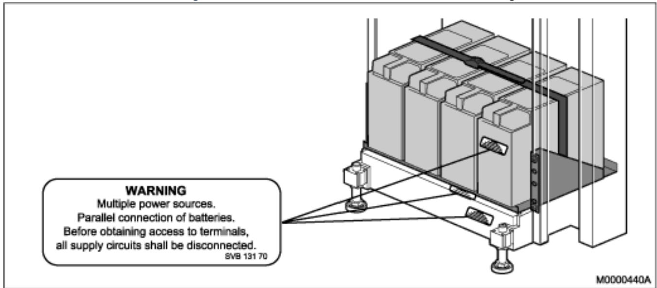
Figure 3.27: Parallel Connection of Batteries Warning Label
