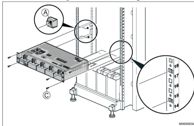
Figure 3.28: Installing AC/DC Unit
