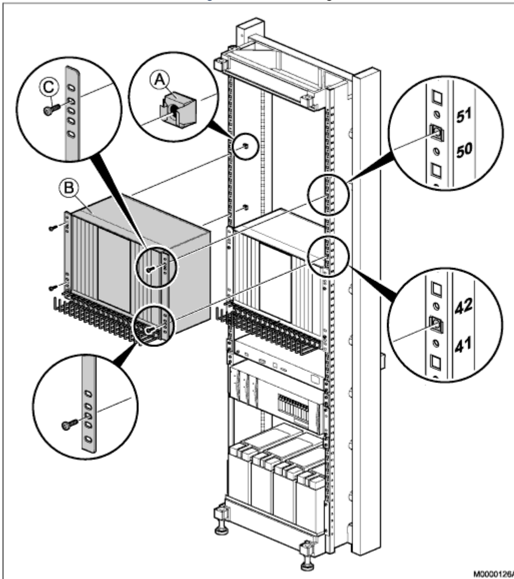
Figure 3.34: Installing Subrack A
