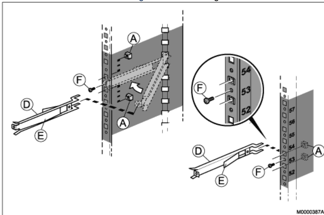
Figure 3.37: Installing Slides
