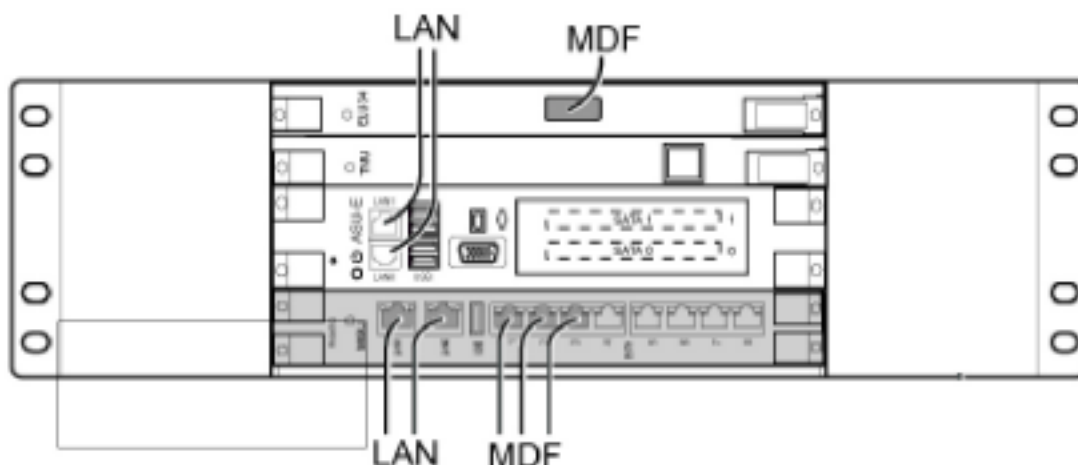
Figure 3.60: MX-ONE Lite cabling example
