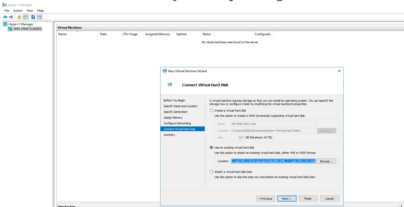
Figure 4.25: Image Selection_1
