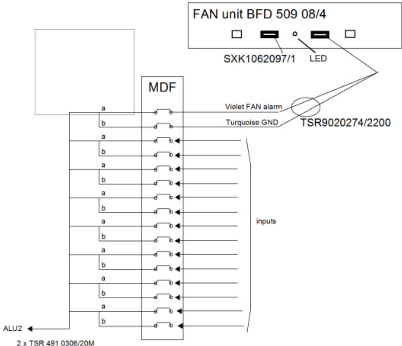
Figure 3.76: MDF Alarms for the Fan Unit BFD 509 08/4
