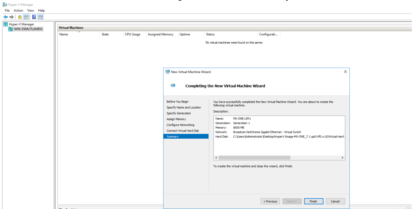
Figure 4.27: Review Summary
