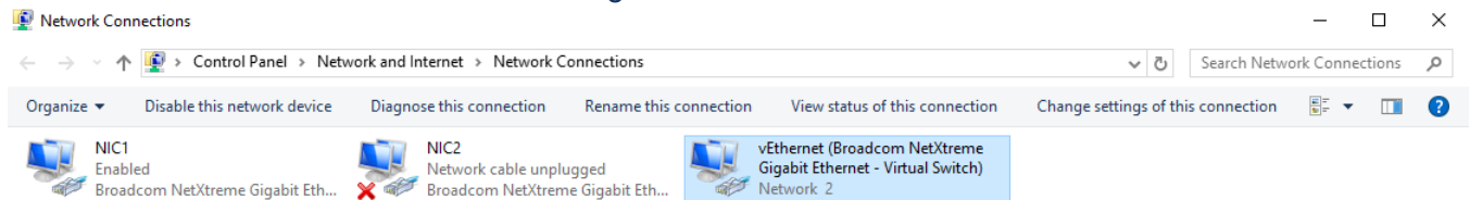
Figure 4.20: Network Connections
