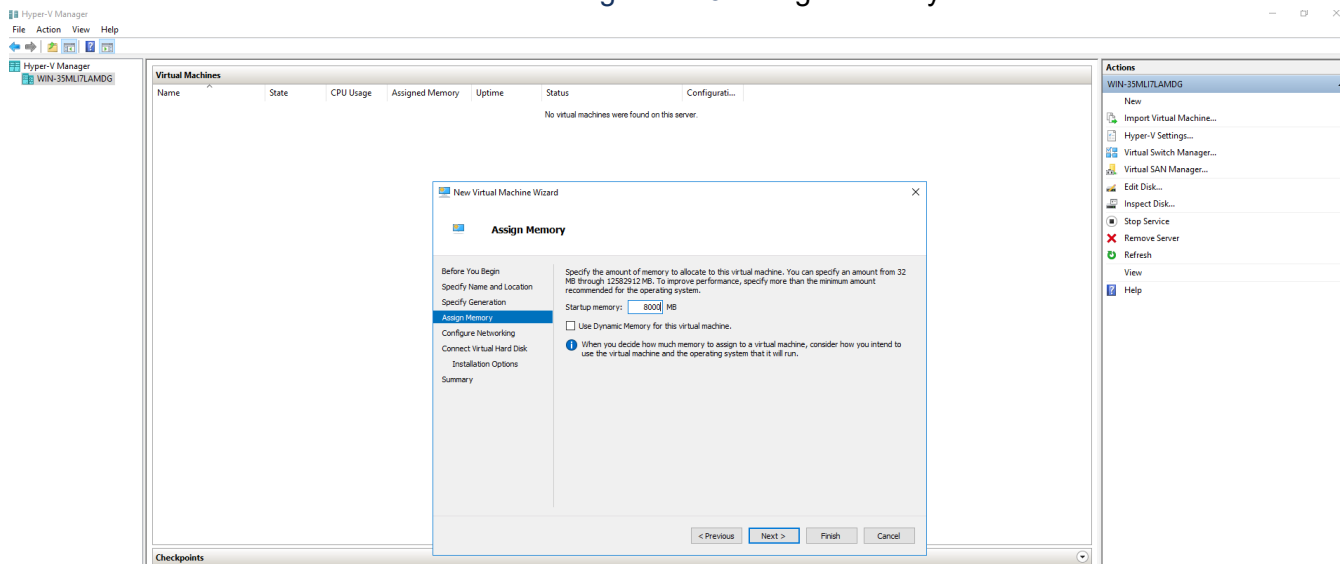
Figure 4.23: Assign Memory
