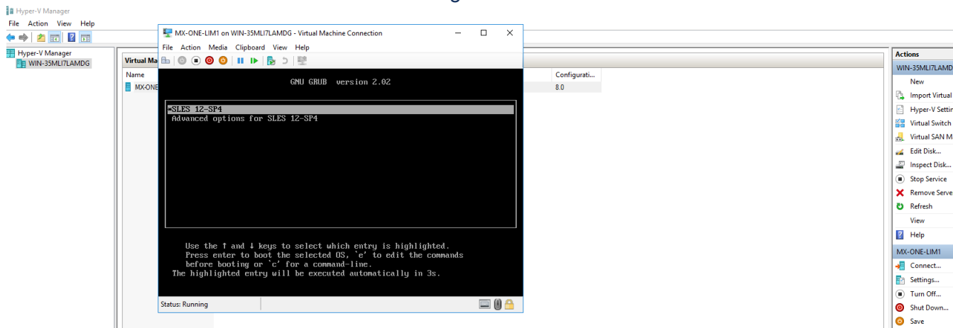
Figure 4.29: Select VM
