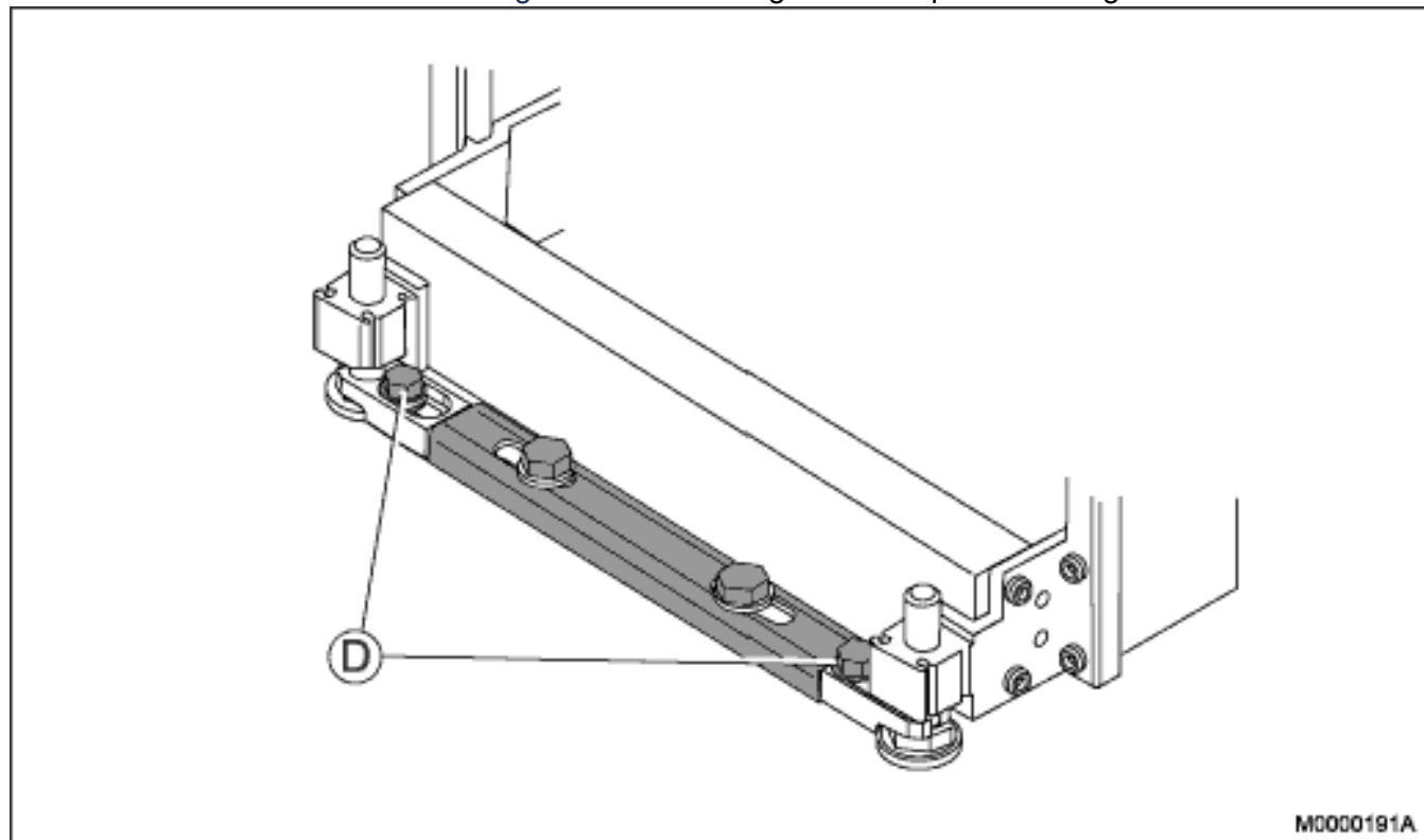
Figure 3.19: Securing the Earthquake Bracing
