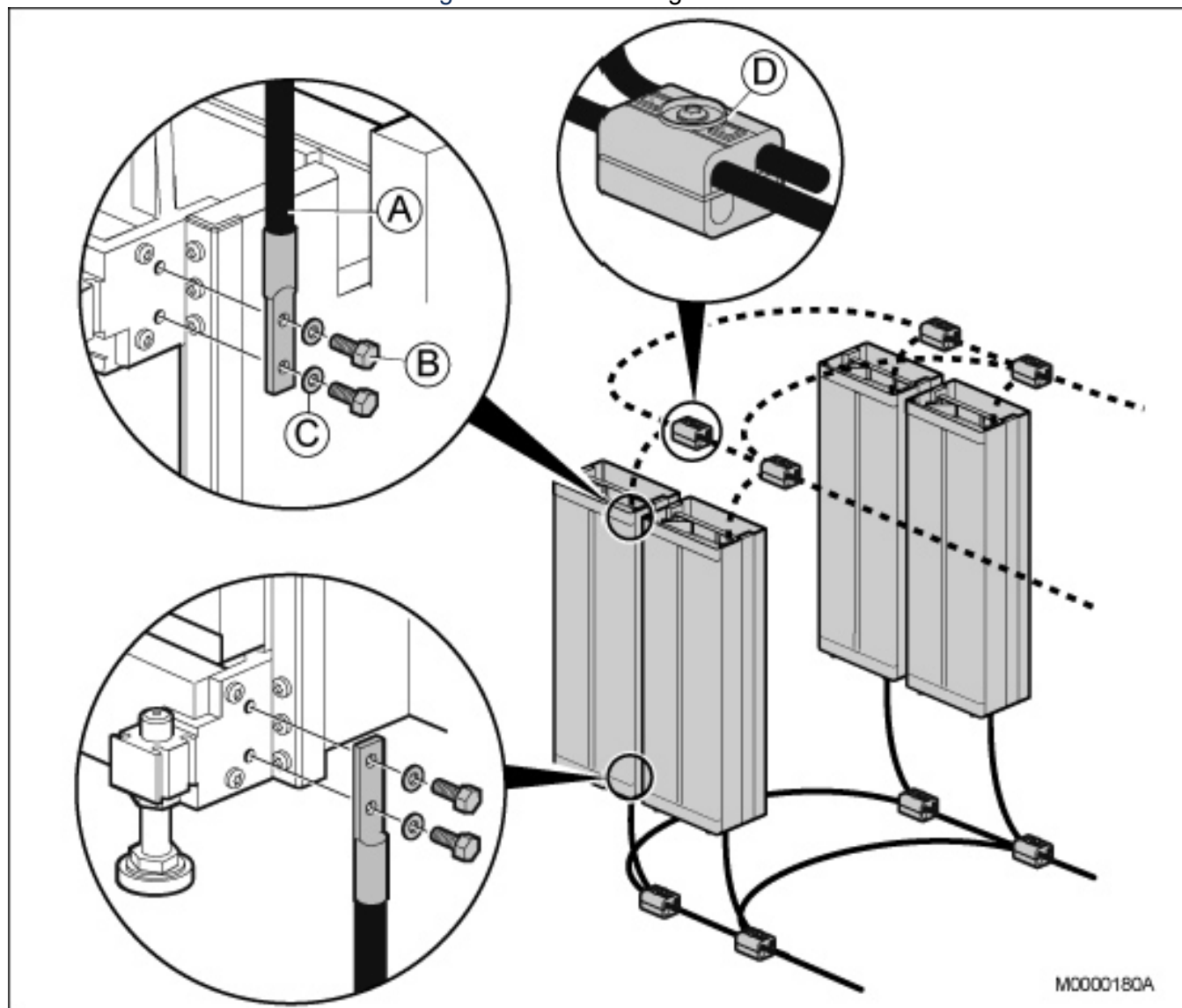
Figure 3.10: Grounding of BYB 501 Cabinet
