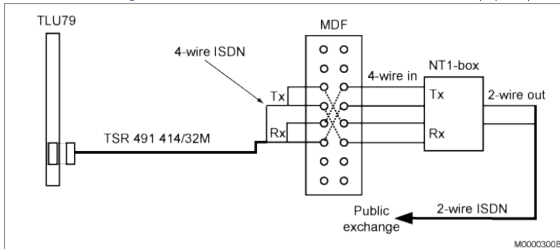
Figure 3.72: 2-wire ISDN with TLU79 and an NT1-box (8 pairs)
