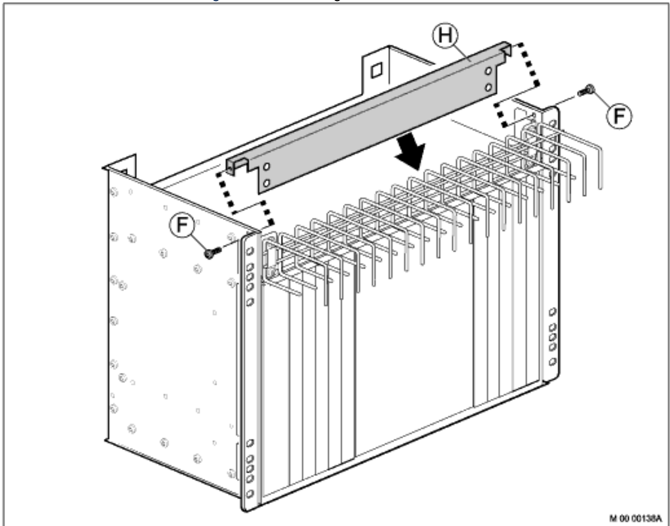
Figure 3.32: Mounting the Front Air Plate in Subrack A
