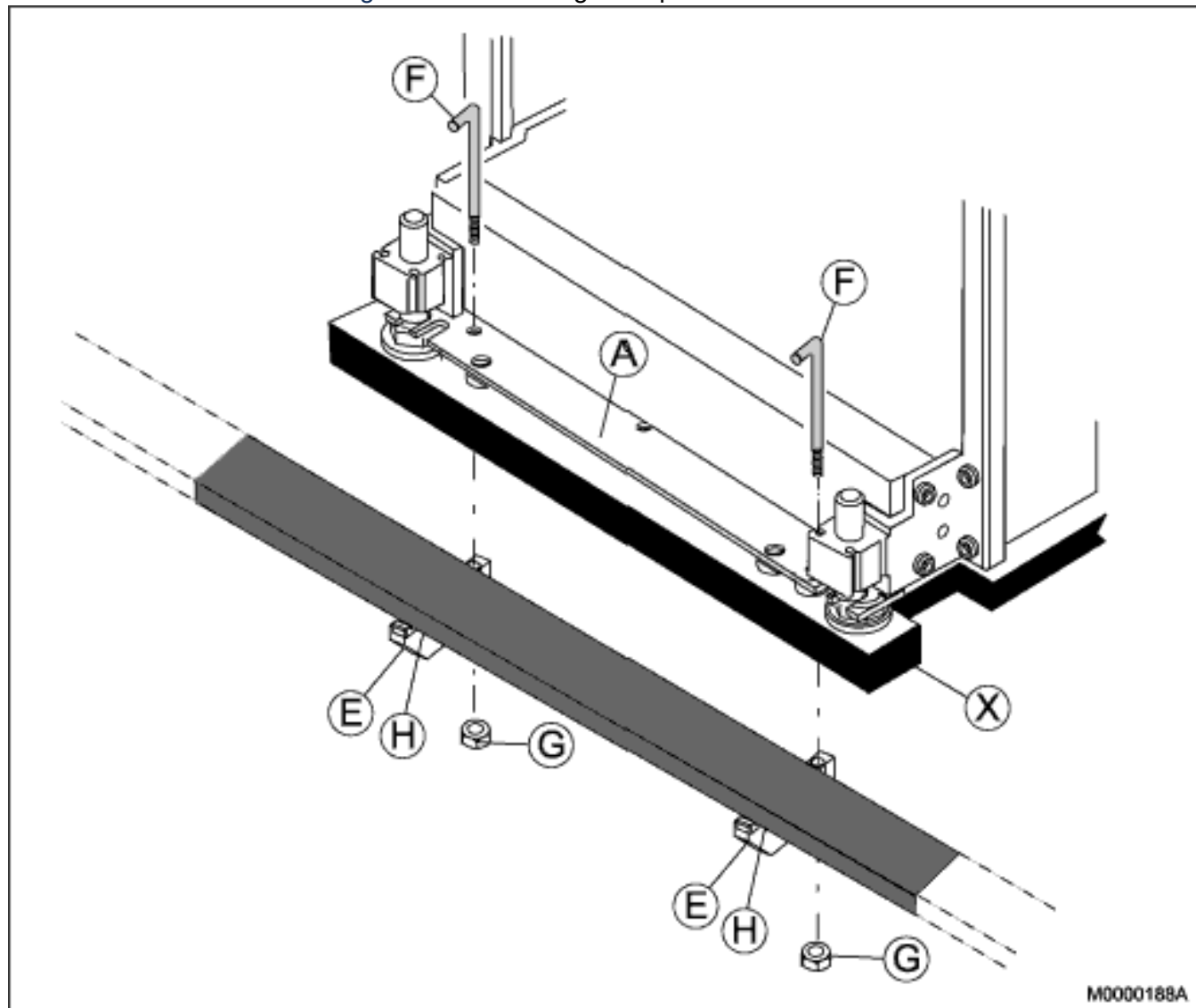
Figure 3.16: Installing the Tip Protection on a Raised Floor
