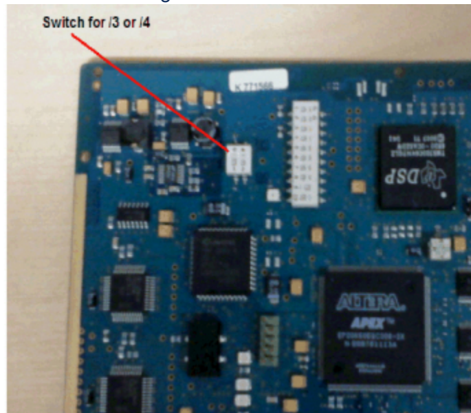
Figure 3.68: ELU31/4 - location of switch
