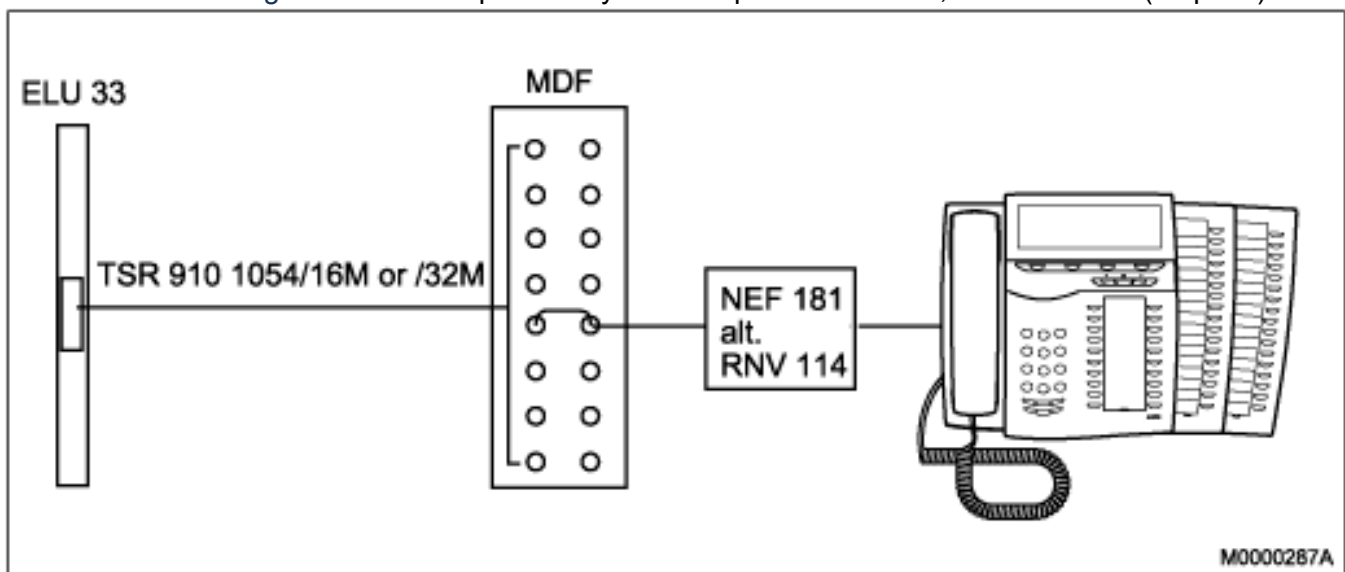
Figure 3.65: Example with system telephone DBC 2xx, ELU33 - MDF (32 pairs)
