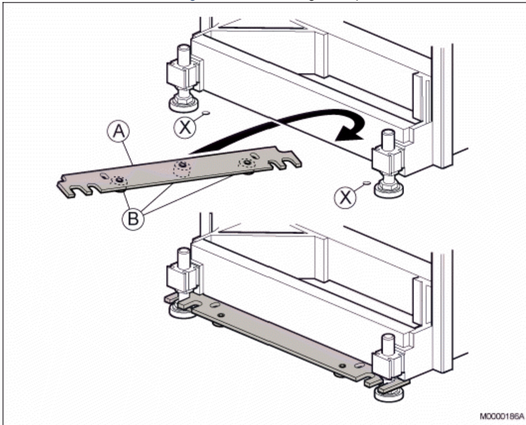
Figure 3.14: Installing the Tip Protection
