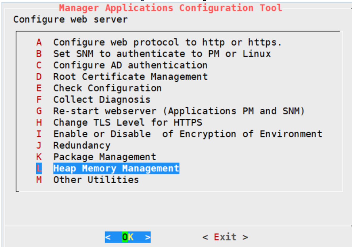
Figure 1.23: Configure Web Server
