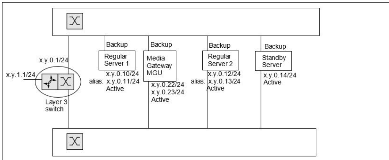
Figure 1.1: Server redundancy with Ethernet bonded network redundancy. System database is not shown here.
