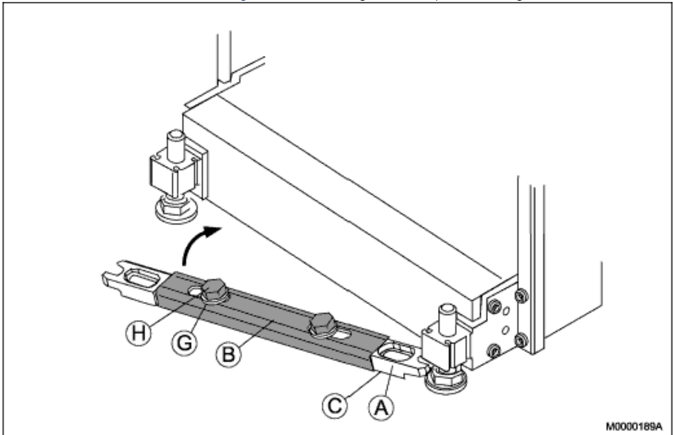
Figure 3.17: Installing the Earthquake Bracing
