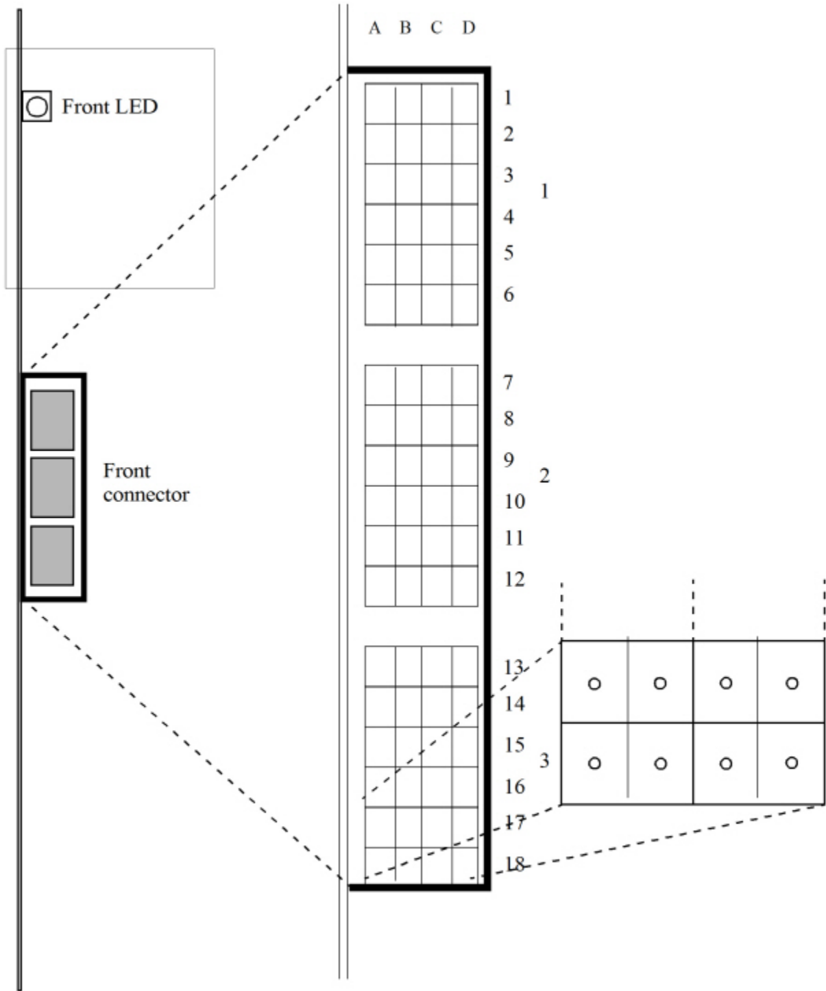
Figure 3.63: Front view
