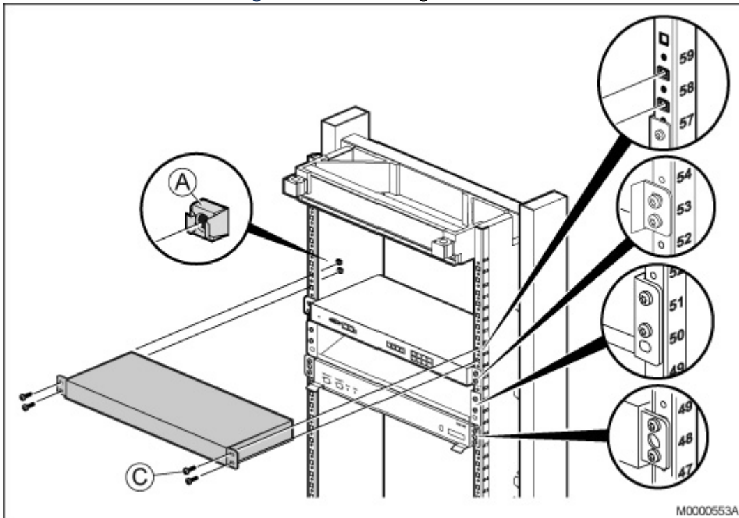
Figure 3.39: Installing MX-ONE 1U chassis
