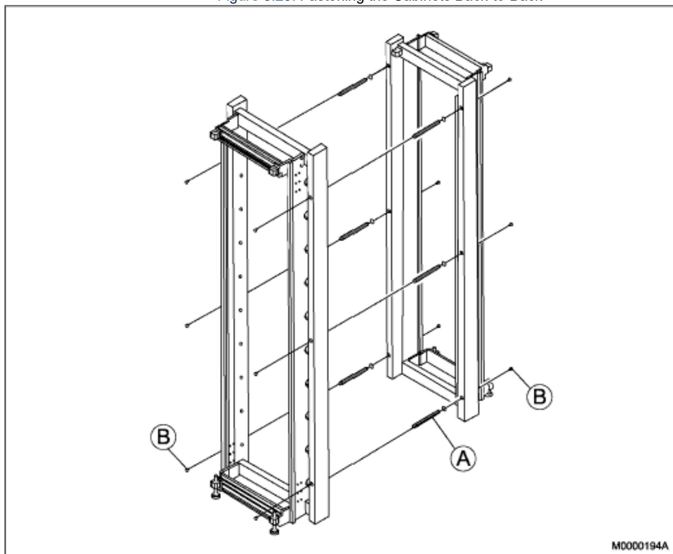
Figure 3.20: Fastening the Cabinets Back-to-Back
